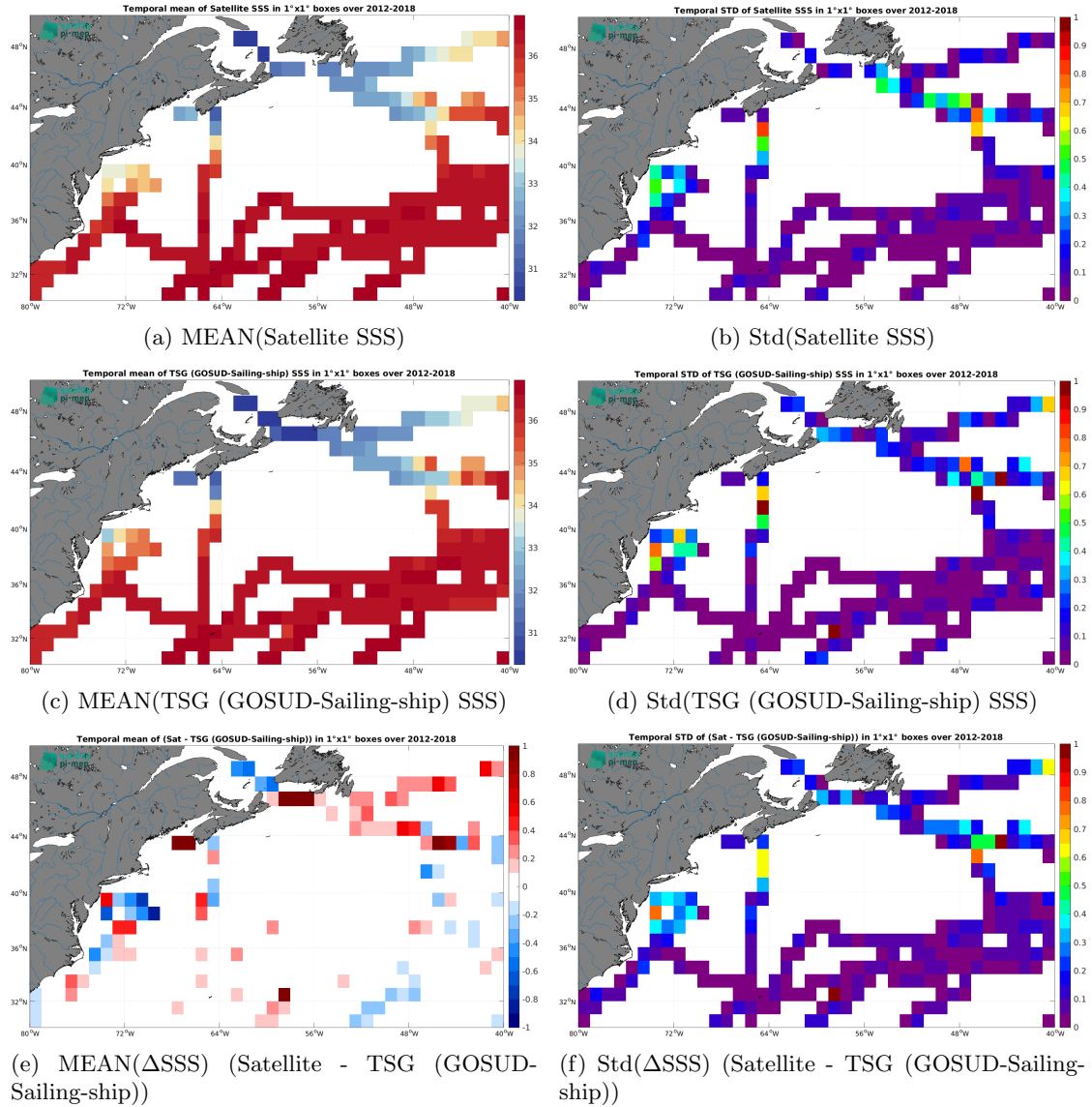
Figure 7: Temporal mean (left) and Std (right) of SSS from CCI SSS L4 Merged-OI v4.41 - 7-day running (ESA) (top), TSG (GOSUD-Sailing-ship) (middle), and of \Delta SSS (Satellite - TSG (GOSUD-Sailing-ship)). Only match-up pairs are used to generate these maps.
