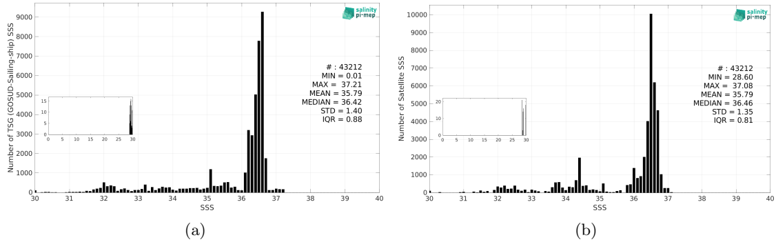
Figure 3: Histograms of SSS from TSG (GOSUD-Sailing-ship) (a) and CCI SSS L4 Merged-OI v4.41 - 7-day running (ESA) (b) considering all match-up pairs per bins of 0.1 over the Gulf Stream Pi-MEP region and for the full satellite product period.
