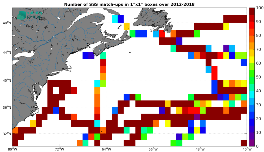
Figure 5: Number of SSS match-ups between TSG (GOSUD-Sailing-ship) SSS and the CCI SSS L4 Merged-OI v4.41 - 7-day running (ESA) SSS product for the Gulf Stream Pi-MEP region over 1^\circ \times 1^\circ boxes and for the full satellite product period.
