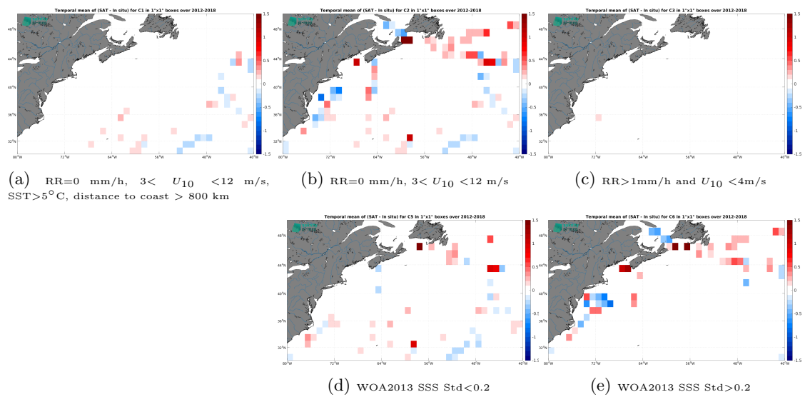
Figure 14: Temporal mean gridded over spatial boxes of size 1^\circ \times 1^\circ of \Delta SSS (CCI SSS L4 Merged-OI v4.41 - 7-day running (ESA) - TSG (GOSUD-Sailing-ship)) for 5 different subdatasets corresponding to:RR=0 mm/h, 3 < U_{10} < 12 m/s, SST >5^\circ C, distance to coast > 800 km (a), RR=0 mm/h, 3 < U_{10} < 12 m/s (b), RR >1 mm/h and U_{10} < 4 m/s (c), WOA2013 SSS Std <0.2 (d), WOA2013 SSS Std >0.2 (e).
