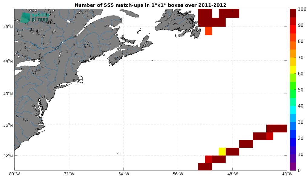
Figure 5: Number of SSS match-ups between TSG (CSIC-UTM) SSS and the CCI SSS L4 Merged-OI v4.41 - 7-day running (ESA) SSS product for the Gulf Stream Pi-MEP region over 1^\circ \times 1^\circ boxes and for the full satellite product period.
