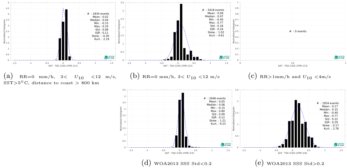
Figure 15: Normalized histogram of \Delta SSS (CCI SSS L4 Merged-OI v4.41 - 7-day running (ESA) - TSG (CSIC-UTM)) for 5 different subdatasets corresponding to: RR=0 mm/h, 3 < U_{10} < 12 m/s, SST>5°C, distance to coast > 800 km (a), RR=0 mm/h, 3 < U_{10} < 12 m/s (b), RR>1mm/h and U_{10} < 4 m/s (c), WOA2013 SSS Std<0.2 (d), WOA2013 SSS Std>0.2 (e).
