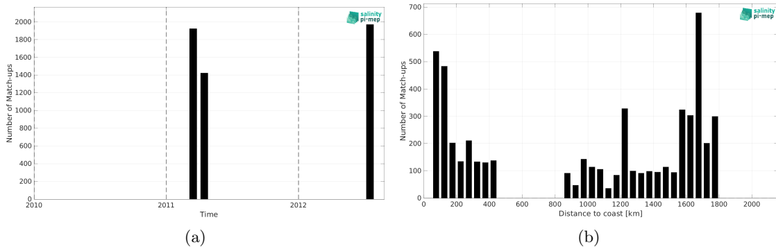
Figure 2: Number of match-ups between TSG (CSIC-UTM) and CCI SSS L4 Merged-OI v4.41 - 7-day running (ESA) SSS as a function of time (a) and as function of the distance to coast (b) over the Gulf Stream Pi-MEP region and for the full satellite product period.
