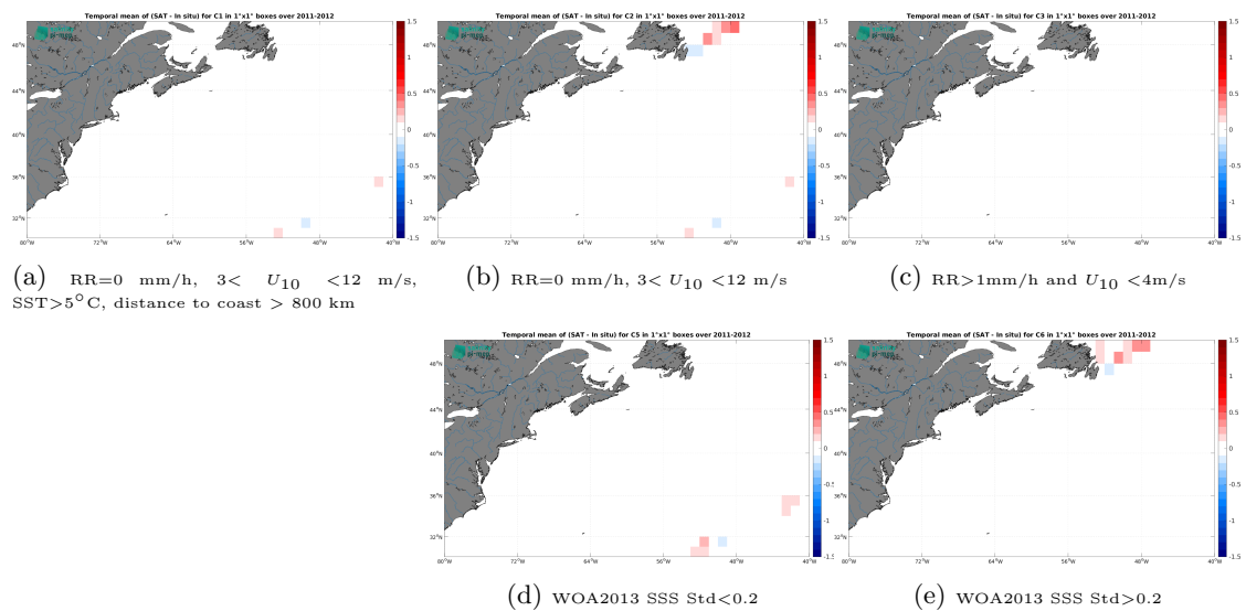
Figure 14: Temporal mean gridded over spatial boxes of size 1^\circ \times 1^\circ of \Delta SSS (CCI SSS L4 Merged-OI v4.41 - 7-day running (ESA) - TSG (CSIC-UTM)) for 5 different subdatasets corresponding to:RR=0 mm/h, 3 < U_{10} < 12 m/s, SST >5^\circ C, distance to coast > 800 km (a), RR=0 mm/h, 3 < U_{10} < 12 m/s (b), RR >1 mm/h and U_{10} < 4 m/s (c), WOA2013 SSS Std <0.2 (d), WOA2013 SSS Std >0.2 (e).
