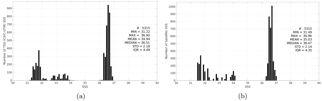
Figure 3: Histograms of SSS from TSG (CSIC-UTM) (a) and CCI SSS L4 Merged-OI v4.41 - 7-day running (ESA) (b) considering all match-up pairs per bins of 0.1 over the Gulf Stream Pi-MEP region and for the full satellite product period.
