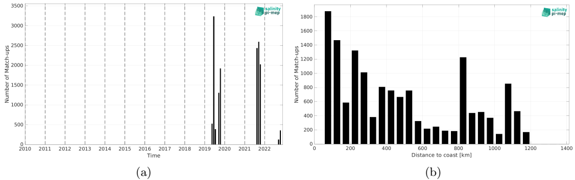
Figure 2: Number of match-ups between Saildrone and CCI SSS L4 Merged-OI v4.41 - 7-day running (ESA) SSS as a function of time (a) and as function of the distance to coast (b) over the Gulf Stream Pi-MEP region and for the full satellite product period.
