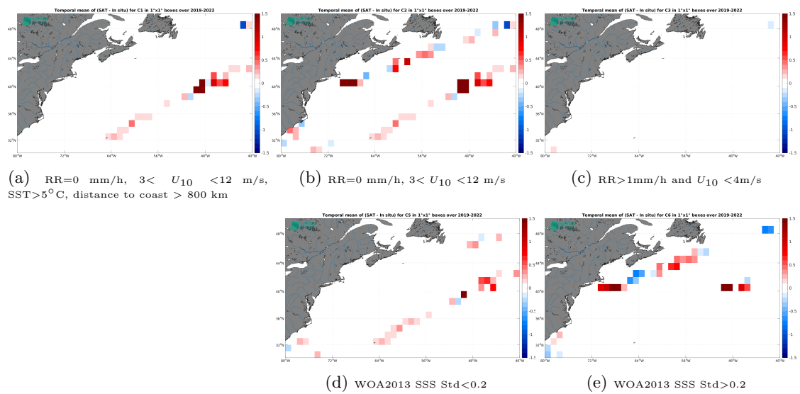
Figure 14: Temporal mean gridded over spatial boxes of size 1^\circ \times 1^\circ of \Delta SSS (CCI SSS L4 Merged-OI v4.41 - 7-day running (ESA) - Saildrone) for 5 different subdatasets corresponding to:RR=0 mm/h, 3 < U_{10} < 12 m/s, SST >5^\circ\text{C} , distance to coast > 800 km (a), RR=0 mm/h, 3 < U_{10} < 12 m/s (b), RR >1 mm/h and U_{10} < 4 m/s (c), WOA2013 SSS Std <0.2 (d), WOA2013 SSS Std >0.2 (e).
