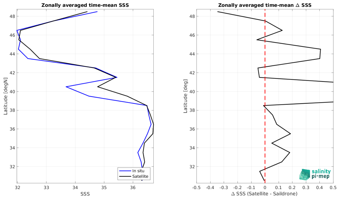
Figure 9: Left panel: Zonal mean SSS from CCI SSS L4 Merged-OI v4.41 - 7-day running (ESA) satellite product (black) and from Sairdron (blue). Right panel: Zonal mean of \Delta SSS (Satellite - Sairdron) for all the collected Pi-MEP match-up pairs estimated over the full satellite product period.
