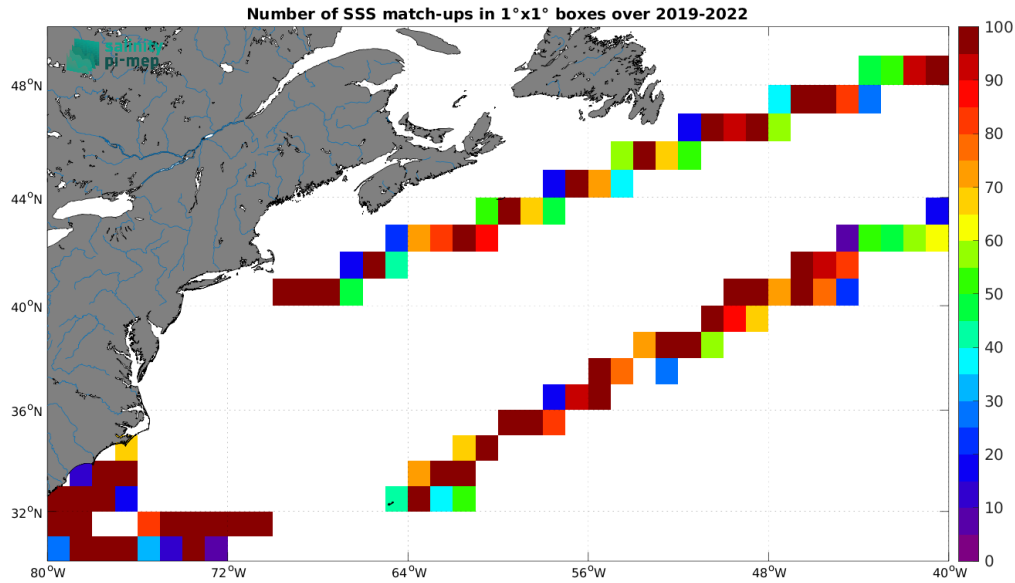
Figure 5: Number of SSS match-ups between Saildrone SSS and the CCI SSS L4 Merged-OI v4.41 - 7-day running (ESA) SSS product for the Gulf Stream Pi-MEP region over 1^\circ \times 1^\circ boxes and for the full satellite product period.
