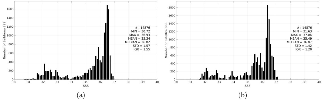
Figure 3: Histograms of SSS from Saildrone (a) and CCI SSS L4 Merged-OI v4.41 - 7-day running (ESA) (b) considering all match-up pairs per bins of 0.1 over the Gulf Stream Pi-MEP region and for the full satellite product period.
