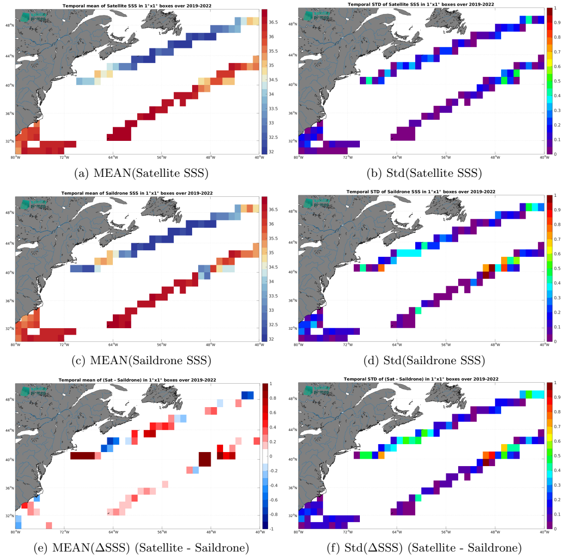
Figure 7: Temporal mean (left) and Std (right) of SSS from CCI SSS L4 Merged-OI v4.41 - 7-day running (ESA) (top), Saildrone (middle), and of \Delta SSS (Satellite - Saildrone). Only match-up pairs are used to generate these maps.
