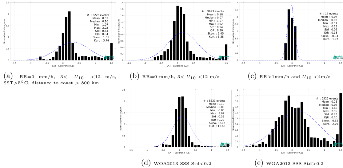
Figure 15: Normalized histogram of \Delta\text{SSS} (CCI SSS L4 Merged-OI v4.41 - 7-day running (ESA) - Saildrone) for 5 different subdatasets corresponding to: RR=0 mm/h, 3 < U_{10} < 12 m/s, SST>5°C, distance to coast > 800 km (a), RR=0 mm/h, 3 < U_{10} < 12 m/s (b), RR>1mm/h and U_{10} < 4 m/s (c), WOA2013 SSS Std<0.2 (d), WOA2013 SSS Std>0.2 (e).
