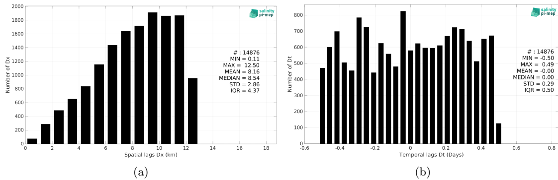
Figure 6: Histograms of the spatial (a) and temporal (b) lags between the location/time of the Saildrone measurement and the date of the corresponding CCI SSS L4 Merged-OI v4.41 - 7-day running (ESA) SSS pixel.
