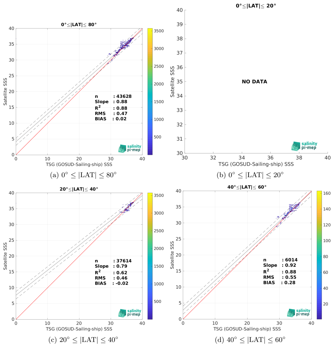
Figure 10: Contour maps of the concentration of CCI SSS L4 Merged-OI v4.41 - 30-day running (ESA) SSS (y-axis) versus TSG (GOSUD-Sailing-ship) SSS (x-axis) at match-up pairs for different latitude bands. For each plot, the red line shows x=y . The black thin and dashed lines indicate a linear fit through the data cloud and the \pm 95\% confidence levels, respectively. The number match-up pairs n , the slope and R^2 coefficient of the linear fit, the root mean square (RMS) and the mean bias between satellite and in situ data are indicated for each latitude band in each plots.
