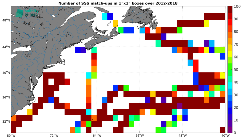
Figure 5: Number of SSS match-ups between TSG (GOSUD-Sailing-ship) SSS and the CCI SSS L4 Merged-OI v4.41 - 30-day running (ESA) SSS product for the Gulf Stream Pi-MEP region over 1^\circ \times 1^\circ boxes and for the full satellite product period.
