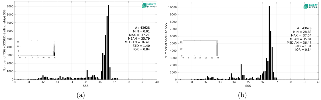
Figure 3: Histograms of SSS from TSG (GOSUD-Sailing-ship) (a) and CCI SSS L4 Merged-OI v4.41 - 30-day running (ESA) (b) considering all match-up pairs per bins of 0.1 over the Gulf Stream Pi-MEP region and for the full satellite product period.
