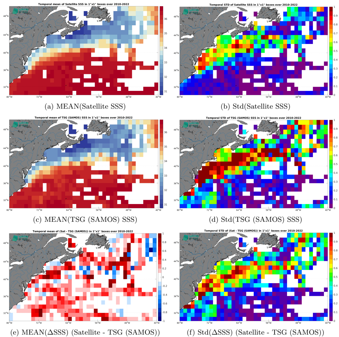
Figure 6: Temporal mean (left) and Std (right) of SSS from CCI SSS L4 Merged-OI v4.4 - 7-day running (ESA) (top), TSG (SAMOS) (middle), and of \Delta SSS (Satellite - TSG (SAMOS)). Only match-up pairs are used to generate these maps.
