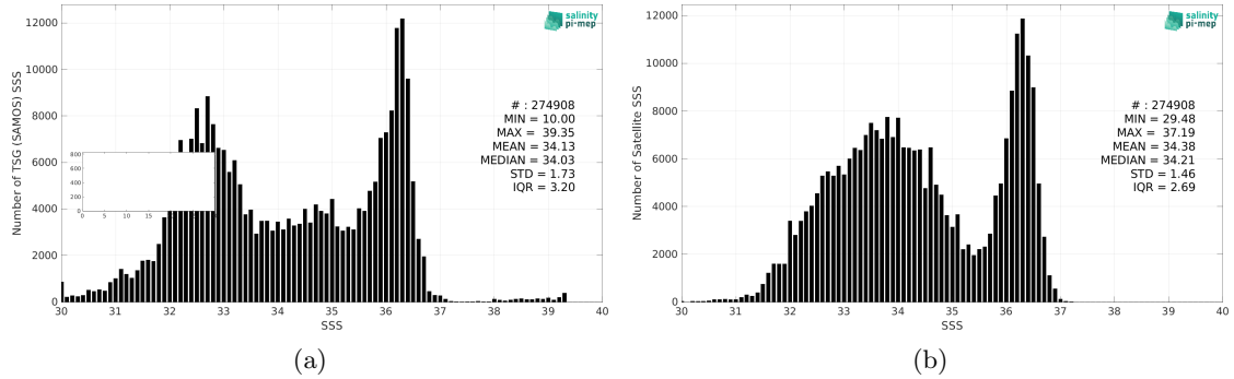
Figure 2: Histograms of SSS from TSG (SAMOS) (a) and CCI SSS L4 Merged-OI v4.4 - 7-day running (ESA) (b) considering all match-up pairs per bins of 0.1 over the Gulf Stream Pi-MEP region and for the full satellite product period.
