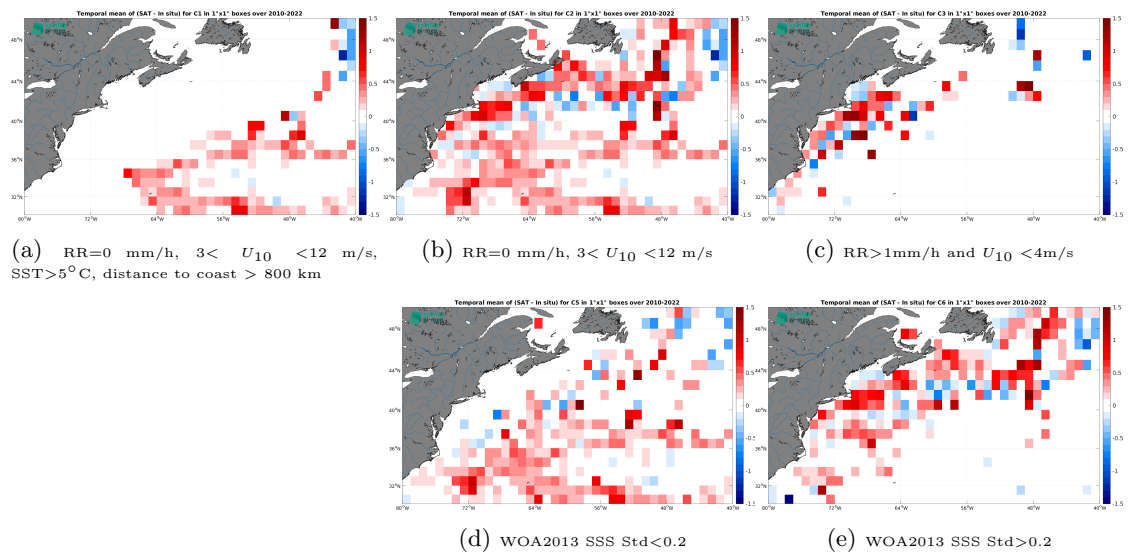
Figure 12: Temporal mean gridded over spatial boxes of size 1^\circ \times 1^\circ of \Delta SSS (CCI SSS L4 Merged-OI v4.4 - 7-day running (ESA) - TSG (SAMOS)) for 5 different subdatasets corresponding to:RR=0 mm/h, 3 < U_{10} < 12 m/s, SST >5^\circ C, distance to coast > 800 km (a), RR=0 mm/h, 3 < U_{10} < 12 m/s (b), RR >1 mm/h and U_{10} < 4 m/s (c), WOA2013 SSS Std <0.2 (d), WOA2013 SSS Std >0.2 (e).
