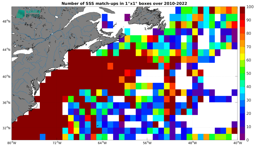
Figure 4: Number of SSS match-ups between TSG (SAMOS) SSS and the CCI SSS L4 Merged-OI v4.4 - 7-day running (ESA) SSS product for the Gulf Stream Pi-MEP region over 1^\circ \times 1^\circ boxes and for the full satellite product period.
