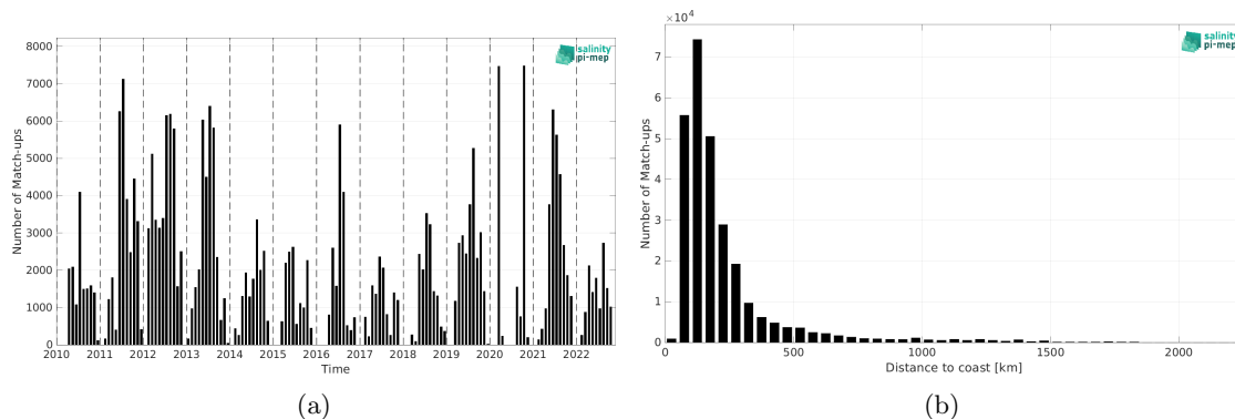
Figure 1: Number of match-ups between TSG (SAMOS) and CCI SSS L4 Merged-OI v4.4 - 7-day running (ESA) SSS as a function of time (a) and as function of the distance to coast (b) over the Gulf Stream Pi-MEP region and for the full satellite product period.
