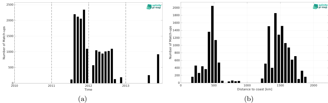
Figure 1: Number of match-ups between Surface drifters and CCI SSS L4 Merged-OI v4.4 - 30-day running (ESA) SSS as a function of time (a) and as function of the distance to coast (b) over the Gulf Stream Pi-MEP region and for the full satellite product period.
