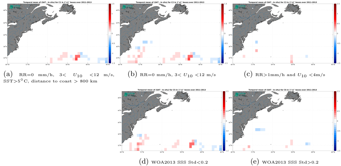
Figure 11: Temporal mean gridded over spatial boxes of size 1^{\circ}\times 1^{\circ} of \Delta\text{SSS} (CCI SSS L4 Merged-OI v4.4 - 30-day running (ESA) - Surface drifters) for 5 different subdatasets corresponding to:RR=0 mm/h, 3 < U_{10} < 12 m/s, SST >5^{\circ}\text{C} , distance to coast > 800 km (a), RR=0 mm/h, 3 < U_{10} < 12 m/s (b), RR >1 mm/h and U_{10} < 4 m/s (c), WOA2013 SSS Std <0.2 (d), WOA2013 SSS Std >0.2 (e).
