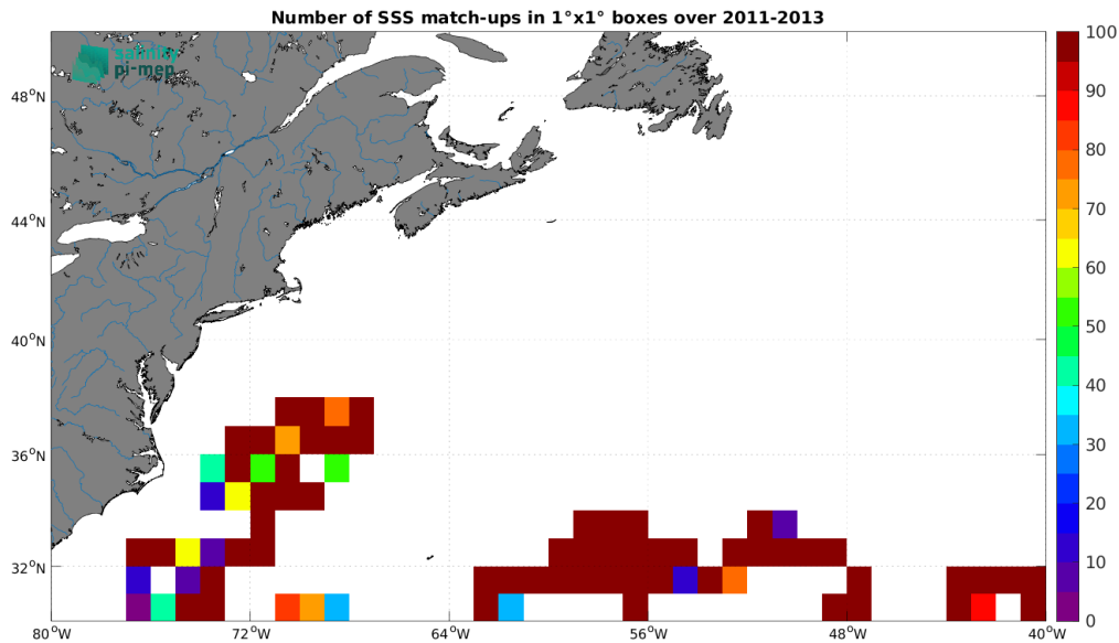
Figure 3: Number of SSS match-ups between Surface drifters SSS and the CCI SSS L4 Merged-OI v4.4 - 30-day running (ESA) SSS product for the Gulf Stream Pi-MEP region over 1^\circ \times 1^\circ boxes and for the full satellite product period.
