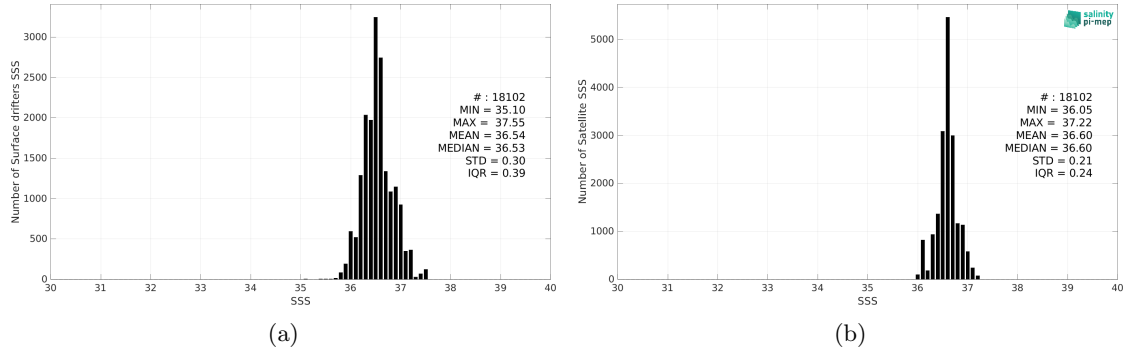
Figure 2: Histograms of SSS from Surface drifters (a) and CCI SSS L4 Merged-OI v4.4 - 30-day running (ESA) (b) considering all match-up pairs per bins of 0.1 over the Gulf Stream Pi-MEP region and for the full satellite product period.
