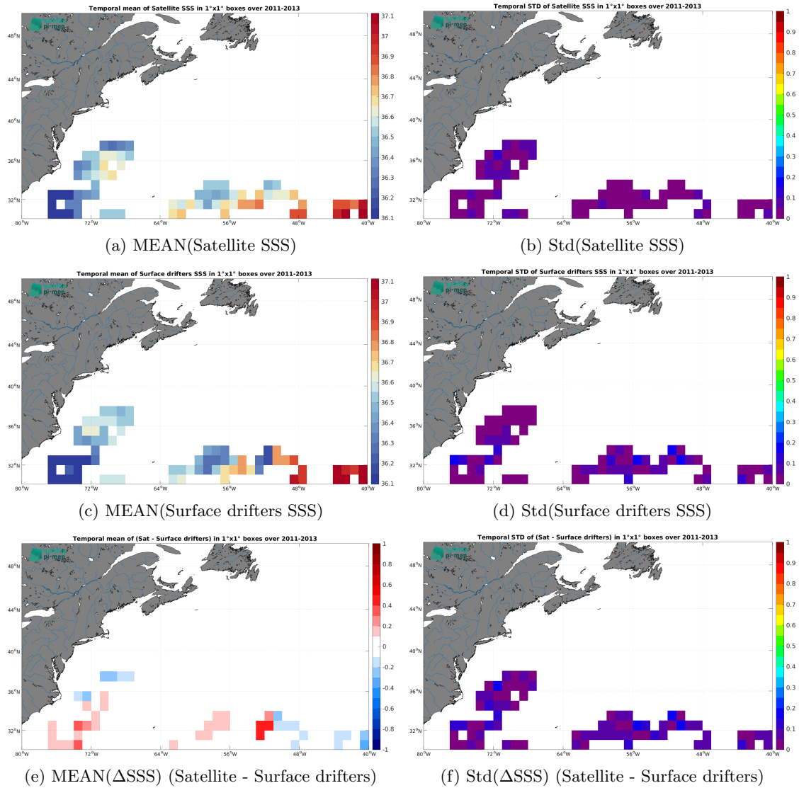
Figure 5: Temporal mean (left) and Std (right) of SSS from CCI SSS L4 Merged-OI v4.4 - 30-day running (ESA) (top), Surface drifters (middle), and of \Delta SSS (Satellite - Surface drifters). Only match-up pairs are used to generate these maps.
