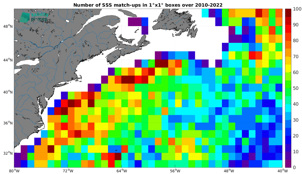
Figure 4: Number of SSS match-ups between Argo SSS and the CCI SSS L4 Merged-OI v4.4 - 30-day running (ESA) SSS product for the Gulf Stream Pi-MEP region over 1^\circ \times 1^\circ boxes and for the full satellite product period.
