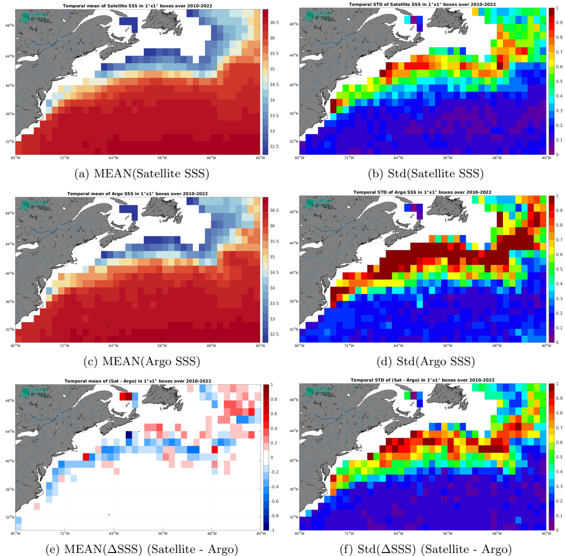
Figure 6: Temporal mean (left) and Std (right) of SSS from CCI SSS L4 Merged-OI v4.4 - 30-day running (ESA) (top), Argo (middle), and of \Delta SSS (Satellite - Argo). Only match-up pairs are used to generate these maps.
