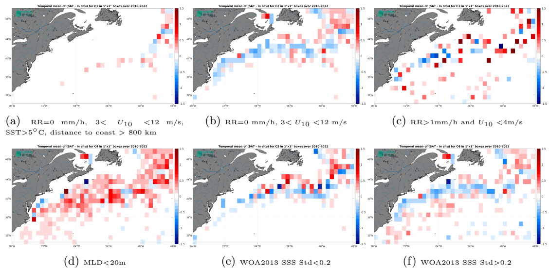
Figure 12: Temporal mean gridded over spatial boxes of size 1^\circ \times 1^\circ of \Delta SSS (CCI SSS L4 Merged-OI v4.4 - 30-day running (ESA) - Argo) for 6 different subdatasets corresponding to:RR=0 mm/h, 3 < U_{10} < 12 m/s, SST > 5^\circ\text{C} , distance to coast > 800 km (a), RR=0 mm/h, 3 < U_{10} < 12 m/s (b), RR > 1 mm/h and U_{10} < 4 m/s (c),MLD < 20 m (d),WOA2013 SSS Std < 0.2 (e),WOA2013 SSS Std > 0.2 (f).
