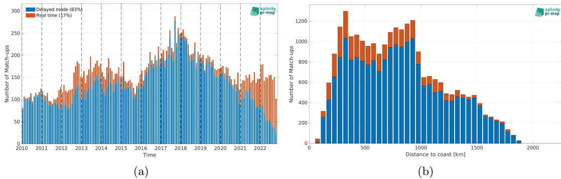
Figure 1: Number of match-ups between Argo and CCI SSS L4 Merged-OI v4.4 - 30-day running (ESA) SSS as a function of time (a) and as function of the distance to coast (b) over the Gulf Stream Pi-MEP region and for the full satellite product period.
