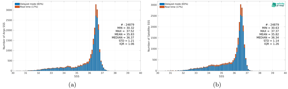
Figure 2: Histograms of SSS from Argo (a) and CCI SSS L4 Merged-OI v4.4 - 30-day running (ESA) (b) considering all match-up pairs per bins of 0.1 over the Gulf Stream Pi-MEP region and for the full satellite product period.
