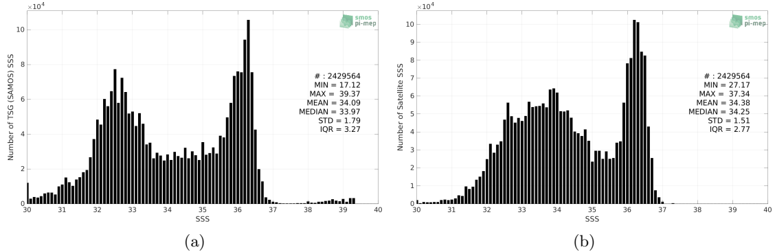
Figure 2: Histograms of SSS from TSG (SAMOS) (a) and CCI SSS L4 Merged-OI v3.2 - 7-day running (ESA) (b) considering all match-up pairs per bins of 0.1 over the Gulf Stream Pi-MEP region and for the full satellite product period.
