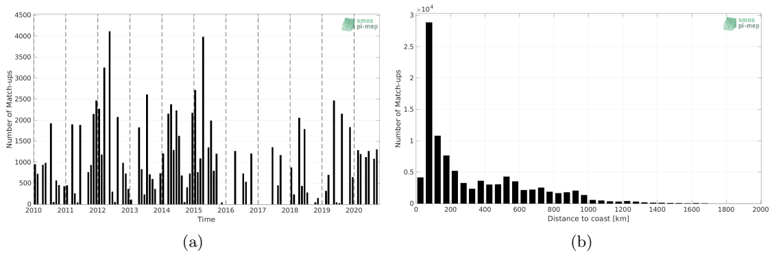
Figure 1: Number of match-ups between TSG (LEGOS-DM) and CCI SSS L4 Merged-OI v3.2 - 7-day running (ESA) SSS as a function of time (a) and as function of the distance to coast (b) over the Gulf Stream Pi-MEP region and for the full satellite product period.
