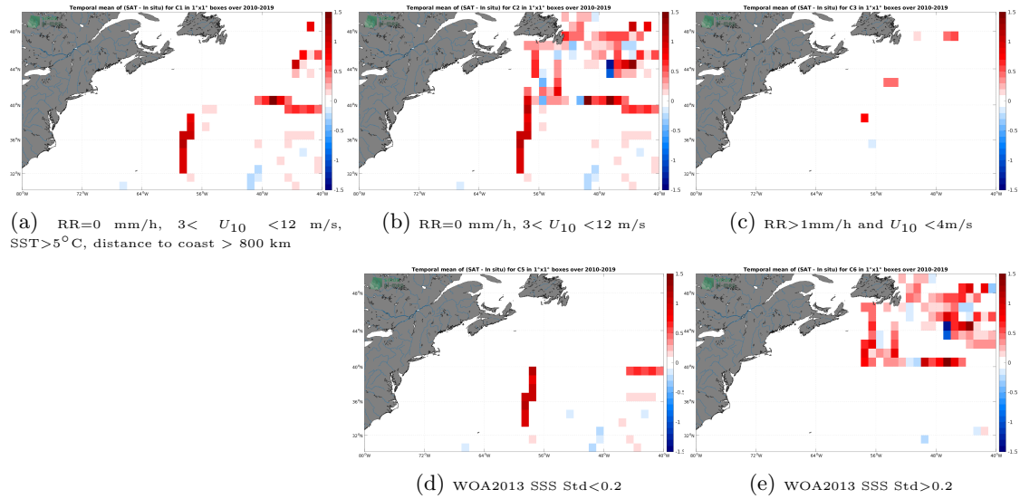
Figure 12: Temporal mean gridded over spatial boxes of size 1^{\circ}\times 1^{\circ} of \Delta SSS (CCI SSS L4 Merged-OI v3.2 - 7-day running (ESA) - TSG (GOSUD-Research-vessel)) for 5 different subdatasets corresponding to:RR=0 mm/h, 3 < U_{10} < 12 m/s, SST >5^{\circ}\text{C} , distance to coast > 800 km (a), RR=0 mm/h, 3 < U_{10} < 12 m/s (b), RR >1 mm/h and U_{10} < 4 m/s (c), WOA2013 SSS Std <0.2 (d), WOA2013 SSS Std >0.2 (e).
