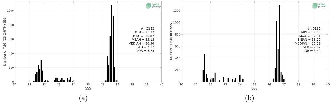
Figure 2: Histograms of SSS from TSG (CSIC-UTM) (a) and CCI SSS L4 Merged-OI v3.2 - 7-day running (ESA) (b) considering all match-up pairs per bins of 0.1 over the Gulf Stream Pi-MEP region and for the full satellite product period.
