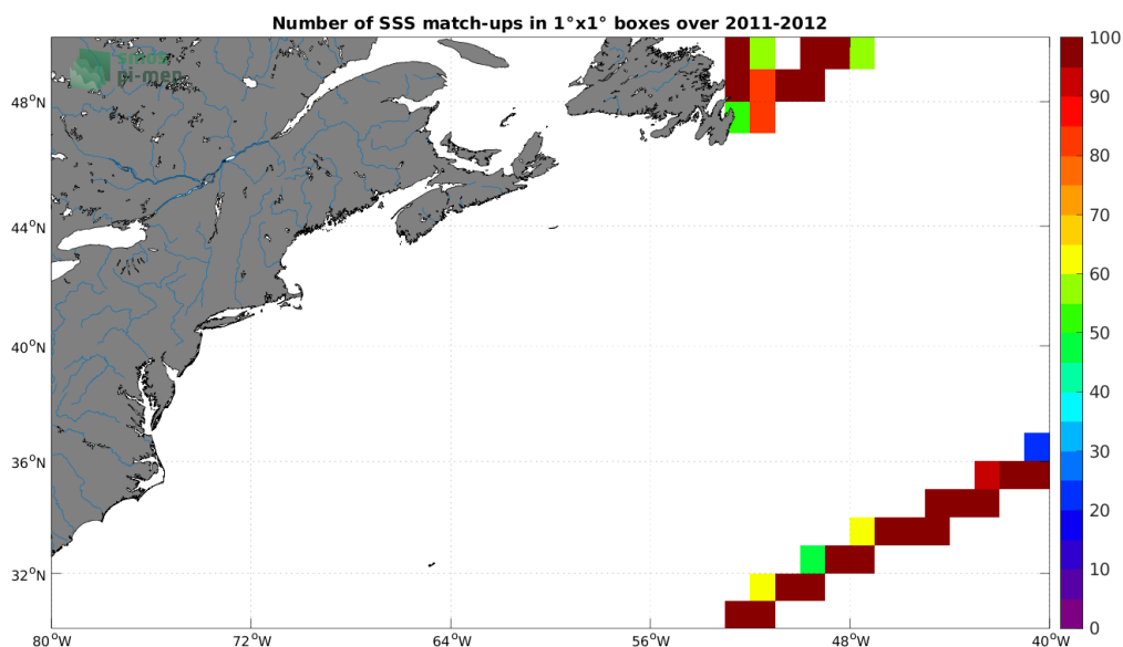
Figure 4: Number of SSS match-ups between TSG (CSIC-UTM) SSS and the CCI SSS L4 Merged-OI v3.2 - 7-day running (ESA) SSS product for the Gulf Stream Pi-MEP region over 1^\circ \times 1^\circ boxes and for the full satellite product period.
