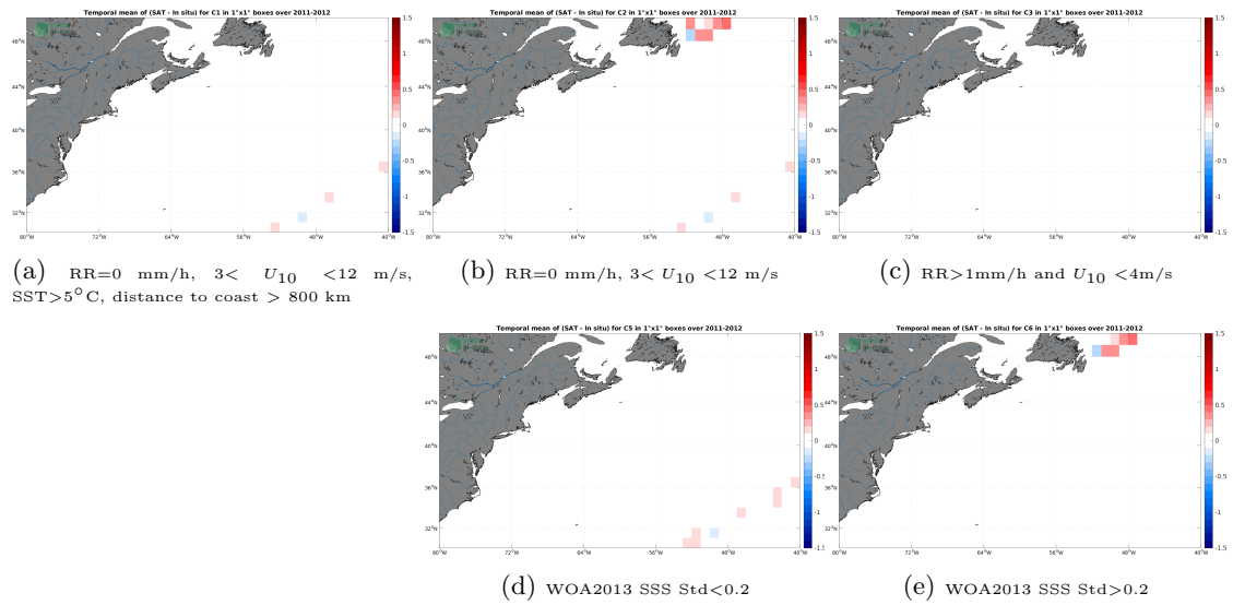
Figure 12: Temporal mean gridded over spatial boxes of size 1^\circ \times 1^\circ of \Delta SSS (CCI SSS L4 Merged-OI v3.2 - 7-day running (ESA) - TSG (CSIC-UTM)) for 5 different subdatasets corresponding to:RR=0 mm/h, 3 < U_{10} < 12 m/s, SST >5^\circ C, distance to coast > 800 km (a), RR=0 mm/h, 3 < U_{10} < 12 m/s (b), RR >1 mm/h and U_{10} < 4 m/s (c), WOA2013 SSS Std <0.2 (d), WOA2013 SSS Std >0.2 (e).
