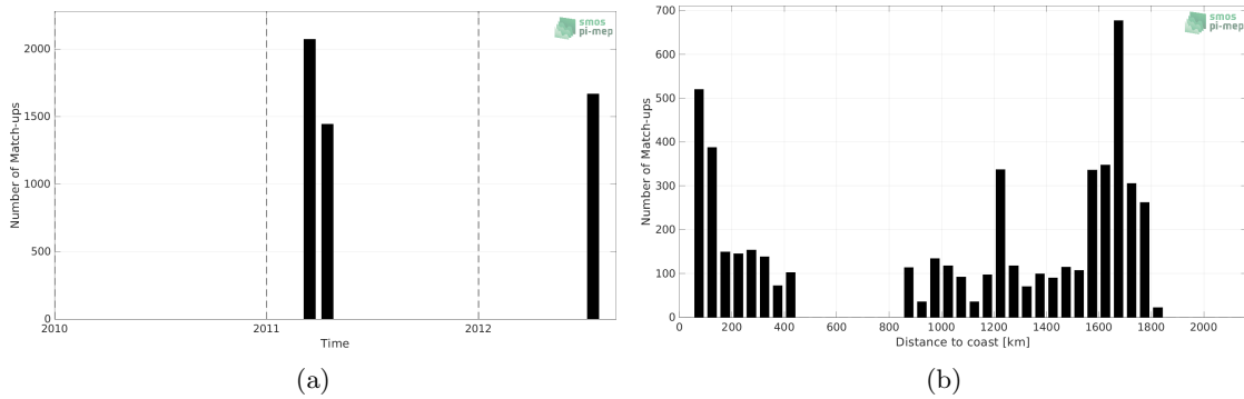
Figure 1: Number of match-ups between TSG (CSIC-UTM) and CCI SSS L4 Merged-OI v3.2 - 7-day running (ESA) SSS as a function of time (a) and as function of the distance to coast (b) over the Gulf Stream Pi-MEP region and for the full satellite product period.
