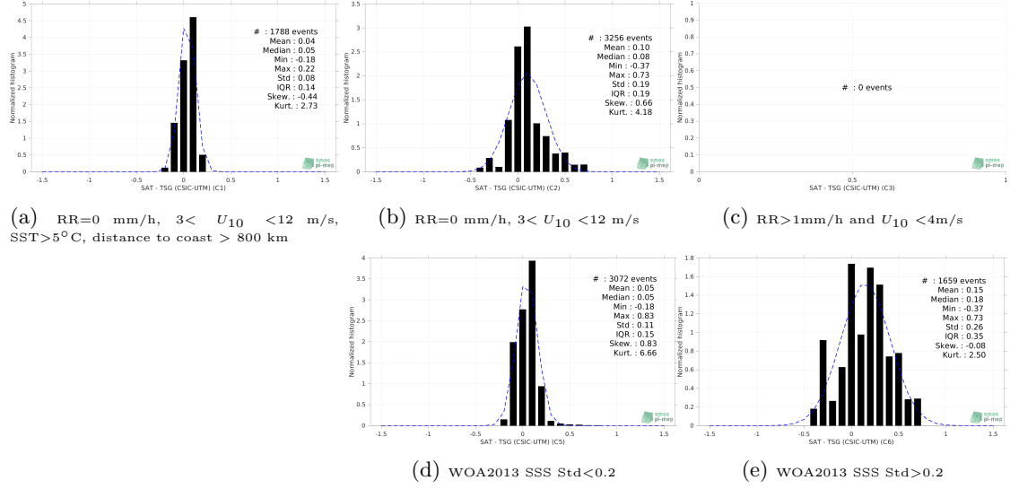
Figure 13: Normalized histogram of \Delta SSS (CCI SSS L4 Merged-OI v3.2 - 7-day running (ESA) - TSG (CSIC-UTM)) for 5 different subdatasets corresponding to: RR=0 mm/h, 3 < U_{10} < 12 m/s, SST>5°C, distance to coast > 800 km (a), RR=0 mm/h, 3 < U_{10} < 12 m/s (b), RR>1mm/h and U_{10} < 4 m/s (c), WOA2013 SSS Std<0.2 (d), WOA2013 SSS Std>0.2 (e).
