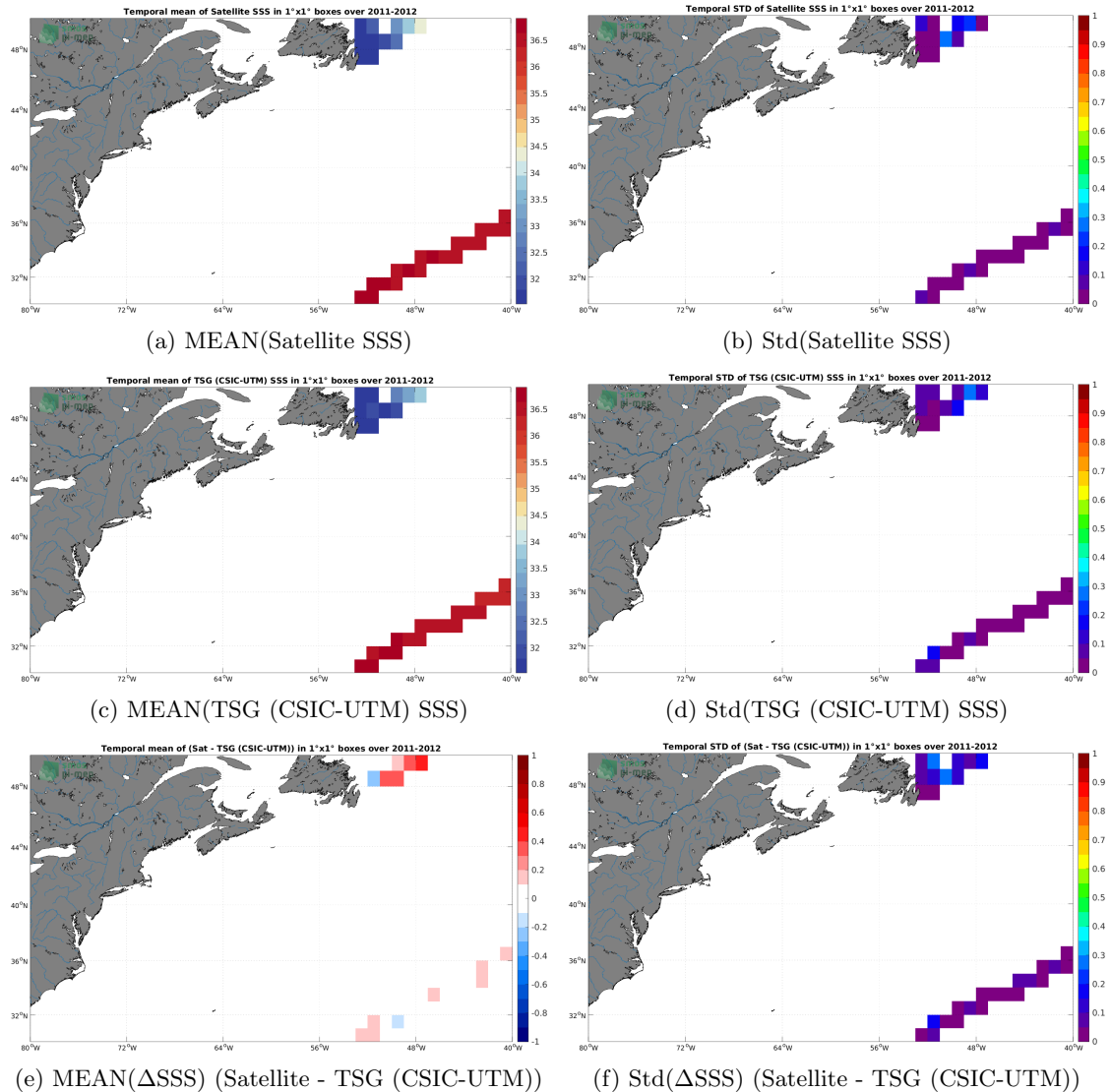
Figure 6: Temporal mean (left) and Std (right) of SSS from CCI SSS L4 Merged-OI v3.2 - 7-day running (ESA) (top), TSG (CSIC-UTM) (middle), and of \Delta SSS (Satellite - TSG (CSIC-UTM)). Only match-up pairs are used to generate these maps.
