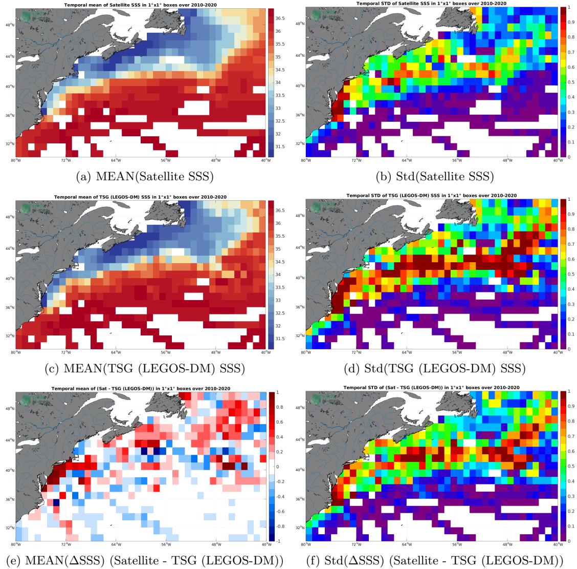
Figure 6: Temporal mean (left) and Std (right) of SSS from CCI SSS L4 Merged-OI v3.2 - 30-day running (ESA) (top), TSG (LEGOS-DM) (middle), and of \Delta SSS (Satellite - TSG (LEGOS-DM)). Only match-up pairs are used to generate these maps.
