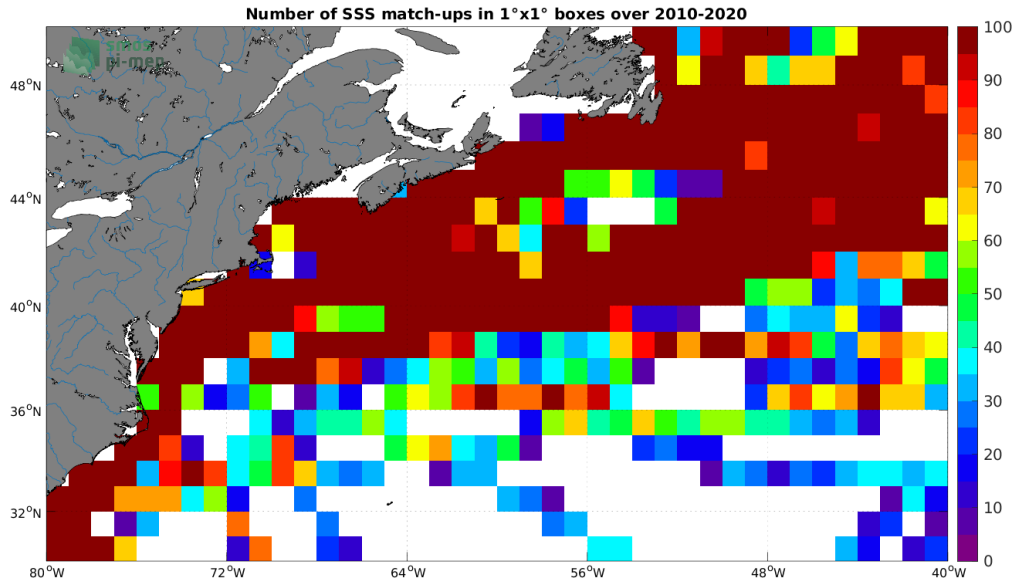
Figure 4: Number of SSS match-ups between TSG (LEGOS-DM) SSS and the CCI SSS L4 Merged-OI v3.2 - 30-day running (ESA) SSS product for the Gulf Stream Pi-MEP region over 1^\circ \times 1^\circ boxes and for the full satellite product period.
