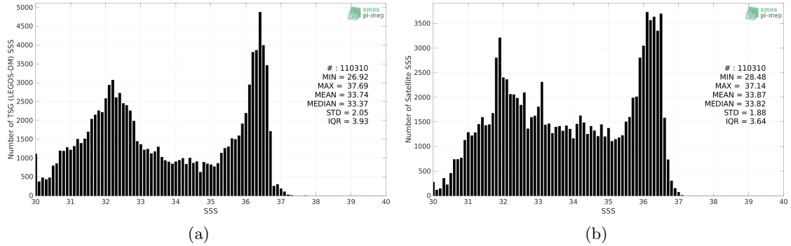
Figure 2: Histograms of SSS from TSG (LEGOS-DM) (a) and CCI SSS L4 Merged-OI v3.2 - 30-day running (ESA) (b) considering all match-up pairs per bins of 0.1 over the Gulf Stream Pi-MEP region and for the full satellite product period.
