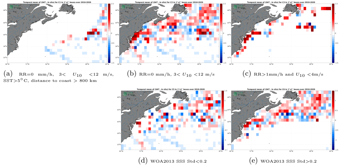
Figure 12: Temporal mean gridded over spatial boxes of size 1^{\circ}\times 1^{\circ} of \Delta\text{SSS} (CCI SSS L4 Merged-OI v3.2 - 30-day running (ESA) - TSG (LEGOS-DM)) for 5 different subdatasets corresponding to:RR=0 mm/h, 3 < U_{10} < 12 m/s, SST >5^{\circ}\text{C} , distance to coast > 800 km (a), RR=0 mm/h, 3 < U_{10} < 12 m/s (b), RR >1 mm/h and U_{10} < 4 m/s (c), WOA2013 SSS Std <0.2 (d), WOA2013 SSS Std >0.2 (e).
