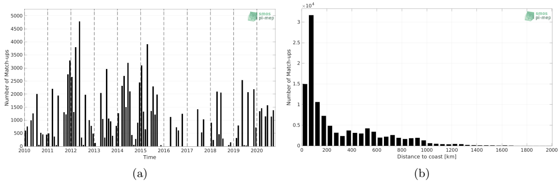
Figure 1: Number of match-ups between TSG (LEGOS-DM) and CCI SSS L4 Merged-OI v3.2 - 30-day running (ESA) SSS as a function of time (a) and as function of the distance to coast (b) over the Gulf Stream Pi-MEP region and for the full satellite product period.
