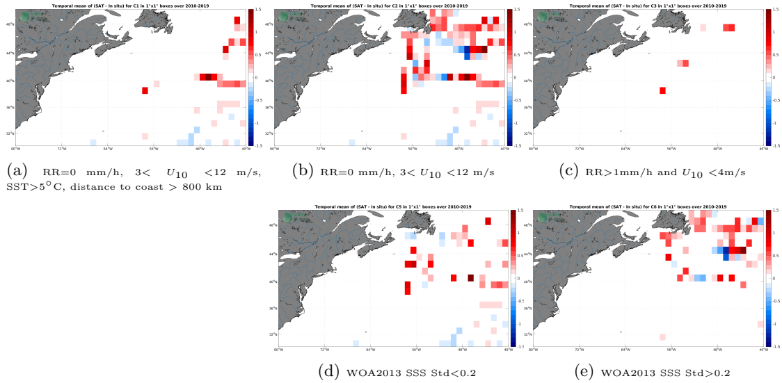
Figure 12: Temporal mean gridded over spatial boxes of size 1^\circ \times 1^\circ of \Delta SSS (CCI SSS L4 Merged-OI v3.2 - 30-day running (ESA) - TSG (GOSUD-Research-vessel)) for 5 different subdatasets corresponding to:RR=0 mm/h, 3 < U_{10} < 12 m/s, SST >5^\circ\text{C} , distance to coast > 800 km (a), RR=0 mm/h, 3 < U_{10} < 12 m/s (b), RR >1 mm/h and U_{10} < 4 m/s (c), WOA2013 SSS Std <0.2 (d), WOA2013 SSS Std >0.2 (e).
