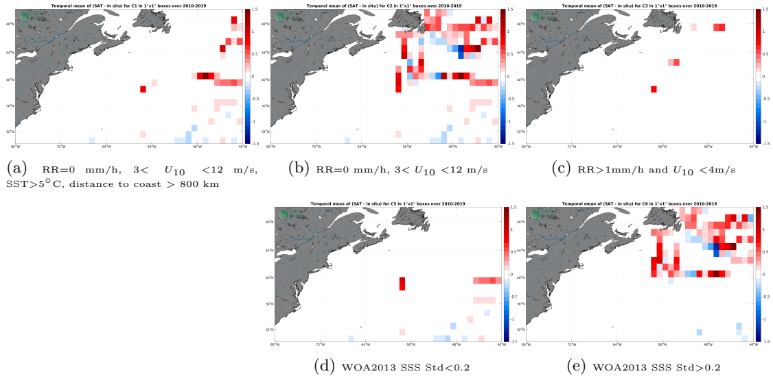
Figure 12: Temporal mean gridded over spatial boxes of size 1^{\circ}\times 1^{\circ} of \Delta SSS (CCI SSS L4 Merged-OI v3.2 - 30-day running (ESA) - TSG (GOSUD-Research-vessel)) for 5 different subdatasets corresponding to:RR=0 mm/h, 3 < U_{10} < 12 m/s, SST >5^{\circ}\text{C} , distance to coast > 800 km (a), RR=0 mm/h, 3 < U_{10} < 12 m/s (b), RR >1 mm/h and U_{10} < 4 m/s (c), WOA2013 SSS Std <0.2 (d), WOA2013 SSS Std >0.2 (e).
