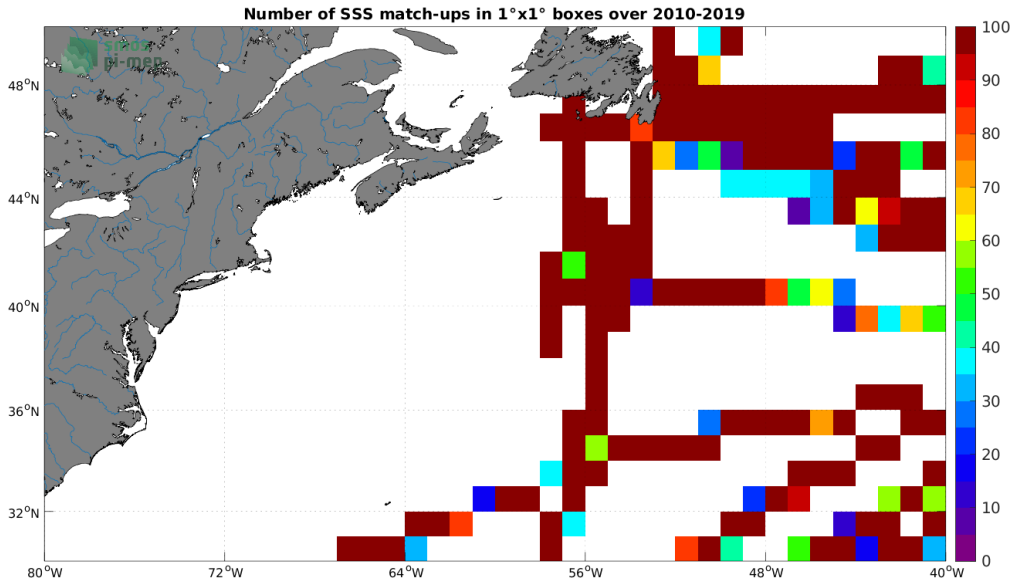
Figure 4: Number of SSS match-ups between TSG (GOSUD-Research-vessel) SSS and the CCI SSS L4 Merged-OI v3.2 - 30-day running (ESA) SSS product for the Gulf Stream Pi-MEP region over 1^\circ \times 1^\circ boxes and for the full satellite product period.
