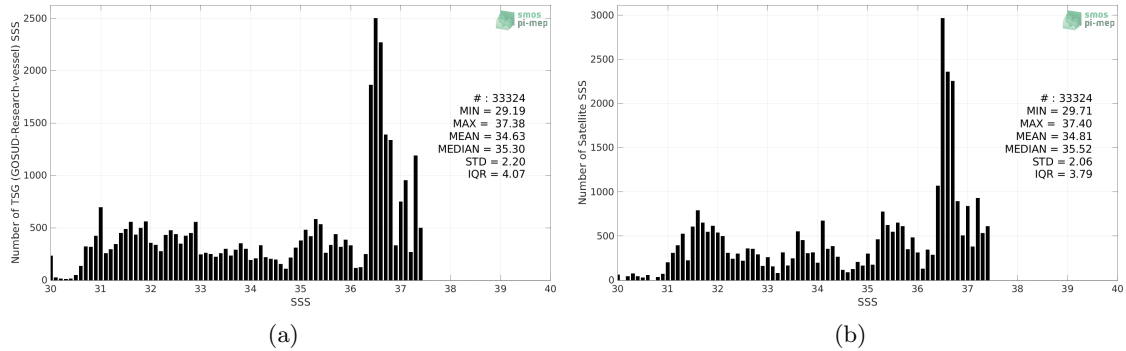
Figure 2: Histograms of SSS from TSG (GOSUD-Research-vessel) (a) and CCI SSS L4 Merged-OI v3.2 - 30-day running (ESA) (b) considering all match-up pairs per bins of 0.1 over the Gulf Stream Pi-MEP region and for the full satellite product period.
