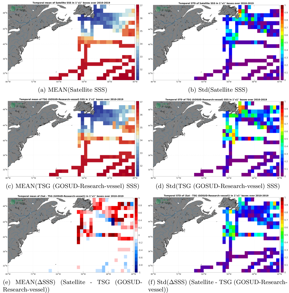
Figure 6: Temporal mean (left) and Std (right) of SSS from CCI SSS L4 Merged-OI v3.2 - 30-day running (ESA) (top), TSG (GOSUD-Research-vessel) (middle), and of \Delta SSS (Satellite - TSG (GOSUD-Research-vessel)). Only match-up pairs are used to generate these maps.
