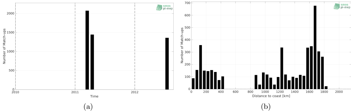
Figure 1: Number of match-ups between TSG (CSIC-UTM) and CCI SSS L4 Merged-OI v3.2 - 30-day running (ESA) SSS as a function of time (a) and as function of the distance to coast (b) over the Gulf Stream Pi-MEP region and for the full satellite product period.
