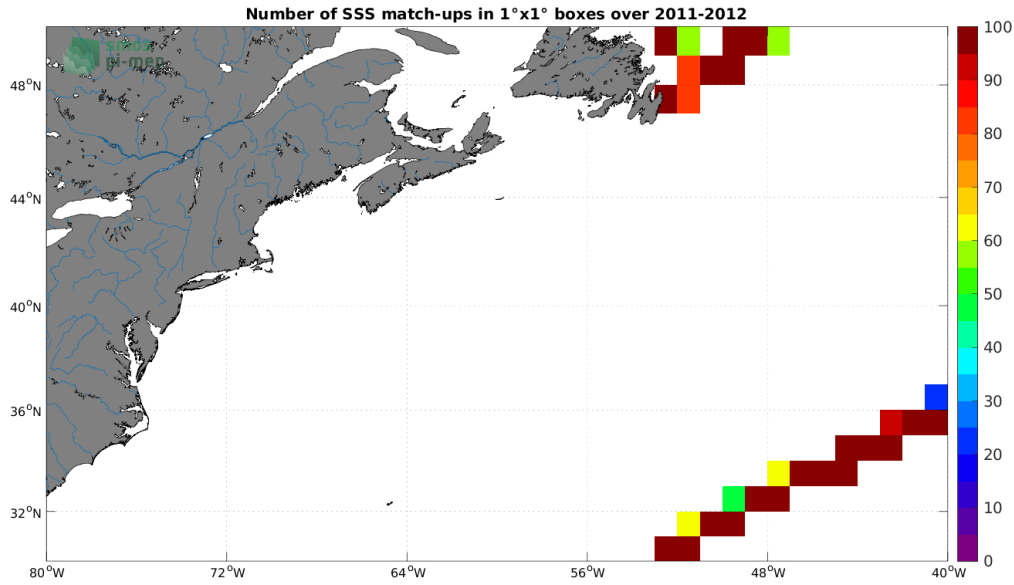
Figure 4: Number of SSS match-ups between TSG (CSIC-UTM) SSS and the CCI SSS L4 Merged-OI v3.2 - 30-day running (ESA) SSS product for the Gulf Stream Pi-MEP region over 1^\circ \times 1^\circ boxes and for the full satellite product period.
