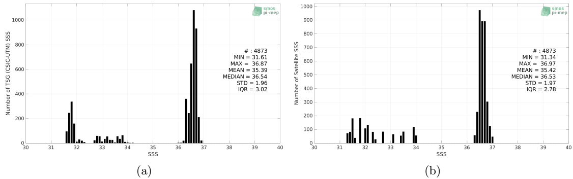
Figure 2: Histograms of SSS from TSG (CSIC-UTM) (a) and CCI SSS L4 Merged-OI v3.2 - 30-day running (ESA) (b) considering all match-up pairs per bins of 0.1 over the Gulf Stream Pi-MEP region and for the full satellite product period.
