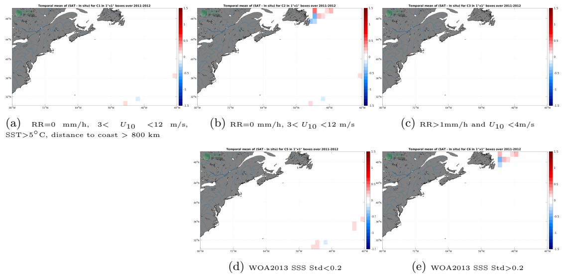
Figure 12: Temporal mean gridded over spatial boxes of size 1^\circ \times 1^\circ of \Delta SSS (CCI SSS L4 Merged-OI v3.2 - 30-day running (ESA) - TSG (CSIC-UTM)) for 5 different subdatasets corresponding to:RR=0 mm/h, 3 < U_{10} < 12 m/s, SST >5^\circ C, distance to coast > 800 km (a), RR=0 mm/h, 3 < U_{10} < 12 m/s (b), RR >1 mm/h and U_{10} < 4 m/s (c), WOA2013 SSS Std <0.2 (d), WOA2013 SSS Std >0.2 (e).
