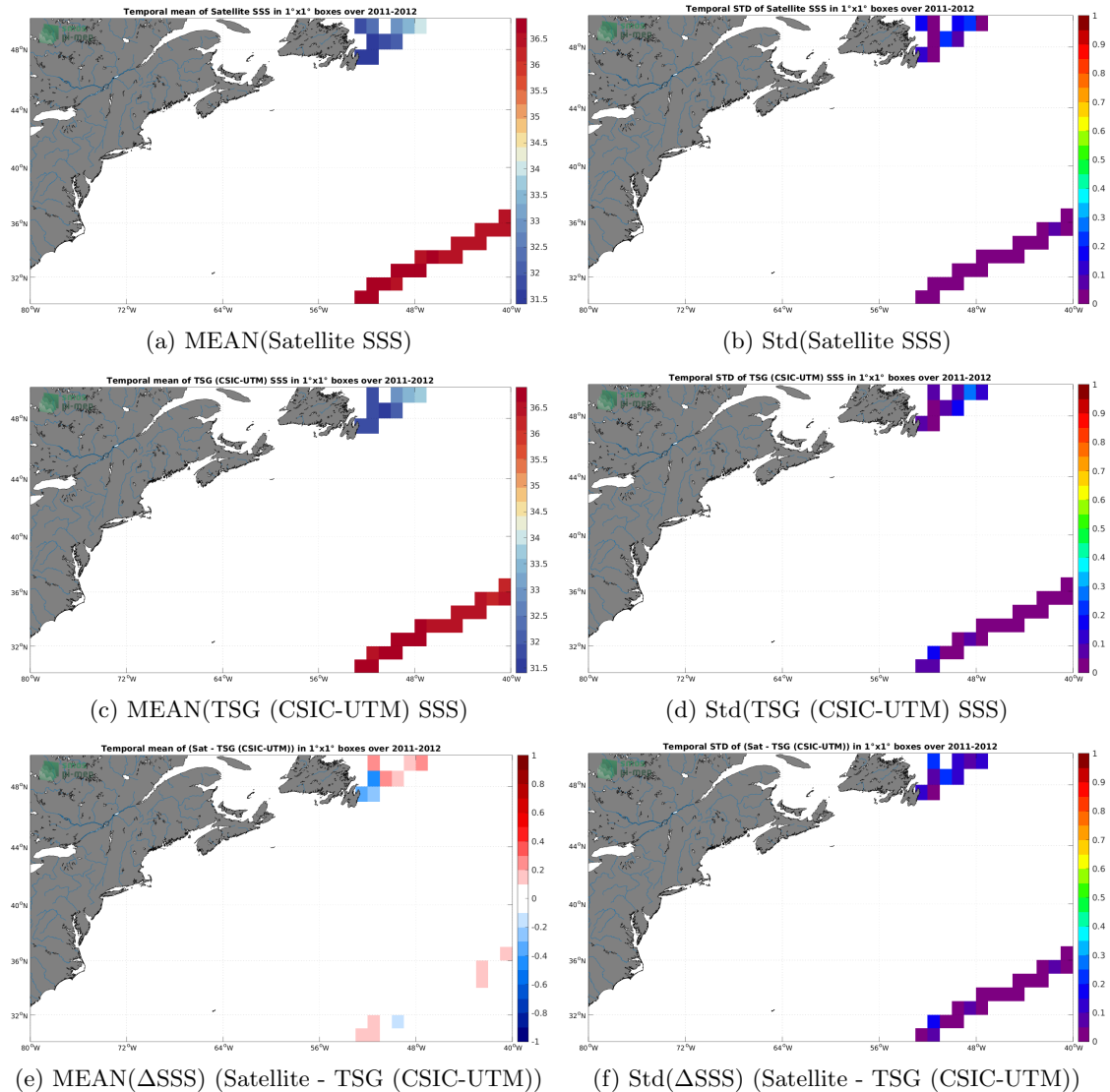
Figure 6: Temporal mean (left) and Std (right) of SSS from CCI SSS L4 Merged-OI v3.2 - 30-day running (ESA) (top), TSG (CSIC-UTM) (middle), and of \Delta SSS (Satellite - TSG (CSIC-UTM)). Only match-up pairs are used to generate these maps.
