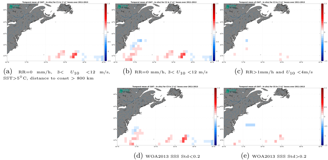
Figure 11: Temporal mean gridded over spatial boxes of size 1^{\circ}\times 1^{\circ} of \Delta\text{SSS} (CCI SSS L4 Merged-OI v3.2 - 30-day running (ESA) - Surface drifters) for 5 different subdatasets corresponding to:RR=0 mm/h, 3 < U_{10} < 12 m/s, SST >5^{\circ}\text{C} , distance to coast > 800 km (a), RR=0 mm/h, 3 < U_{10} < 12 m/s (b), RR >1 mm/h and U_{10} < 4 m/s (c), WOA2013 SSS Std <0.2 (d), WOA2013 SSS Std >0.2 (e).
