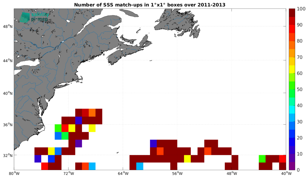
Figure 3: Number of SSS match-ups between Surface drifters SSS and the CCI SSS L4 Merged-OI v3.2 - 30-day running (ESA) SSS product for the Gulf Stream Pi-MEP region over 1^\circ \times 1^\circ boxes and for the full satellite product period.
