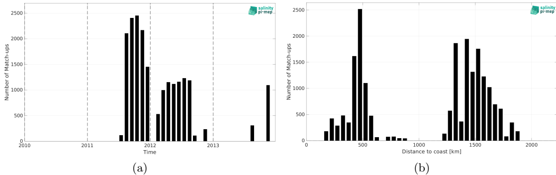
Figure 1: Number of match-ups between Surface drifters and CCI SSS L4 Merged-OI v3.2 - 30-day running (ESA) SSS as a function of time (a) and as function of the distance to coast (b) over the Gulf Stream Pi-MEP region and for the full satellite product period.
