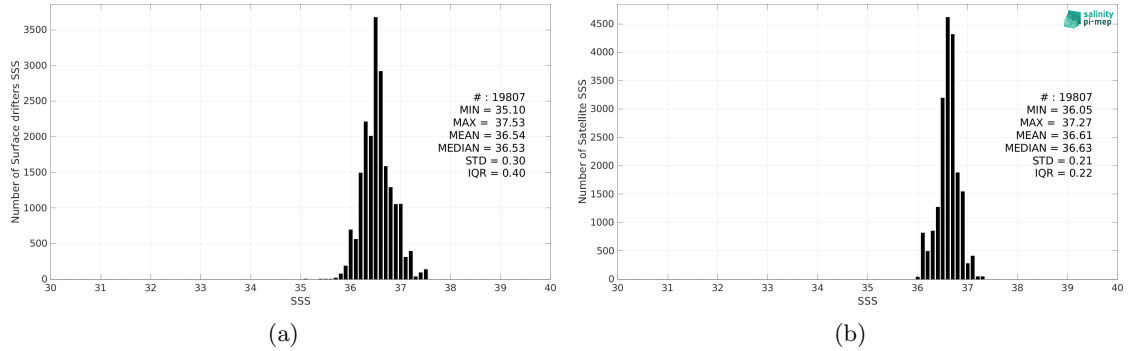
Figure 2: Histograms of SSS from Surface drifters (a) and CCI SSS L4 Merged-OI v3.2 - 30-day running (ESA) (b) considering all match-up pairs per bins of 0.1 over the Gulf Stream Pi-MEP region and for the full satellite product period.
