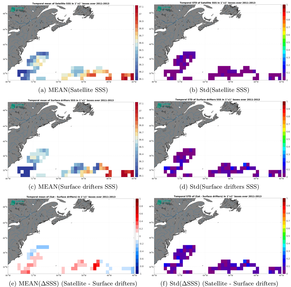
Figure 5: Temporal mean (left) and Std (right) of SSS from CCI SSS L4 Merged-OI v3.2 - 30-day running (ESA) (top), Surface drifters (middle), and of \Delta SSS (Satellite - Surface drifters). Only match-up pairs are used to generate these maps.
