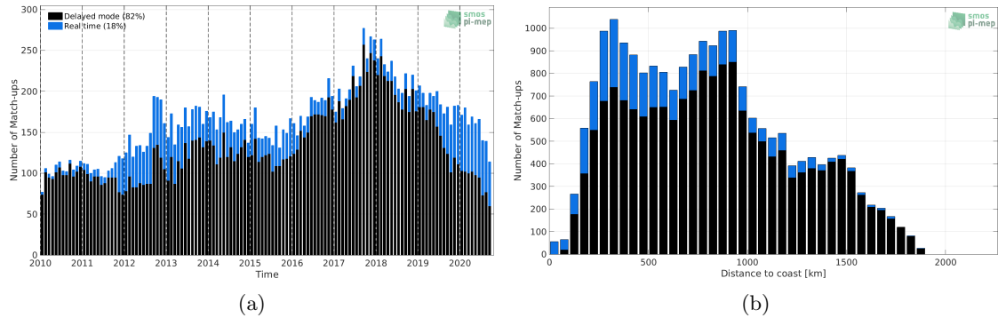
Figure 1: Number of match-ups between Argo and CCI SSS L4 Merged-OI v3.2 - 30-day running (ESA) SSS as a function of time (a) and as function of the distance to coast (b) over the Gulf Stream Pi-MEP region and for the full satellite product period.
