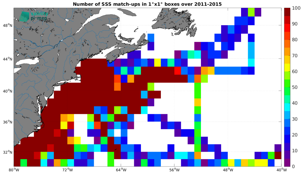
Figure 5: Number of SSS match-ups between TSG (SAMOS) SSS and the Aquarius SSS L4 OI v5 - Weekly (IPRC) SSS product for the Gulf Stream Pi-MEP region over 1^\circ \times 1^\circ boxes and for the full satellite product period.
