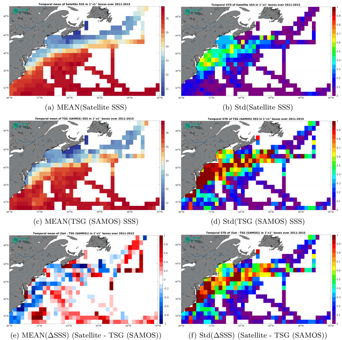
Figure 7: Temporal mean (left) and Std (right) of SSS from Aquarius SSS L4 OI v5 - Weekly (IPRC) (top), TSG (SAMOS) (middle), and of \Delta SSS (Satellite - TSG (SAMOS)). Only match-up pairs are used to generate these maps.
