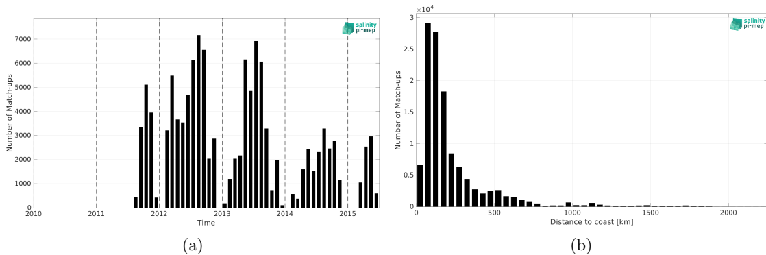
Figure 2: Number of match-ups between TSG (SAMOS) and Aquarius SSS L4 OI v5 - Weekly (IPRC) SSS as a function of time (a) and as function of the distance to coast (b) over the Gulf Stream Pi-MEP region and for the full satellite product period.
