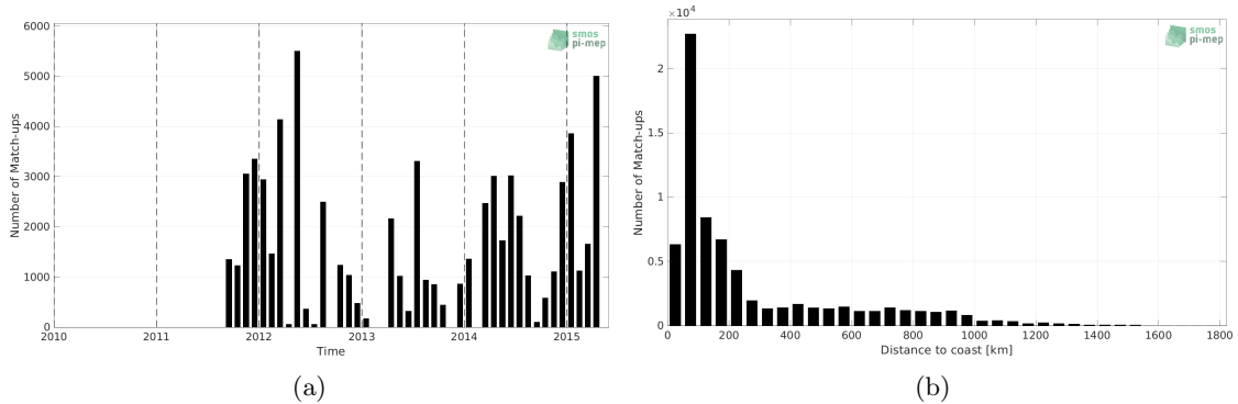
Figure 1: Number of match-ups between TSG (LEGOS-DM) and Aquarius SSS L4 OI v5 - Weekly (IPRC) SSS as a function of time (a) and as function of the distance to coast (b) over the Gulf Stream Pi-MEP region and for the full satellite product period.
