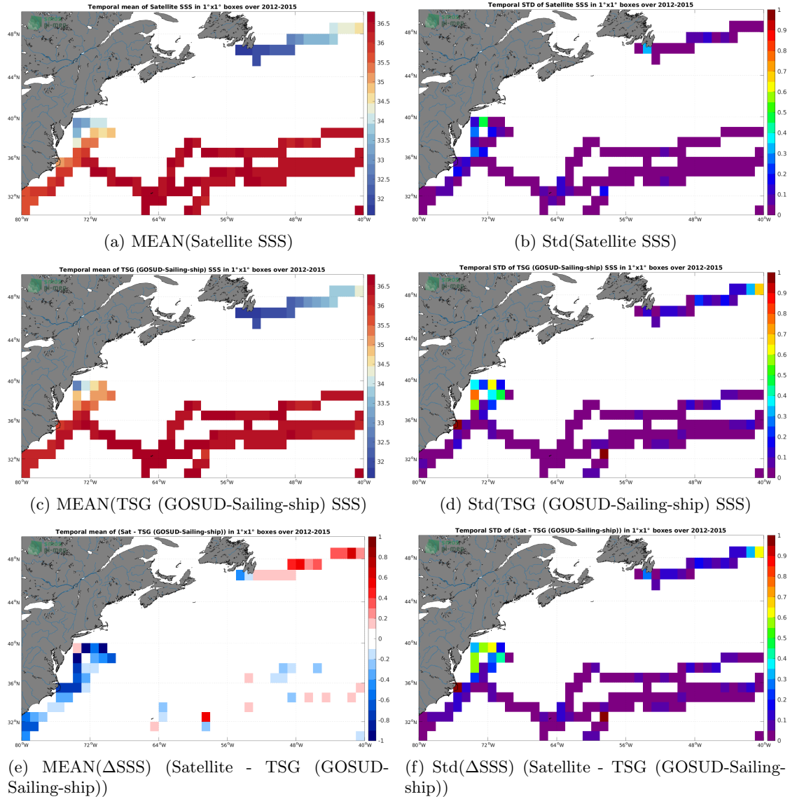
Figure 6: Temporal mean (left) and Std (right) of SSS from Aquarius SSS L4 OI v5 - Weekly (IPRC) (top), TSG (GOSUD-Sailing-ship) (middle), and of \Delta SSS (Satellite - TSG (GOSUD-Sailing-ship)). Only match-up pairs are used to generate these maps.
