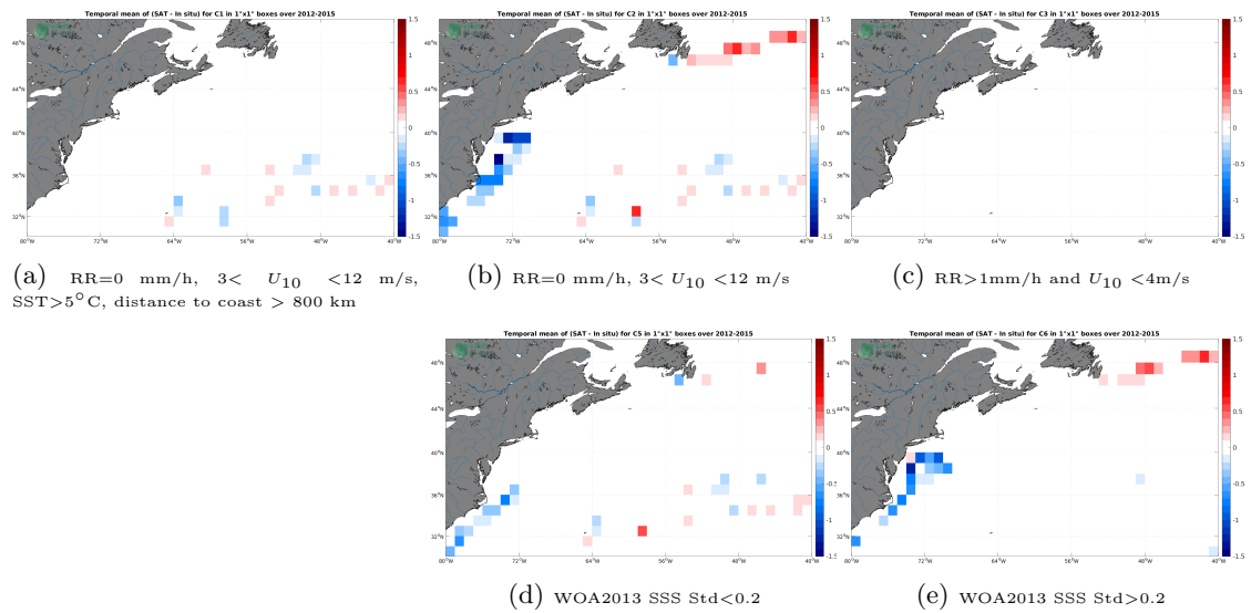
Figure 12: Temporal mean gridded over spatial boxes of size 1^\circ \times 1^\circ of \Delta SSS (Aquarius SSS L4 OI v5 - Weekly (IPRC) - TSG (GOSUD-Sailing-ship)) for 5 different subdatasets corresponding to:RR=0 mm/h, 3 < U_{10} < 12 m/s, SST >5^\circ C, distance to coast > 800 km (a), RR=0 mm/h, 3 < U_{10} < 12 m/s (b), RR >1 mm/h and U_{10} < 4 m/s (c), WOA2013 SSS Std <0.2 (d), WOA2013 SSS Std >0.2 (e).
