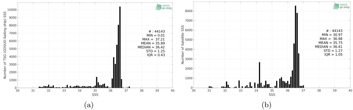
Figure 2: Histograms of SSS from TSG (GOSUD-Sailing-ship) (a) and Aquarius SSS L4 OI v5 - Weekly (IPRC) (b) considering all match-up pairs per bins of 0.1 over the Gulf Stream Pi-MEP region and for the full satellite product period.
