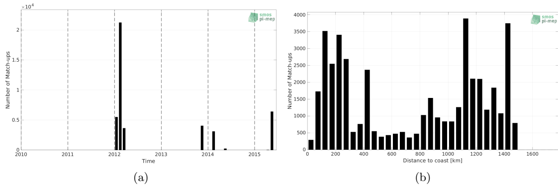
Figure 1: Number of match-ups between TSG (GOSUD-Sailing-ship) and Aquarius SSS L4 OI v5 - Weekly (IPRC) SSS as a function of time (a) and as function of the distance to coast (b) over the Gulf Stream Pi-MEP region and for the full satellite product period.
