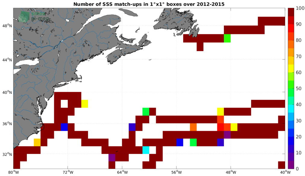
Figure 4: Number of SSS match-ups between TSG (GOSUD-Sailing-ship) SSS and the Aquarius SSS L4 OI v5 - Weekly (IPRC) SSS product for the Gulf Stream Pi-MEP region over 1^{\circ} \times 1^{\circ} boxes and for the full satellite product period.
