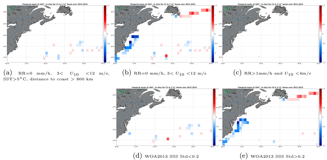
Figure 12: Temporal mean gridded over spatial boxes of size 1°x1° of \Delta SSS (Aquarius SSS L4 OI v5 - Weekly (IPRC) - TSG (GOSUD-Sailing-ship)) for 5 different subdatasets corresponding to:RR=0 mm/h, 3 < U_{10} < 12 m/s, SST > 5^{\circ}C , distance to coast > 800 km (a), RR=0 mm/h, 3 < U_{10} < 12 m/s (b), RR>1mm/h and U_{10} < 4m/s (c), WOA2013 SSS Std<0.2 (d), WOA2013 SSS Std>0.2 (e).
