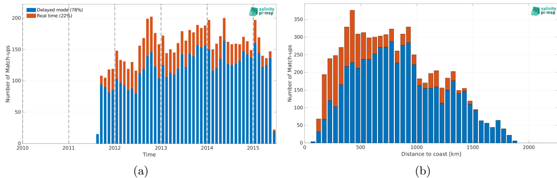
Figure 2: Number of match-ups between Argo and Aquarius SSS L4 OI v5 - Weekly (IPRC) SSS as a function of time (a) and as function of the distance to coast (b) over the Gulf Stream Pi-MEP region and for the full satellite product period.
