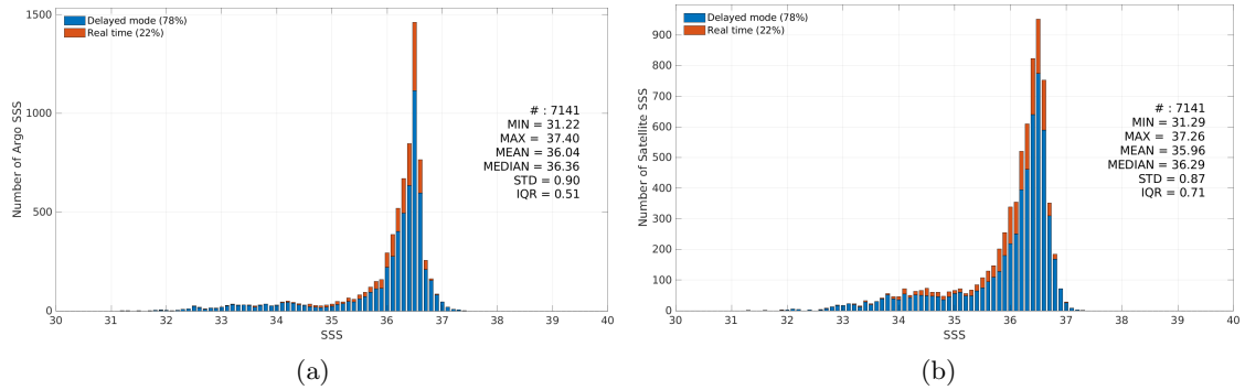
Figure 3: Histograms of SSS from Argo (a) and Aquarius SSS L4 OI v5 - Weekly (IPRC) (b) considering all match-up pairs per bins of 0.1 over the Gulf Stream Pi-MEP region and for the full satellite product period.
