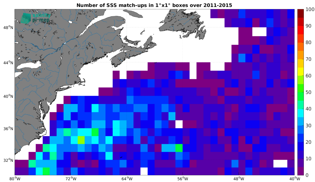
Figure 5: Number of SSS match-ups between Argo SSS and the Aquarius SSS L4 OI v5 - Weekly (IPRC) SSS product for the Gulf Stream Pi-MEP region over 1^\circ \times 1^\circ boxes and for the full satellite product period.
