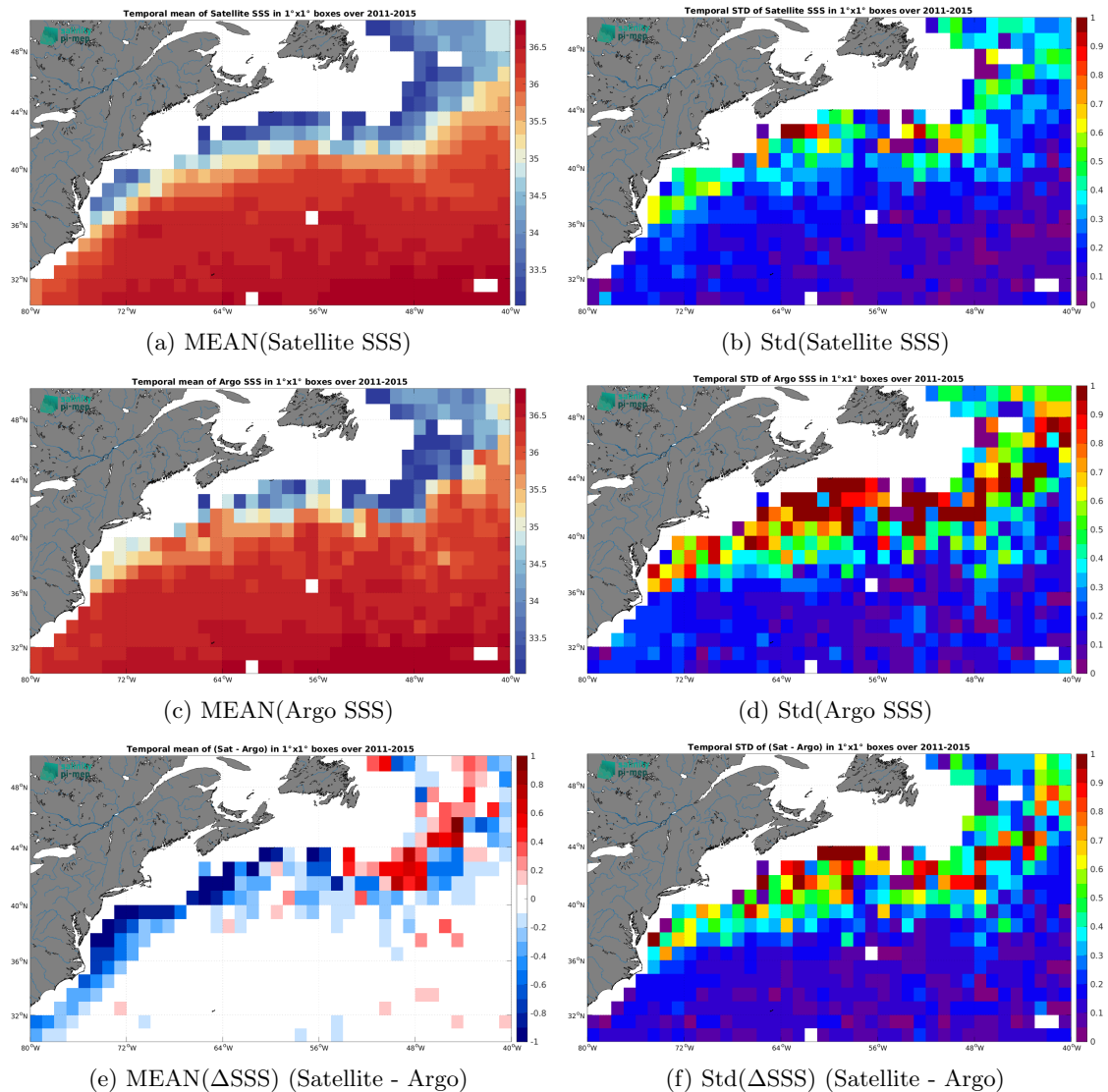
Figure 7: Temporal mean (left) and Std (right) of SSS from Aquarius SSS L4 OI v5 - Weekly (IPRC) (top), Argo (middle), and of \Delta SSS (Satellite - Argo). Only match-up pairs are used to generate these maps.
