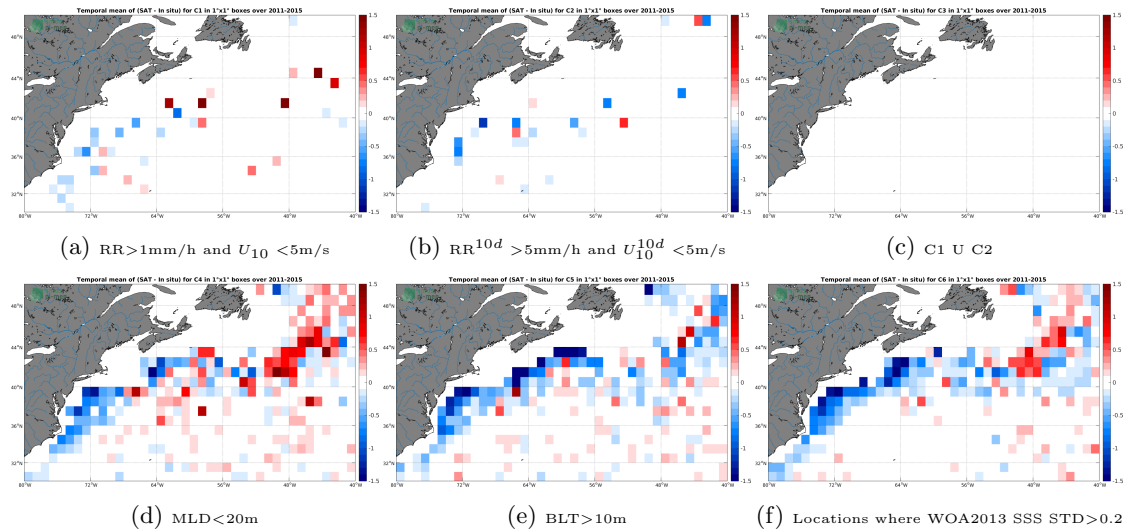
Figure 12: Temporal mean gridded over spatial boxes of size 1^\circ \times 1^\circ of \Delta\text{SSS} (Aquarius-L4-IPRC-V5-WEEKLY - Argo) for 6 different subdatasets corresponding to: RR > 1\text{mm/h} and U_{10} < 5\text{m/s} (a), RR^{10d} > 5\text{mm/h} and U_{10}^{10d} < 5\text{m/s} (b), C1 U C2 (c), MLD < 20\text{m} (d), BLT > 10\text{m} (e), Locations where WOA2013 SSS STD > 0.2 (f).
