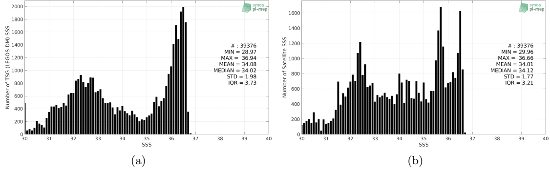
Figure 2: Histograms of SSS from TSG (LEGOS-DM) (a) and Aquarius SSS L4 OI v5 - Monthly (IPRC) (b) considering all match-up pairs per bins of 0.1 over the Gulf Stream Pi-MEP region and for the full satellite product period.
