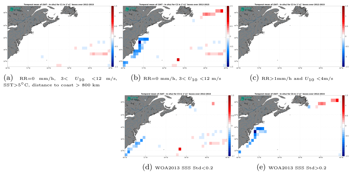
Figure 14: Temporal mean gridded over spatial boxes of size 1^\circ \times 1^\circ of \Delta SSS (Aquarius SSS L4 OI v5 - Monthly (IPRC) - TSG (GOSUD-Sailing-ship)) for 5 different subdatasets corresponding to:RR=0 mm/h, 3 < U_{10} < 12 m/s, SST >5^\circ C, distance to coast > 800 km (a), RR=0 mm/h, 3 < U_{10} < 12 m/s (b), RR >1 mm/h and U_{10} < 4 m/s (c), WOA2013 SSS Std <0.2 (d), WOA2013 SSS Std >0.2 (e).
