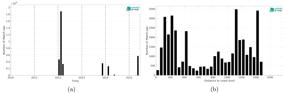
Figure 2: Number of match-ups between TSG (GOSUD-Sailing-ship) and Aquarius SSS L4 OI v5 - Monthly (IPRC) SSS as a function of time (a) and as function of the distance to coast (b) over the Gulf Stream Pi-MEP region and for the full satellite product period.
