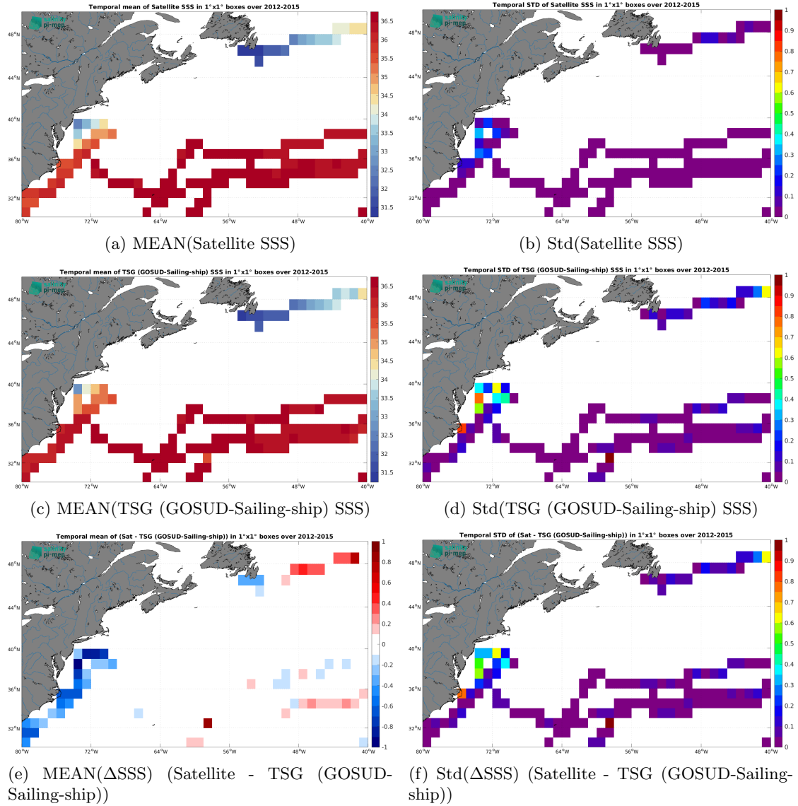
Figure 7: Temporal mean (left) and Std (right) of SSS from Aquarius SSS L4 OI v5 - Monthly (IPRC) (top), TSG (GOSUD-Sailing-ship) (middle), and of \Delta SSS (Satellite - TSG (GOSUD-Sailing-ship)). Only match-up pairs are used to generate these maps.
