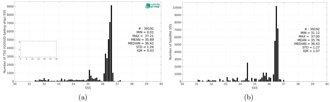
Figure 3: Histograms of SSS from TSG (GOSUD-Sailing-ship) (a) and Aquarius SSS L4 OI v5 - Monthly (IPRC) (b) considering all match-up pairs per bins of 0.1 over the Gulf Stream Pi-MEP region and for the full satellite product period.
