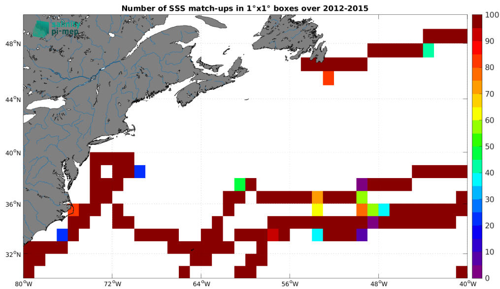
Figure 5: Number of SSS match-ups between TSG (GOSUD-Sailing-ship) SSS and the Aquarius SSS L4 OI v5 - Monthly (IPRC) SSS product for the Gulf Stream Pi-MEP region over 1^\circ \times 1^\circ boxes and for the full satellite product period.
