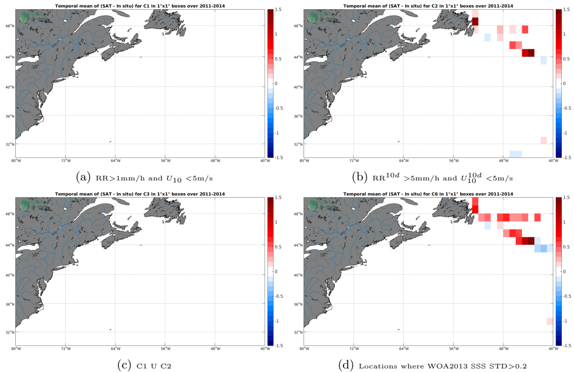
Figure 12: Temporal mean gridded over spatial boxes of size 1^\circ \times 1^\circ of \Delta SSS (Aquarius-L4-IPRC-V5-MONTHLY - TSG-GOSUD-Research-vessel) for 4 different subdatasets corresponding to: RR > 1mm/h and U_{10} < 5\text{m/s} (a), RR^{10d} > 5\text{mm/h} and U_{10}^{10d} < 5\text{m/s} (b), C1 U C2 (c), Locations where WOA2013 SSS STD > 0.2 (d).
