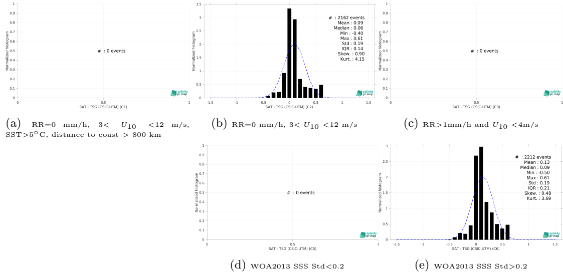
Figure 15: Normalized histogram of \Delta SSS (Aquarius SSS L4 OI v5 - Monthly (IPRC) - TSG (CSIC-UTM)) for 5 different subdatasets corresponding to: RR=0 mm/h, 3 < U_{10} < 12 m/s, SST >5^{\circ} C, distance to coast > 800 km (a), RR=0 mm/h, 3 < U_{10} < 12 m/s (b), RR >1 mm/h and U_{10} < 4 m/s (c), WOA2013 SSS Std <0.2 (d), WOA2013 SSS Std >0.2 (e).
