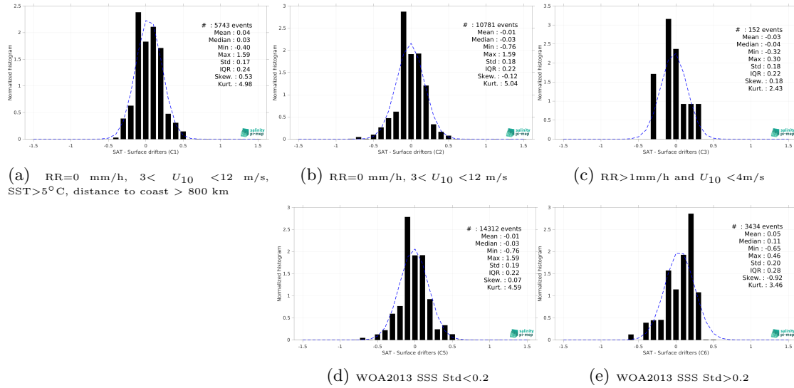
Figure 12: Normalized histogram of \Delta\text{SSS} (Aquarius SSS L4 OI v5 - Monthly (IPRC) - Surface drifters) for 5 different subdatasets corresponding to: RR=0 mm/h, 3 < U_{10} < 12 m/s, SST>5°C, distance to coast > 800 km (a), RR=0 mm/h, 3 < U_{10} < 12 m/s (b), RR>1mm/h and U_{10} < 4 m/s (c), WOA2013 SSS Std<0.2 (d), WOA2013 SSS Std>0.2 (e).
