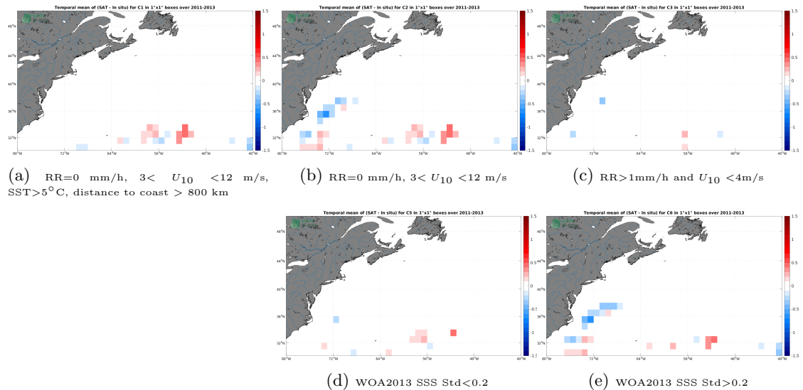
Figure 11: Temporal mean gridded over spatial boxes of size 1^{\circ}\times 1^{\circ} of \Delta\text{SSS} (Aquarius SSS L4 OI v5 - Monthly (IPRC) - Surface drifters) for 5 different subdatasets corresponding to:RR=0 mm/h, 3 < U_{10} < 12 m/s, SST >5^{\circ}\text{C} , distance to coast > 800 km (a), RR=0 mm/h, 3 < U_{10} < 12 m/s (b), RR >1 mm/h and U_{10} < 4 m/s (c), WOA2013 SSS Std <0.2 (d), WOA2013 SSS Std >0.2 (e).
