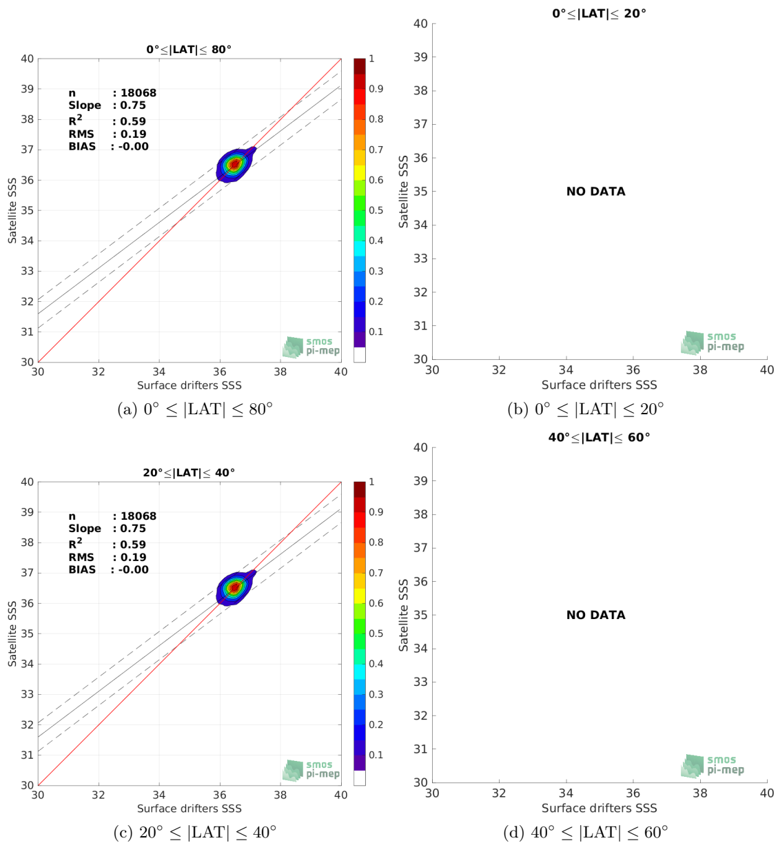
Figure 8: Contour maps of the concentration of Aquarius SSS L4 OI v5 - Monthly (IPRC) SSS (y-axis) versus Surface drifters SSS (x-axis) at match-up pairs for different latitude bands. For each plot, the red line shows x=y . The black thin and dashed lines indicate a linear fit through the data cloud and the \pm 95\% confidence levels, respectively. The number match-up pairs n , the slope and R^2 coefficient of the linear fit, the root mean square (RMS) and the mean bias between satellite and in situ data are indicated for each latitude band in each plots.
