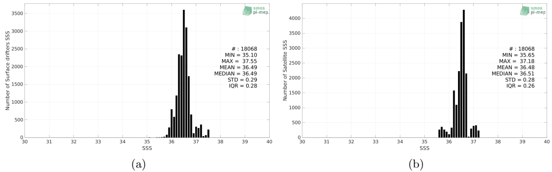
Figure 2: Histograms of SSS from Surface drifters (a) and Aquarius SSS L4 OI v5 - Monthly (IPRC) (b) considering all match-up pairs per bins of 0.1 over the Gulf Stream Pi-MEP region and for the full satellite product period.
