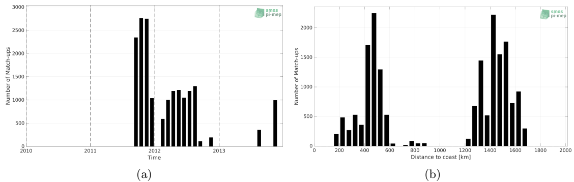
Figure 1: Number of match-ups between Surface drifters and Aquarius SSS L4 OI v5 - Monthly (IPRC) SSS as a function of time (a) and as function of the distance to coast (b) over the Gulf Stream Pi-MEP region and for the full satellite product period.
