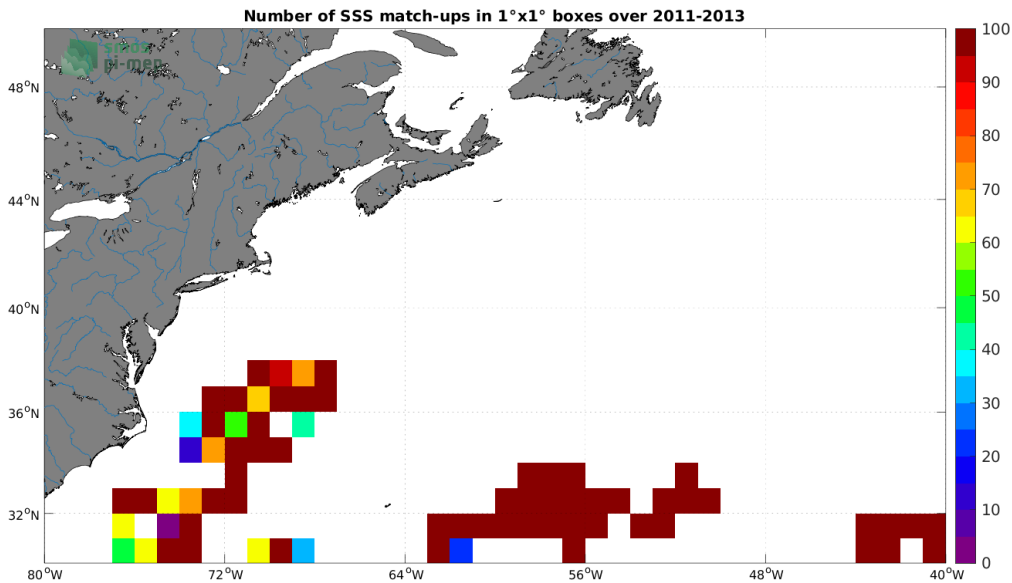
Figure 3: Number of SSS match-ups between Surface drifters SSS and the Aquarius SSS L4 OI v5 - Monthly (IPRC) SSS product for the Gulf Stream Pi-MEP region over 1^\circ \times 1^\circ boxes and for the full satellite product period.
