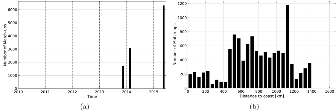
Figure 1: Number of match-ups between TSG-GOSUD-Sailing-ship and Aquarius-L4-IPRC-V4-MONTHLY SSS as a function of time (a) and as function of the distance to coast (b) over the Gulf Stream Pi-MEP region and for the full satellite product period.
