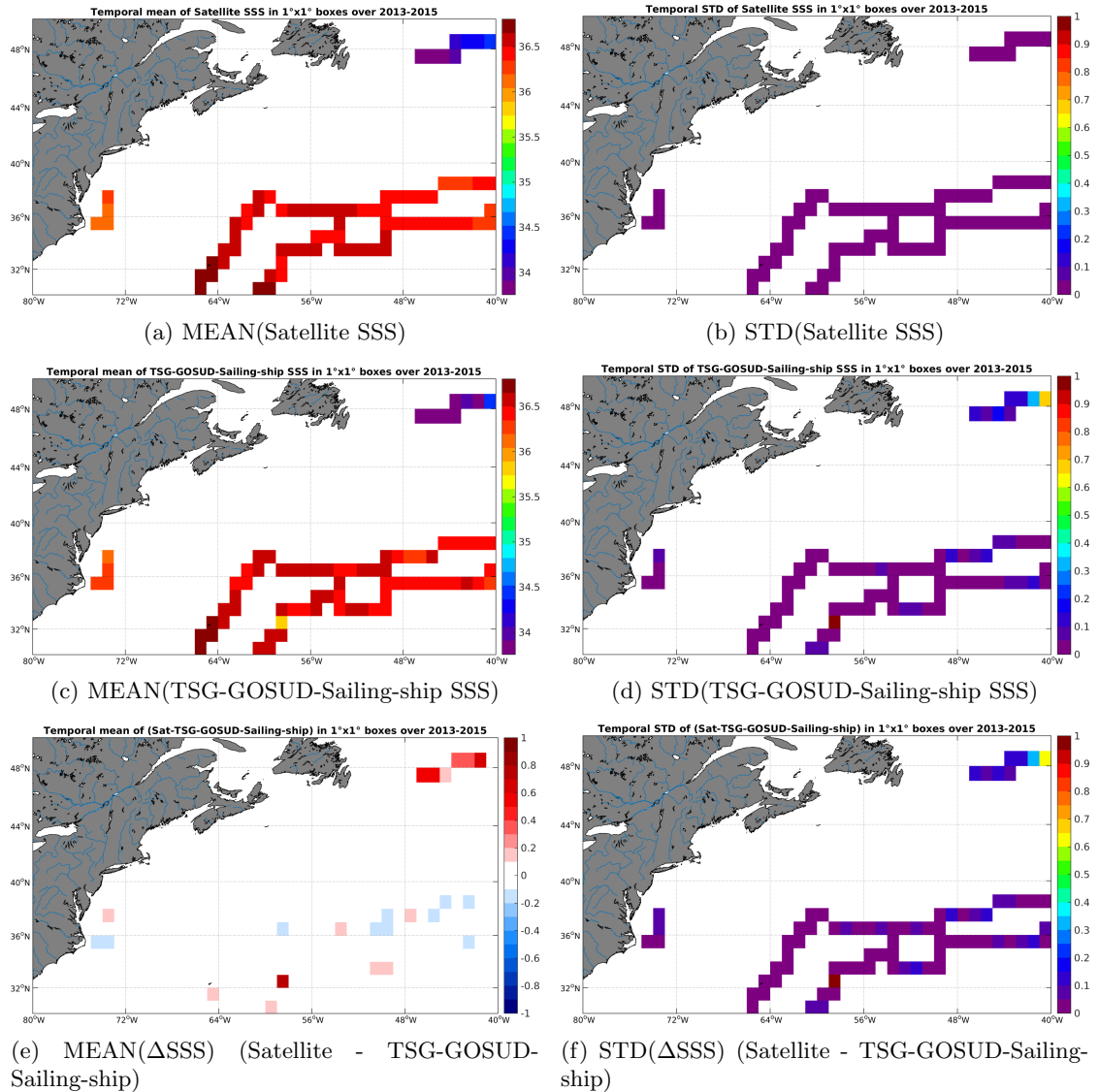
Figure 6: Temporal mean (left) and STD (right) of SSS from Aquarius-L4-IPRC-V4-MONTHLY (top), TSG-GOSUD-Sailing-ship (middle), and of \Delta SSS (Satellite - TSG-GOSUD-Sailing-ship). Only match-up pairs are used to generate these maps.
