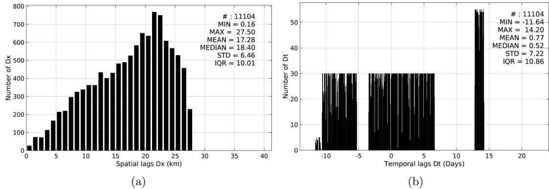
Figure 5: Histograms of the spatial (a) and temporal (b) lags between the time of the TSG-GOSUD-Sailing-ship measurements and the date of the corresponding Aquarius-L4-IPRC-V4-MONTHLY SSS product.
