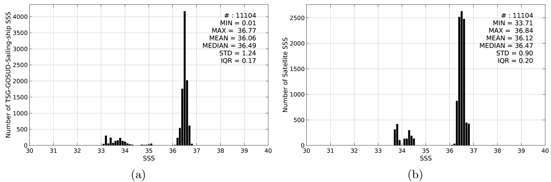
Figure 2: Histograms of SSS from TSG-GOSUD-Sailing-ship (a) and Aquarius-L4-IPRC-V4-MONTHLY (b) considering all match-up pairs per bins of 0.1 over the Gulf Stream Pi-MEP region and for the full satellite product period.
