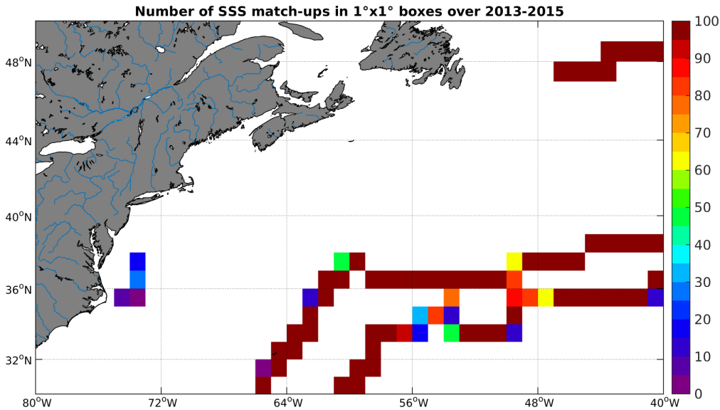
Figure 4: Number of SSS match-ups between TSG-GOSUD-Sailing-ship SSS and the Aquarius-L4-IPRC-V4-MONTHLY SSS product for the Gulf Stream Pi-MEP region over 1^\circ \times 1^\circ boxes and for the full satellite product period.
