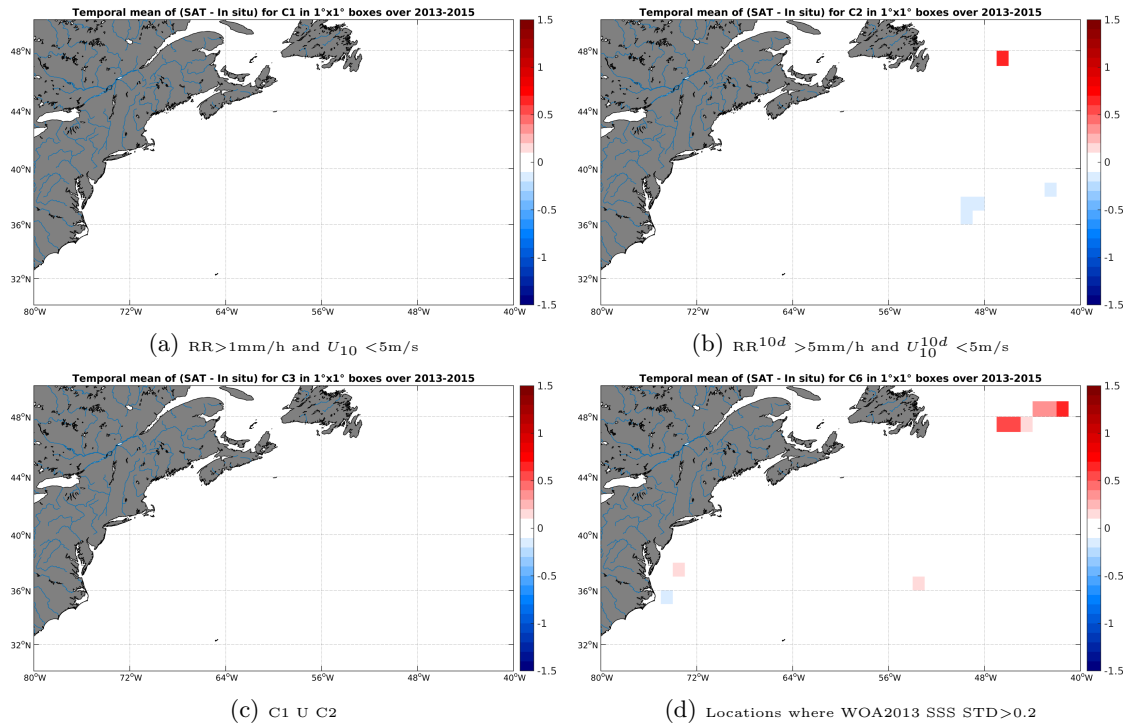
Figure 12: Temporal mean gridded over spatial boxes of size 1°x1° of \Delta SSS (Aquarius-L4-IPRC-V4-MONTHLY - TSG-GOSUD-Sailing-ship) for 4 different subdatasets corresponding to: RR > 1\text{mm/h} and U_{10} < 5\text{m/s} (a), RR^{10d} > 5\text{mm/h} and U_{10}^{10d} < 5\text{m/s} (b), C1 U C2 (c), Locations where WOA2013 SSS STD > 0.2 (d).
