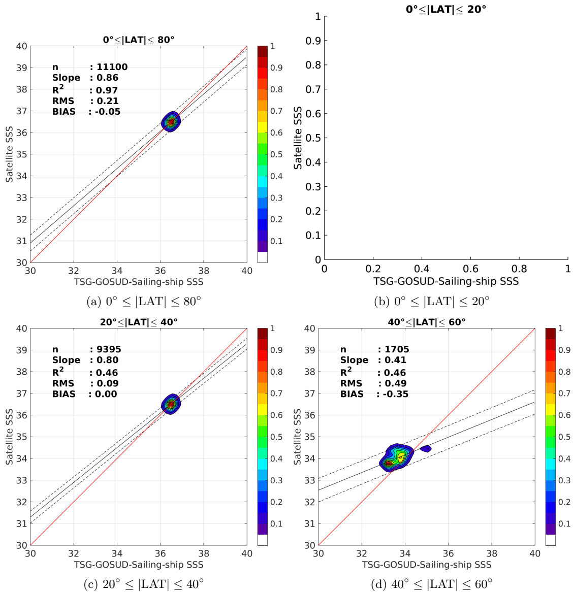
Figure 9: Contour maps of the concentration of Aquarius-L4-IPRC-V4-MONTHLY SSS (y-axis) versus TSG-GOSUD-Sailing-ship SSS (x-axis) at match-up pairs for different latitude bands. For each plot, the red line shows x=y . The black thin and dashed lines indicate a linear fit through the data cloud and the \pm 95\% confidence levels, respectively. The number match-up pairs n , the slope and R^2 coefficient of the linear fit, the root mean square (RMS) and the mean bias between satellite and in situ data are indicated for each latitude band in each plots.
