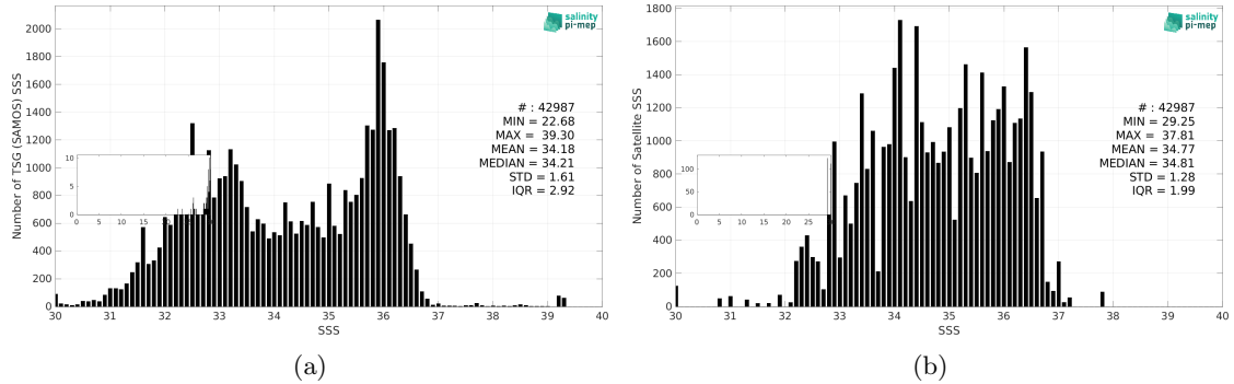
Figure 3: Histograms of SSS from TSG (SAMOS) (a) and Aquarius SSS L3 OR v5 - 7-Day running (NASA-GSFC) (b) considering all match-up pairs per bins of 0.1 over the Gulf Stream Pi-MEP region and for the full satellite product period.
