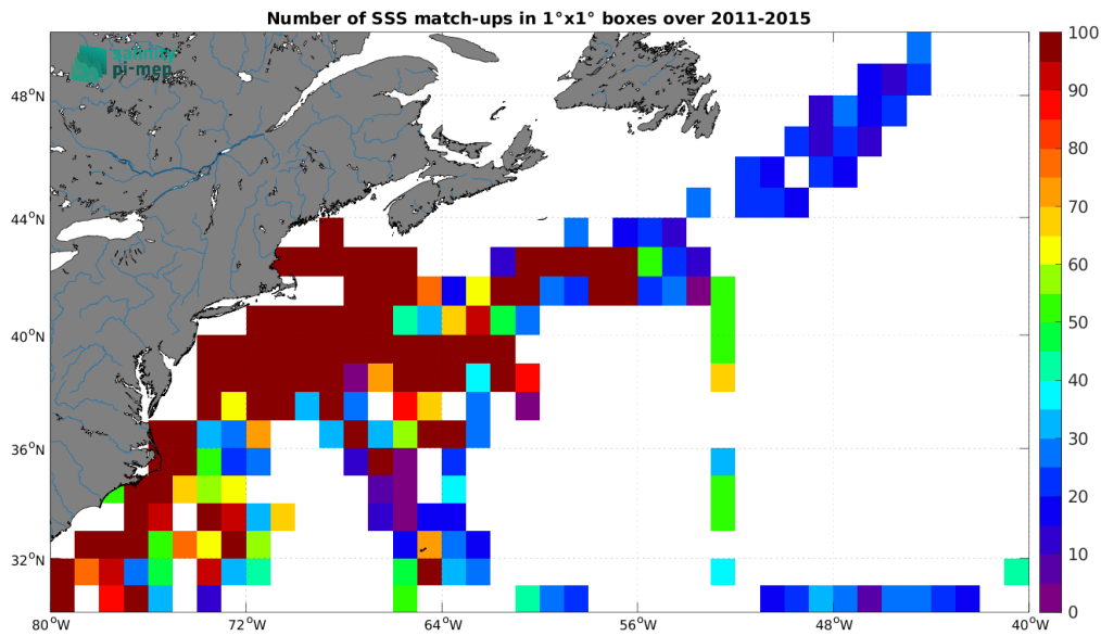
Figure 5: Number of SSS match-ups between TSG (SAMOS) SSS and the Aquarius SSS L3 OR v5 - 7-Day running (NASA-GSFC) SSS product for the Gulf Stream Pi-MEP region over 1^\circ \times 1^\circ boxes and for the full satellite product period.
