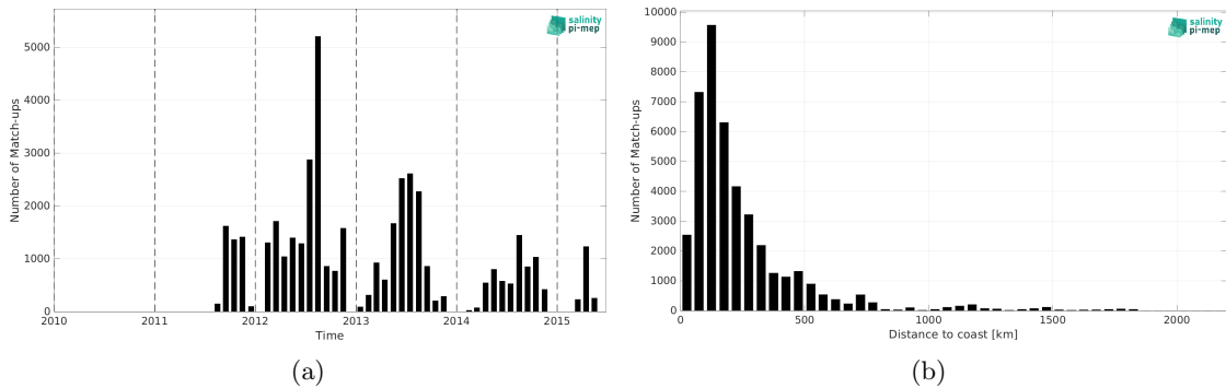
Figure 2: Number of match-ups between TSG (SAMOS) and Aquarius SSS L3 OR v5 - 7-Day running (NASA-GSFC) SSS as a function of time (a) and as function of the distance to coast (b) over the Gulf Stream Pi-MEP region and for the full satellite product period.
