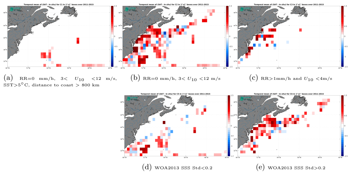
Figure 14: Temporal mean gridded over spatial boxes of size 1^\circ \times 1^\circ of \Delta SSS (Aquarius SSS L3 OR v5 - 7-Day running (NASA-GSFC) - TSG (SAMOS)) for 5 different subdatasets corresponding to:RR=0 mm/h, 3 < U_{10} < 12 m/s, SST >5^\circ\text{C} , distance to coast > 800 km (a), RR=0 mm/h, 3 < U_{10} < 12 m/s (b), RR >1 mm/h and U_{10} < 4 m/s (c), WOA2013 SSS Std <0.2 (d), WOA2013 SSS Std >0.2 (e).
