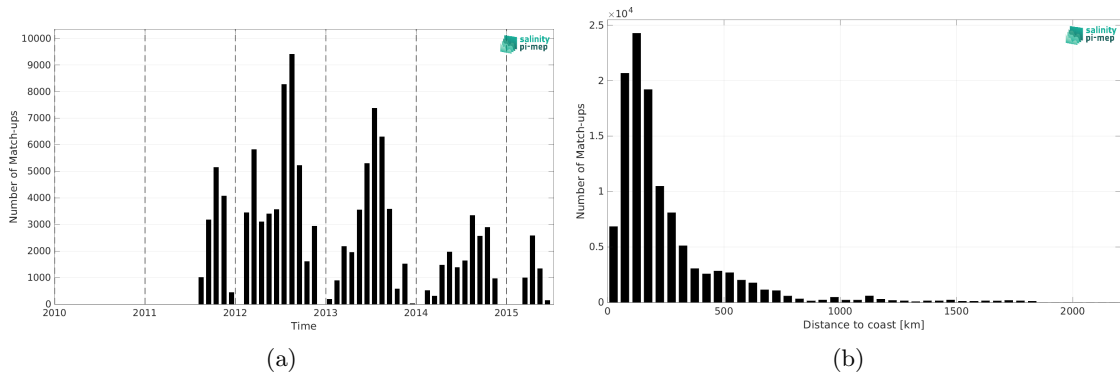
Figure 1: Number of match-ups between TSG (SAMOS) and Aquarius SSS L3 OR v5 - 7-Day running (NASA-GSFC) SSS as a function of time (a) and as function of the distance to coast (b) over the Gulf Stream Pi-MEP region and for the full satellite product period.
