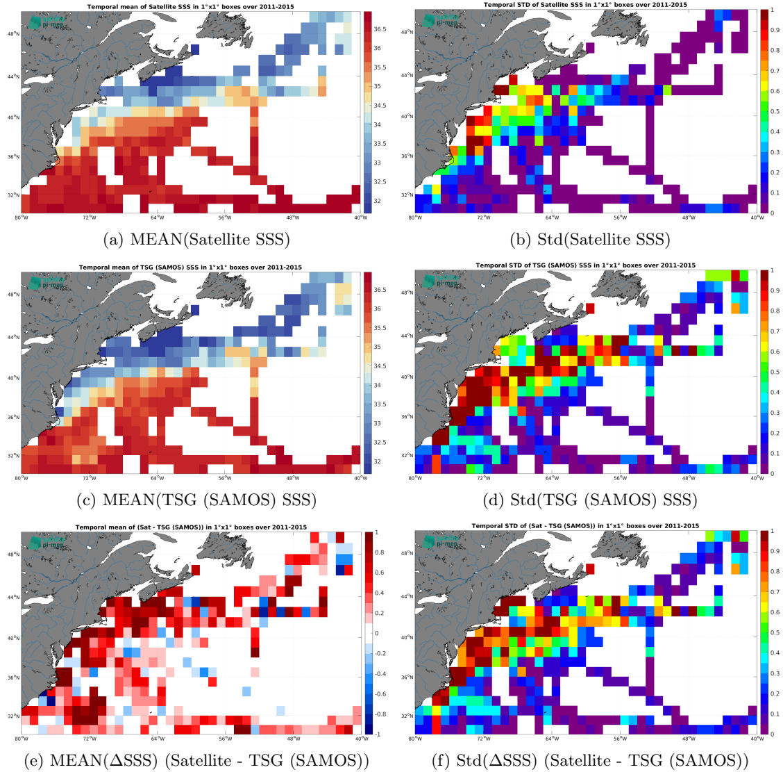
Figure 6: Temporal mean (left) and Std (right) of SSS from Aquarius SSS L3 OR v5 - 7-Day running (NASA-GSFC) (top), TSG (SAMOS) (middle), and of \Delta SSS (Satellite - TSG (SAMOS)). Only match-up pairs are used to generate these maps.
