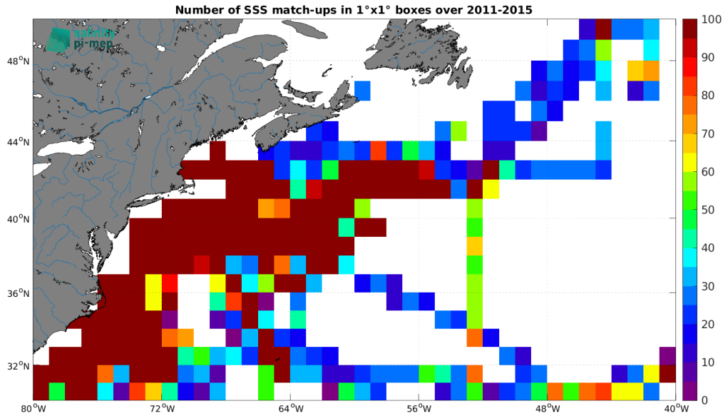
Figure 4: Number of SSS match-ups between TSG (SAMOS) SSS and the Aquarius SSS L3 OR v5 - 7-Day running (NASA-GSFC) SSS product for the Gulf Stream Pi-MEP region over 1^\circ \times 1^\circ boxes and for the full satellite product period.
