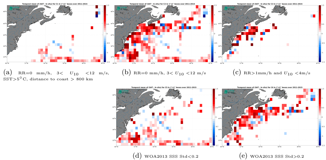
Figure 12: Temporal mean gridded over spatial boxes of size 1^\circ \times 1^\circ of \Delta SSS (Aquarius SSS L3 OR v5 - 7-Day running (NASA-GSFC) - TSG (SAMOS)) for 5 different subdatasets corresponding to:RR=0 mm/h, 3 < U_{10} < 12 m/s, SST >5^\circ C, distance to coast > 800 km (a), RR=0 mm/h, 3 < U_{10} < 12 m/s (b), RR >1 mm/h and U_{10} < 4 m/s (c), WOA2013 SSS Std <0.2 (d), WOA2013 SSS Std >0.2 (e).
