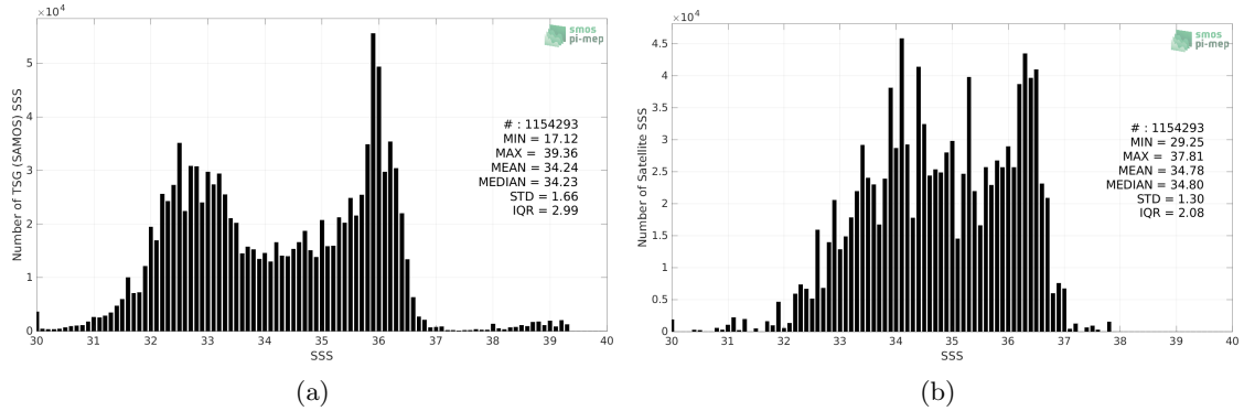
Figure 2: Histograms of SSS from TSG (SAMOS) (a) and Aquarius SSS L3 OR v5 - 7-Day running (NASA-GSFC) (b) considering all match-up pairs per bins of 0.1 over the Gulf Stream Pi-MEP region and for the full satellite product period.
