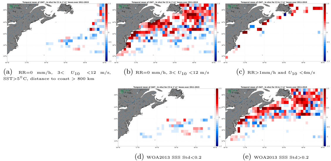
Figure 12: Temporal mean gridded over spatial boxes of size 1^{\circ}\times 1^{\circ} of \Delta\text{SSS} (Aquarius SSS L3 OR v5 - 7-Day running (NASA-GSFC) - TSG (LEGOS-DM)) for 5 different subdatasets corresponding to:RR=0 mm/h, 3 < U_{10} < 12 m/s, SST >5^{\circ}\text{C} , distance to coast > 800 km (a), RR=0 mm/h, 3 < U_{10} < 12 m/s (b), RR >1 mm/h and U_{10} < 4 m/s (c), WOA2013 SSS Std <0.2 (d), WOA2013 SSS Std >0.2 (e).
