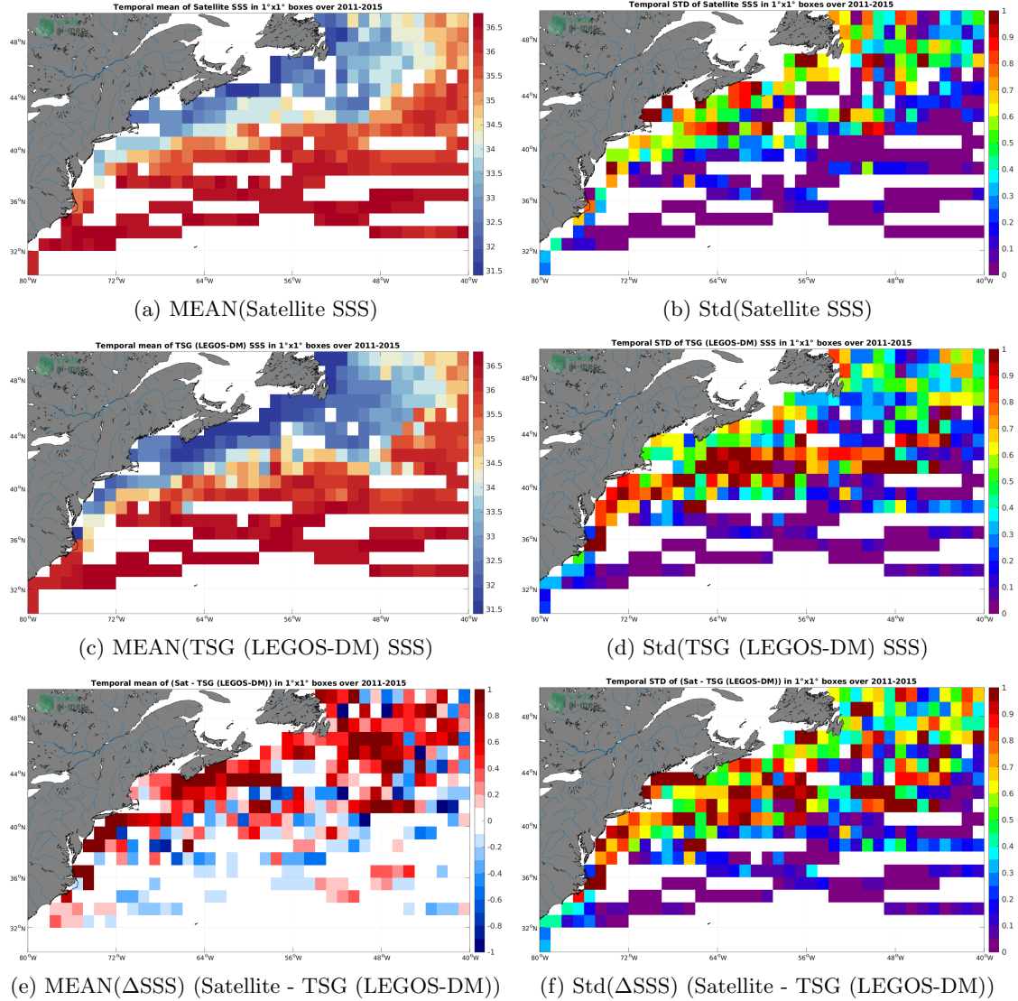
Figure 6: Temporal mean (left) and Std (right) of SSS from Aquarius SSS L3 OR v5 - 7-Day running (NASA-GSFC) (top), TSG (LEGOS-DM) (middle), and of \Delta SSS (Satellite - TSG (LEGOS-DM)). Only match-up pairs are used to generate these maps.
