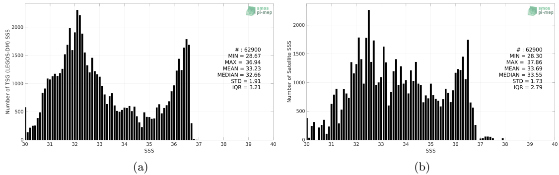
Figure 2: Histograms of SSS from TSG (LEGOS-DM) (a) and Aquarius SSS L3 OR v5 - 7-Day running (NASA-GSFC) (b) considering all match-up pairs per bins of 0.1 over the Gulf Stream Pi-MEP region and for the full satellite product period.
