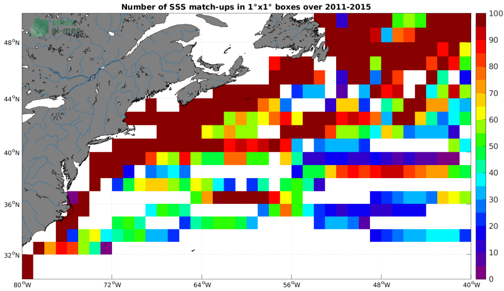
Figure 4: Number of SSS match-ups between TSG (LEGOS-DM) SSS and the Aquarius SSS L3 OR v5 - 7-Day running (NASA-GSFC) SSS product for the Gulf Stream Pi-MEP region over 1^\circ \times 1^\circ boxes and for the full satellite product period.
