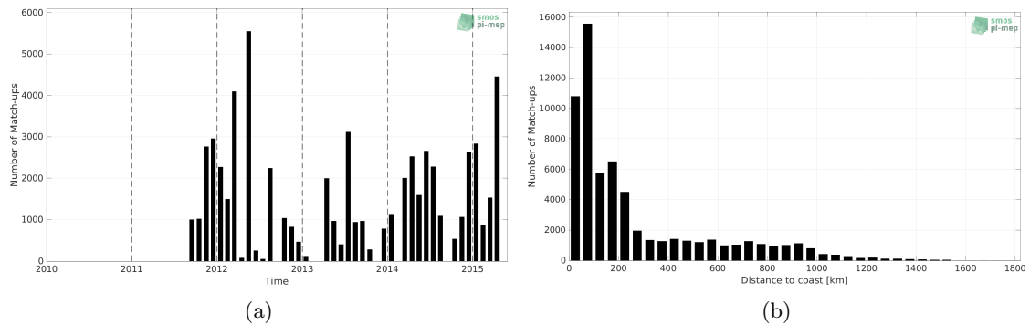
Figure 1: Number of match-ups between TSG (LEGOS-DM) and Aquarius SSS L3 OR v5 - 7-Day running (NASA-GSFC) SSS as a function of time (a) and as function of the distance to coast (b) over the Gulf Stream Pi-MEP region and for the full satellite product period.
