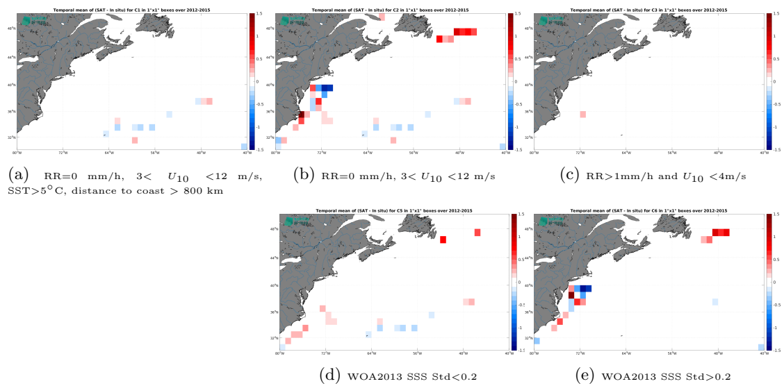
Figure 14: Temporal mean gridded over spatial boxes of size 1^\circ \times 1^\circ of \Delta SSS (Aquarius SSS L3 OR v5 - 7-Day running (NASA-GSFC) - TSG (GOSUD-Sailing-ship)) for 5 different subdatasets corresponding to: RR=0 mm/h, 3 < U_{10} < 12 m/s, SST > 5^\circ C , distance to coast > 800 km (a), RR=0 mm/h, 3 < U_{10} < 12 m/s (b), RR > 1 mm/h and U_{10} < 4 m/s (c), WOA2013 SSS Std < 0.2 (d), WOA2013 SSS Std > 0.2 (e).
