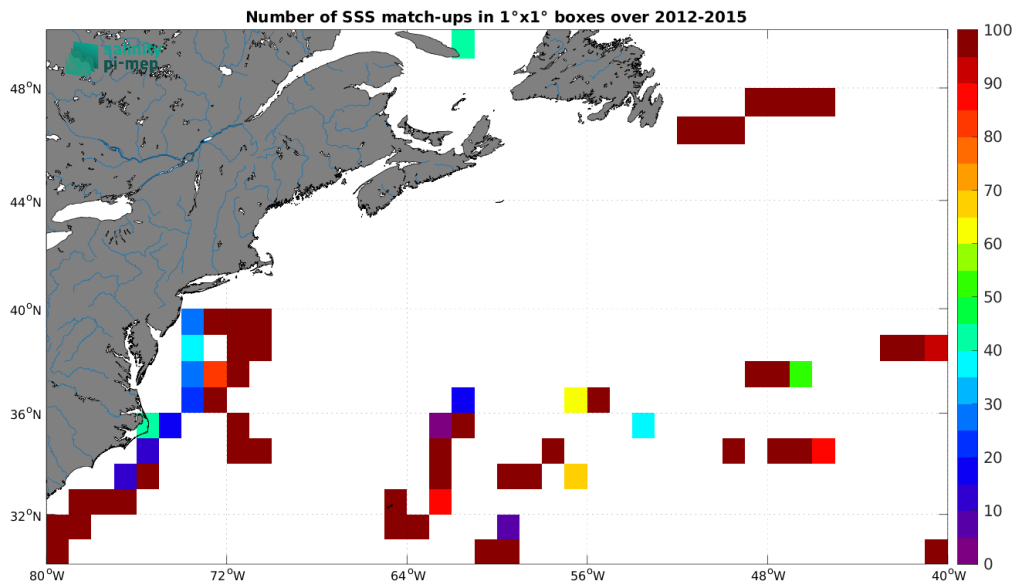
Figure 5: Number of SSS match-ups between TSG (GOSUD-Sailing-ship) SSS and the Aquarius SSS L3 OR v5 - 7-Day running (NASA-GSFC) SSS product for the Gulf Stream Pi-MEP region over 1^\circ \times 1^\circ boxes and for the full satellite product period.
