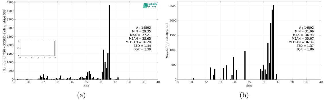
Figure 3: Histograms of SSS from TSG (GOSUD-Sailing-ship) (a) and Aquarius SSS L3 OR v5 - 7-Day running (NASA-GSFC) (b) considering all match-up pairs per bins of 0.1 over the Gulf Stream Pi-MEP region and for the full satellite product period.
