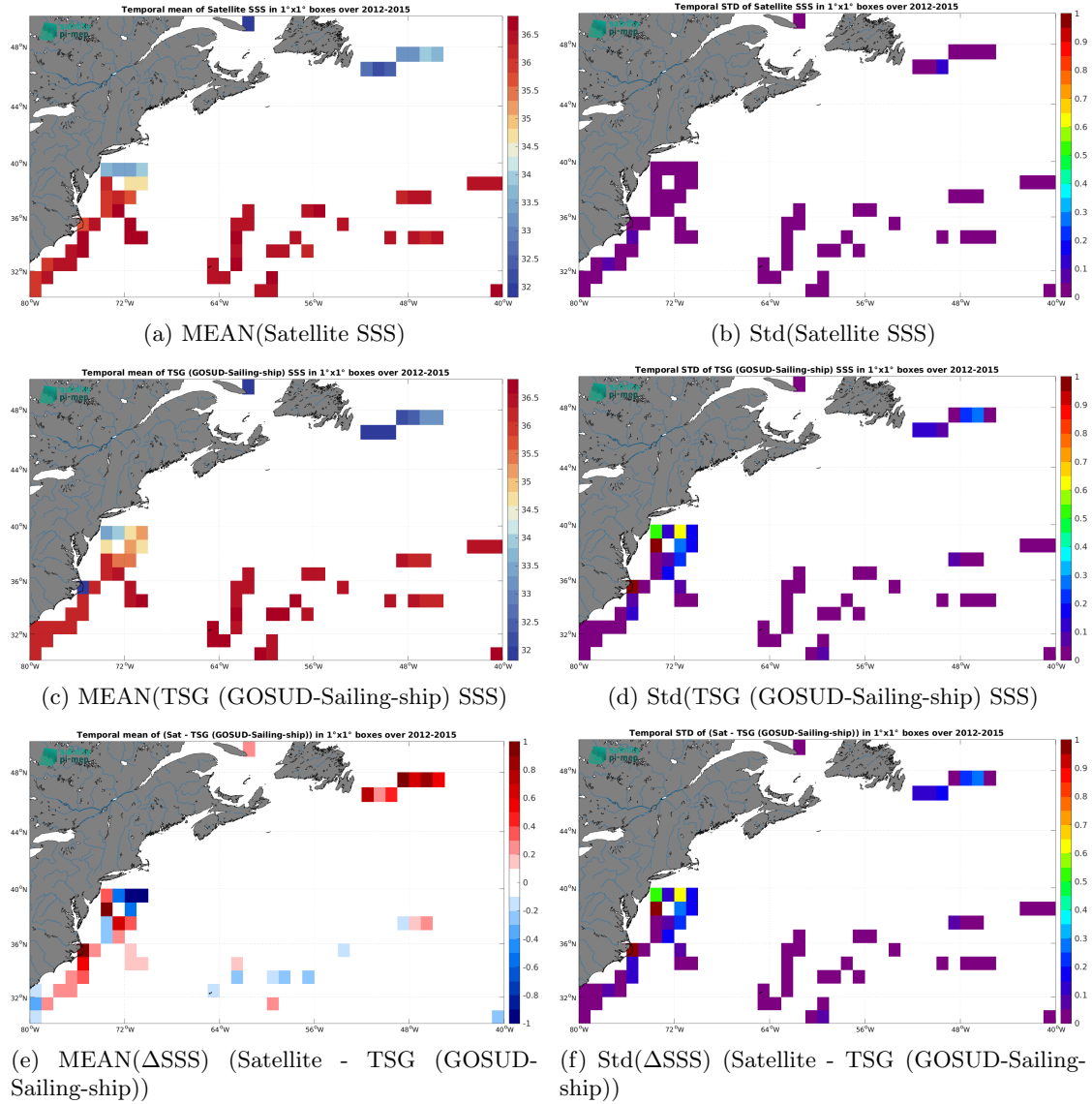
Figure 7: Temporal mean (left) and Std (right) of SSS from Aquarius SSS L3 OR v5 - 7-Day running (NASA-GSFC) (top), TSG (GOSUD-Sailing-ship) (middle), and of \Delta SSS (Satellite - TSG (GOSUD-Sailing-ship)). Only match-up pairs are used to generate these maps.
