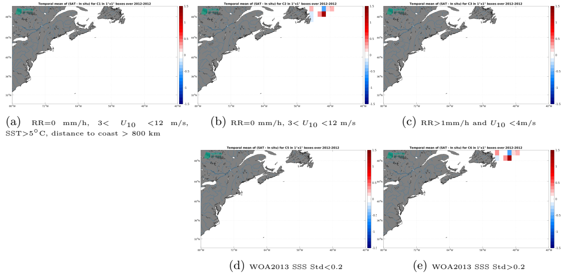
Figure 12: Temporal mean gridded over spatial boxes of size 1^{\circ}\times 1^{\circ} of \Delta\text{SSS} (Aquarius SSS L3 OR v5 - 7-Day running (NASA-GSFC) - TSG (CSIC-UTM)) for 5 different subdatasets corresponding to:RR=0 mm/h, 3 < U_{10} < 12 m/s, SST >5^{\circ}\text{C} , distance to coast > 800 km (a), RR=0 mm/h, 3 < U_{10} < 12 m/s (b), RR >1 mm/h and U_{10} < 4 m/s (c), WOA2013 SSS Std <0.2 (d), WOA2013 SSS Std >0.2 (e).
