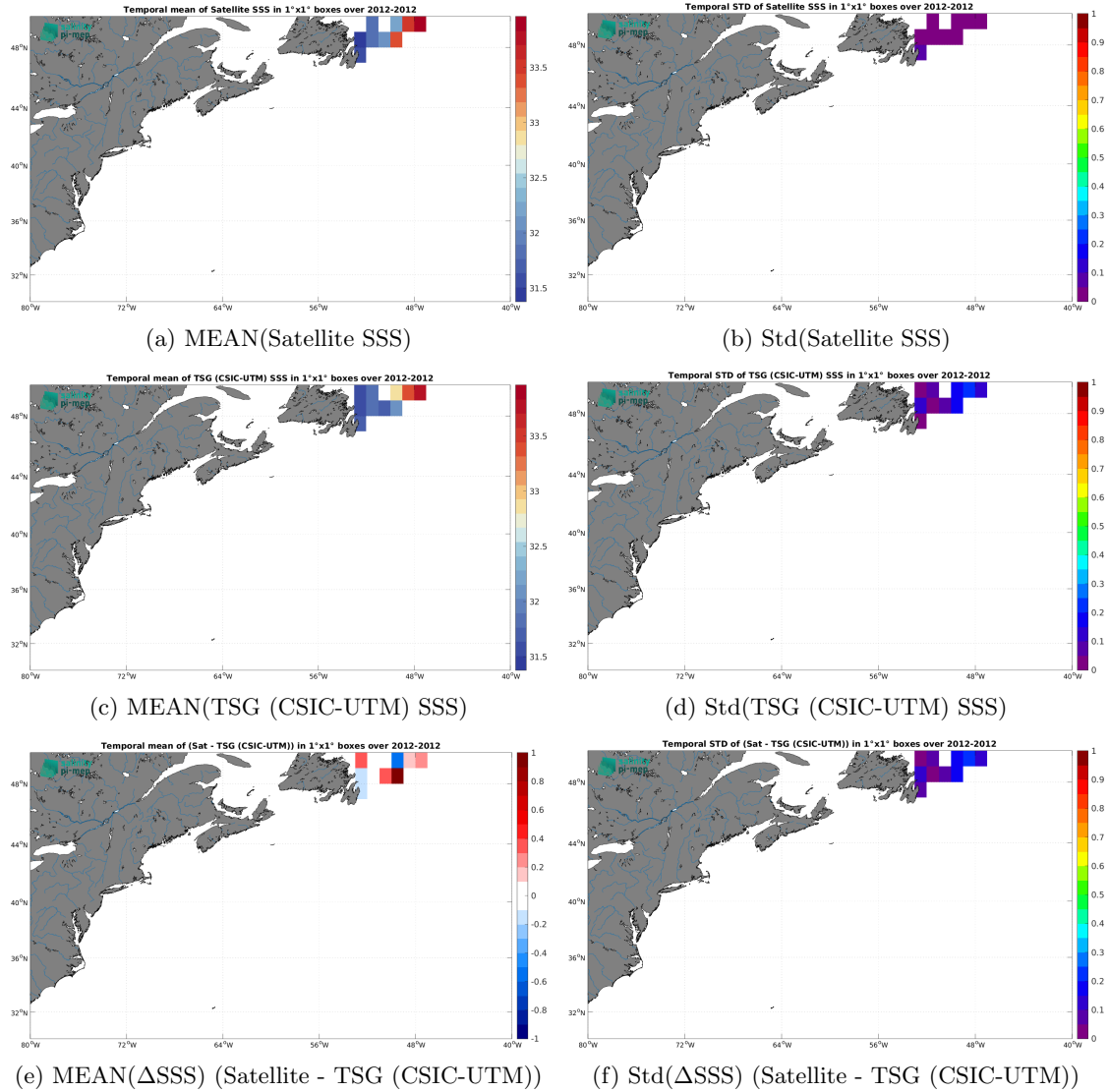
Figure 6: Temporal mean (left) and Std (right) of SSS from Aquarius SSS L3 OR v5 - 7-Day running (NASA-GSFC) (top), TSG (CSIC-UTM) (middle), and of \Delta SSS (Satellite - TSG (CSIC-UTM)). Only match-up pairs are used to generate these maps.
