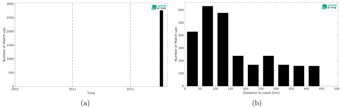
Figure 1: Number of match-ups between TSG (CSIC-UTM) and Aquarius SSS L3 OR v5 - 7-Day running (NASA-GSFC) SSS as a function of time (a) and as function of the distance to coast (b) over the Gulf Stream Pi-MEP region and for the full satellite product period.
