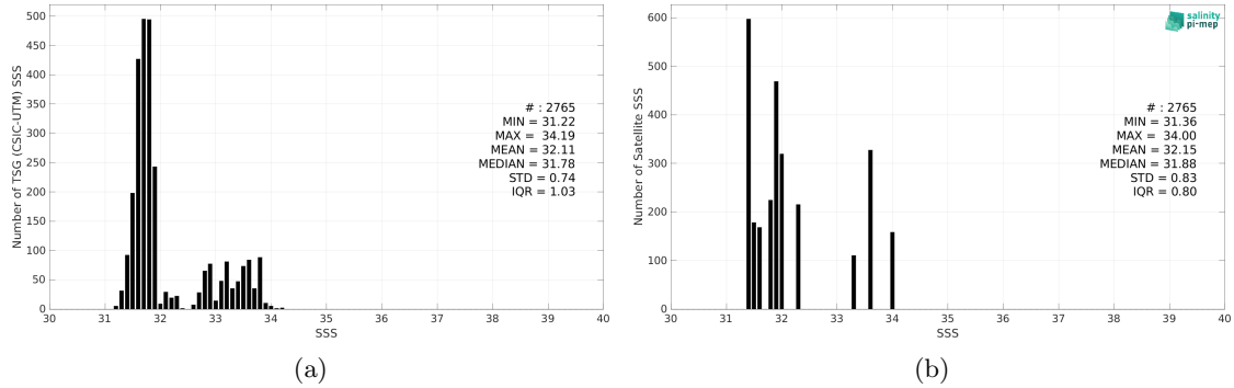
Figure 2: Histograms of SSS from TSG (CSIC-UTM) (a) and Aquarius SSS L3 OR v5 - 7-Day running (NASA-GSFC) (b) considering all match-up pairs per bins of 0.1 over the Gulf Stream Pi-MEP region and for the full satellite product period.
