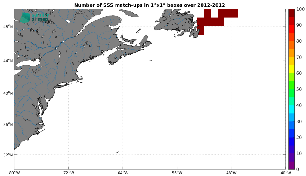
Figure 4: Number of SSS match-ups between TSG (CSIC-UTM) SSS and the Aquarius SSS L3 OR v5 - 7-Day running (NASA-GSFC) SSS product for the Gulf Stream Pi-MEP region over 1^\circ \times 1^\circ boxes and for the full satellite product period.
