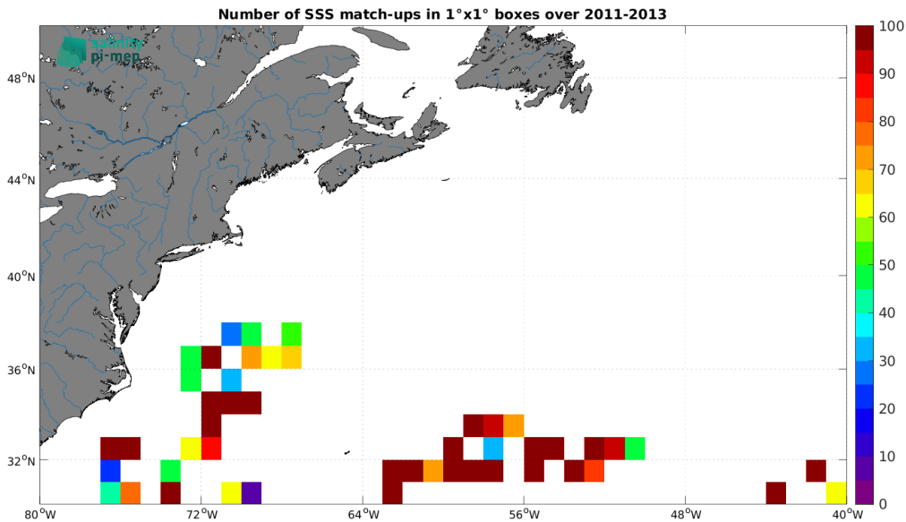
Figure 4: Number of SSS match-ups between Surface drifters SSS and the Aquarius SSS L3 OR v5 - 7-Day running (NASA-GSFC) SSS product for the Gulf Stream Pi-MEP region over 1^\circ \times 1^\circ boxes and for the full satellite product period.
