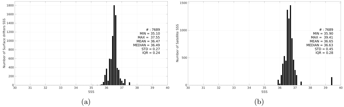
Figure 3: Histograms of SSS from Surface drifters (a) and Aquarius SSS L3 OR v5 - 7-Day running (NASA-GSFC) (b) considering all match-up pairs per bins of 0.1 over the Gulf Stream Pi-MEP region and for the full satellite product period.
