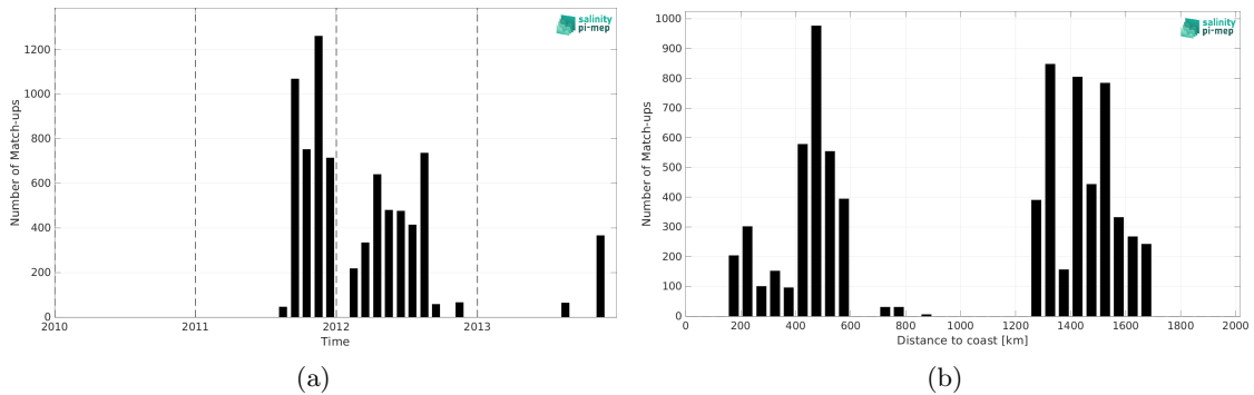
Figure 2: Number of match-ups between Surface drifters and Aquarius SSS L3 OR v5 - 7-Day running (NASA-GSFC) SSS as a function of time (a) and as function of the distance to coast (b) over the Gulf Stream Pi-MEP region and for the full satellite product period.
