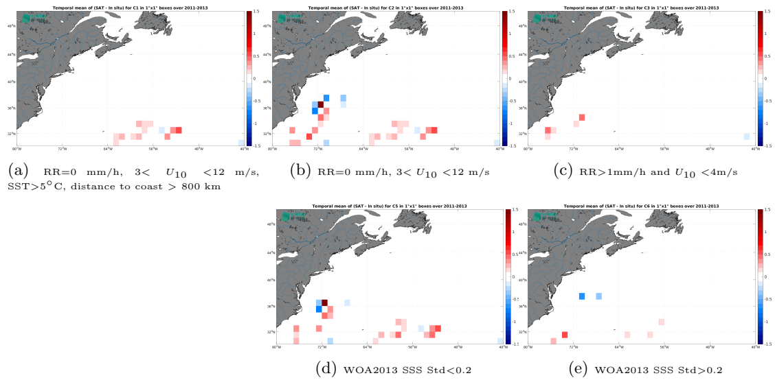
Figure 13: Temporal mean gridded over spatial boxes of size 1^\circ \times 1^\circ of \Delta SSS (Aquarius SSS L3 OR v5 - 7-Day running (NASA-GSFC) - Surface drifters) for 5 different subdatasets corresponding to: RR=0 mm/h, 3 < U_{10} < 12 m/s, SST > 5^\circ C , distance to coast > 800 km (a), RR=0 mm/h, 3 < U_{10} < 12 m/s (b), RR > 1 mm/h and U_{10} < 4 m/s (c), WOA2013 SSS Std < 0.2 (d), WOA2013 SSS Std > 0.2 (e).
