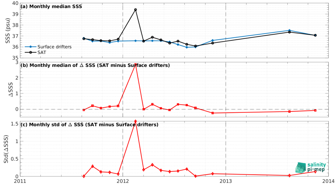
Figure 7: Time series of the monthly median SSS (top), median of \Delta\text{SSS} (Satellite - Surface drifters) and Std of \Delta\text{SSS} (Satellite - Surface drifters) over the Gulf Stream Pi-MEP region considering all match-ups collected by the Pi-MEP.
