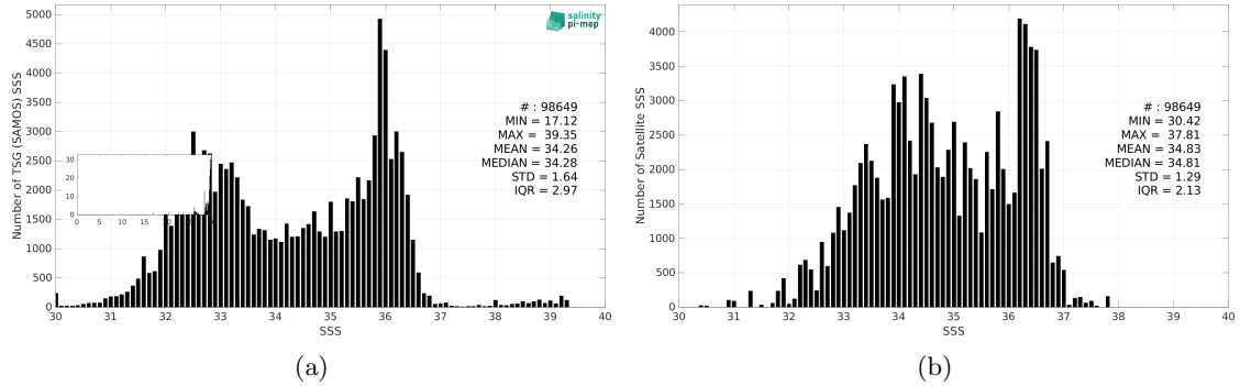
Figure 3: Histograms of SSS from TSG (SAMOS) (a) and Aquarius SSS L3 OR v5 - 7-Day running - Rain mask (NASA-GSFC) (b) considering all match-up pairs per bins of 0.1 over the Gulf Stream Pi-MEP region and for the full satellite product period.
