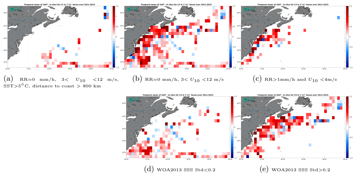
Figure 14: Temporal mean gridded over spatial boxes of size 1^\circ \times 1^\circ of \Delta SSS (Aquarius SSS L3 OR v5 - 7-Day running - Rain mask (NASA-GSFC) - TSG (SAMOS)) for 5 different subdatasets corresponding to:RR=0 mm/h, 3 < U_{10} < 12 m/s, SST >5^\circ C, distance to coast > 800 km (a), RR=0 mm/h, 3 < U_{10} < 12 m/s (b), RR >1 mm/h and U_{10} < 4 m/s (c), WOA2013 SSS Std <0.2 (d), WOA2013 SSS Std >0.2 (e).
