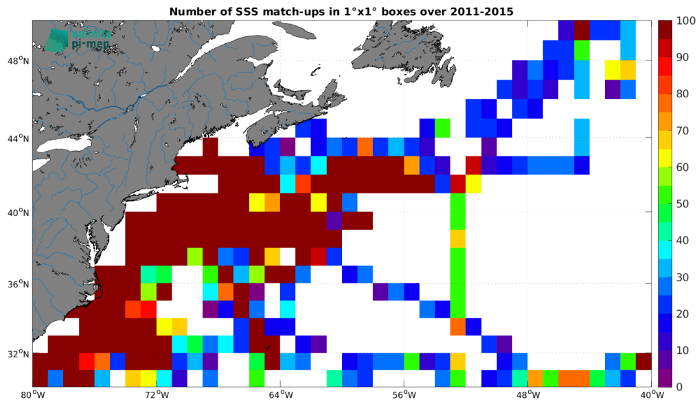
Figure 5: Number of SSS match-ups between TSG (SAMOS) SSS and the Aquarius SSS L3 OR v5 - 7-Day running - Rain mask (NASA-GSFC) SSS product for the Gulf Stream Pi-MEP region over 1^\circ \times 1^\circ boxes and for the full satellite product period.
