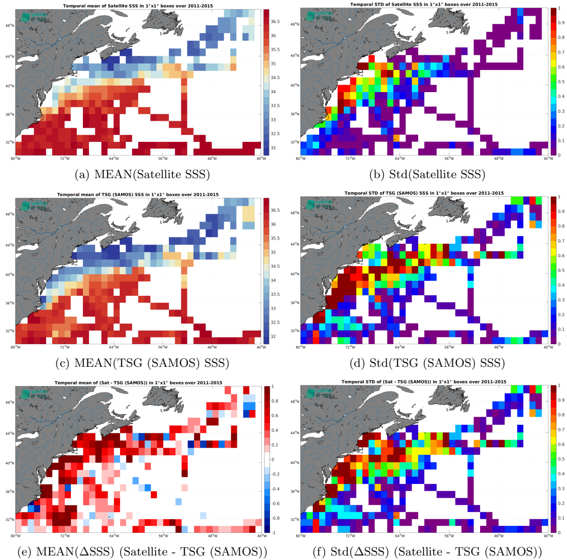
Figure 7: Temporal mean (left) and Std (right) of SSS from Aquarius SSS L3 OR v5 - 7-Day running - Rain mask (NASA-GSFC) (top), TSG (SAMOS) (middle), and of \Delta SSS (Satellite - TSG (SAMOS)). Only match-up pairs are used to generate these maps.
