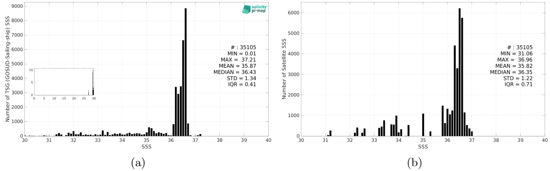
Figure 3: Histograms of SSS from TSG (GOSUD-Sailing-ship) (a) and Aquarius SSS L3 OR v5 - 7-Day running - Rain mask (NASA-GSFC) (b) considering all match-up pairs per bins of 0.1 over the Gulf Stream Pi-MEP region and for the full satellite product period.
