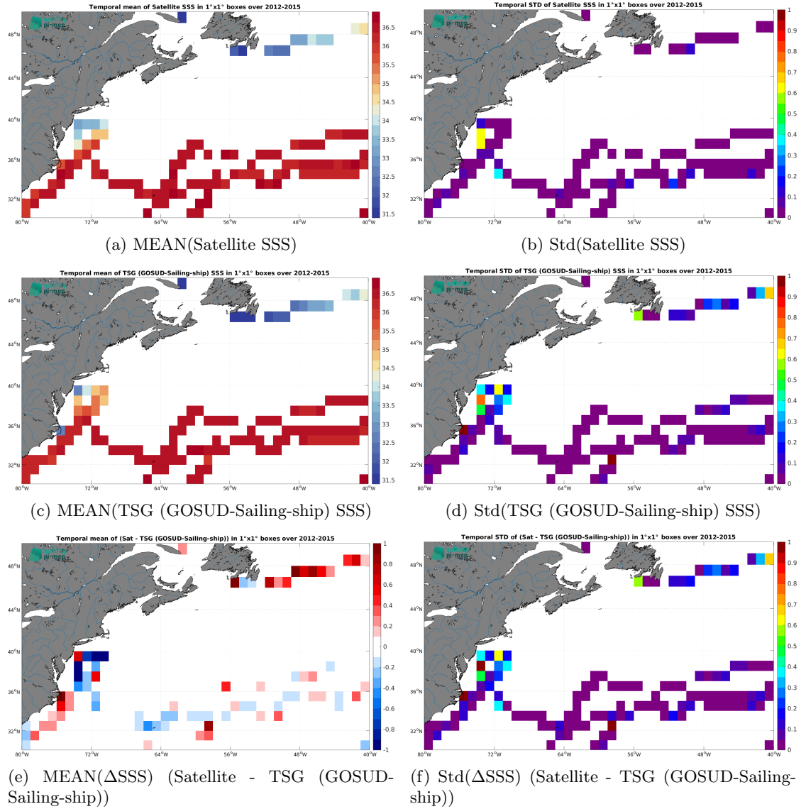
Figure 7: Temporal mean (left) and Std (right) of SSS from Aquarius SSS L3 OR v5 - 7-Day running - Rain mask (NASA-GSFC) (top), TSG (GOSUD-Sailing-ship) (middle), and of \Delta SSS (Satellite - TSG (GOSUD-Sailing-ship)). Only match-up pairs are used to generate these maps.
