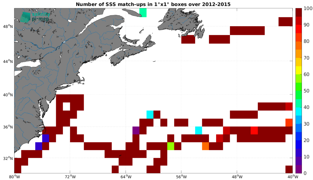
Figure 5: Number of SSS match-ups between TSG (GOSUD-Sailing-ship) SSS and the Aquarius SSS L3 OR v5 - 7-Day running - Rain mask (NASA-GSFC) SSS product for the Gulf Stream Pi-MEP region over 1^\circ \times 1^\circ boxes and for the full satellite product period.
