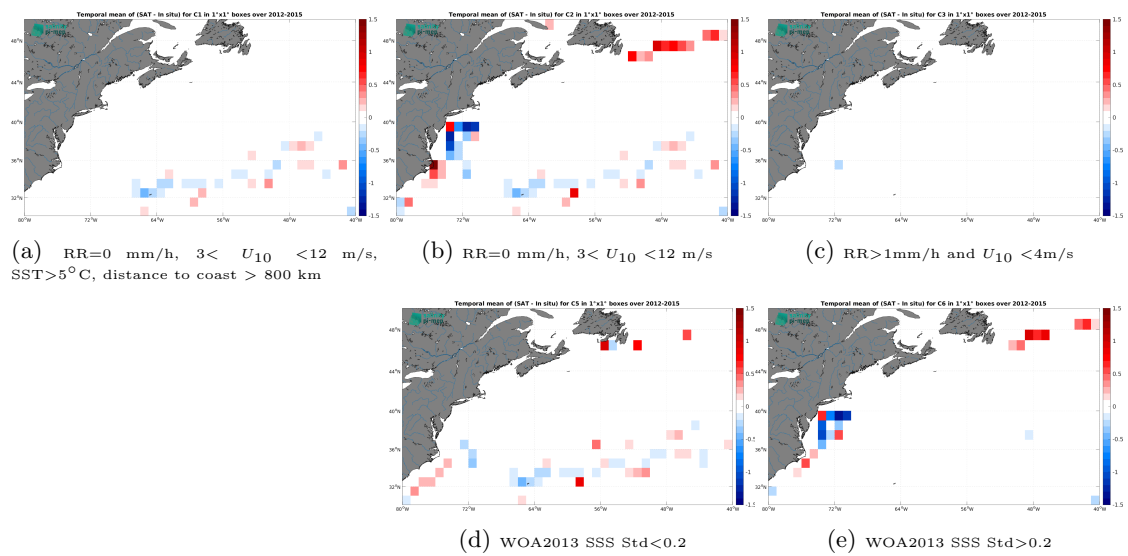
Figure 14: Temporal mean gridded over spatial boxes of size 1^\circ \times 1^\circ of \Delta SSS (Aquarius SSS L3 OR v5 - 7-Day running - Rain mask (NASA-GSFC) - TSG (GOSUD-Sailing-ship)) for 5 different subdatasets corresponding to:RR=0 mm/h, 3 < U_{10} < 12 m/s, SST >5^\circ C, distance to coast > 800 km (a), RR=0 mm/h, 3 < U_{10} < 12 m/s (b), RR >1 mm/h and U_{10} < 4 m/s (c), WOA2013 SSS Std <0.2 (d), WOA2013 SSS Std >0.2 (e).
