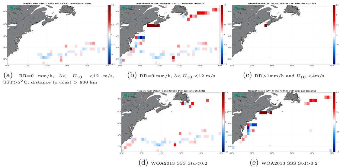
Figure 12: Temporal mean gridded over spatial boxes of size 1^{\circ}\times 1^{\circ} of \Delta SSS (Aquarius SSS L3 OR v5 - 7-Day running - Rain mask (NASA-GSFC) - TSG (GOSUD-Sailing-ship)) for 5 different subdatasets corresponding to:RR=0 mm/h, 3 < U_{10} < 12 m/s, SST >5^{\circ}\text{C} , distance to coast > 800 km (a), RR=0 mm/h, 3 < U_{10} < 12 m/s (b), RR >1 mm/h and U_{10} < 4 m/s (c), WOA2013 SSS Std <0.2 (d), WOA2013 SSS Std >0.2 (e).
