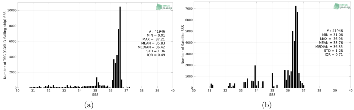
Figure 2: Histograms of SSS from TSG (GOSUD-Sailing-ship) (a) and Aquarius SSS L3 OR v5 - 7-Day running - Rain mask (NASA-GSFC) (b) considering all match-up pairs per bins of 0.1 over the Gulf Stream Pi-MEP region and for the full satellite product period.
