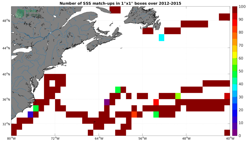
Figure 4: Number of SSS match-ups between TSG (GOSUD-Sailing-ship) SSS and the Aquarius SSS L3 OR v5 - 7-Day running - Rain mask (NASA-GSFC) SSS product for the Gulf Stream Pi-MEP region over 1^\circ \times 1^\circ boxes and for the full satellite product period.
