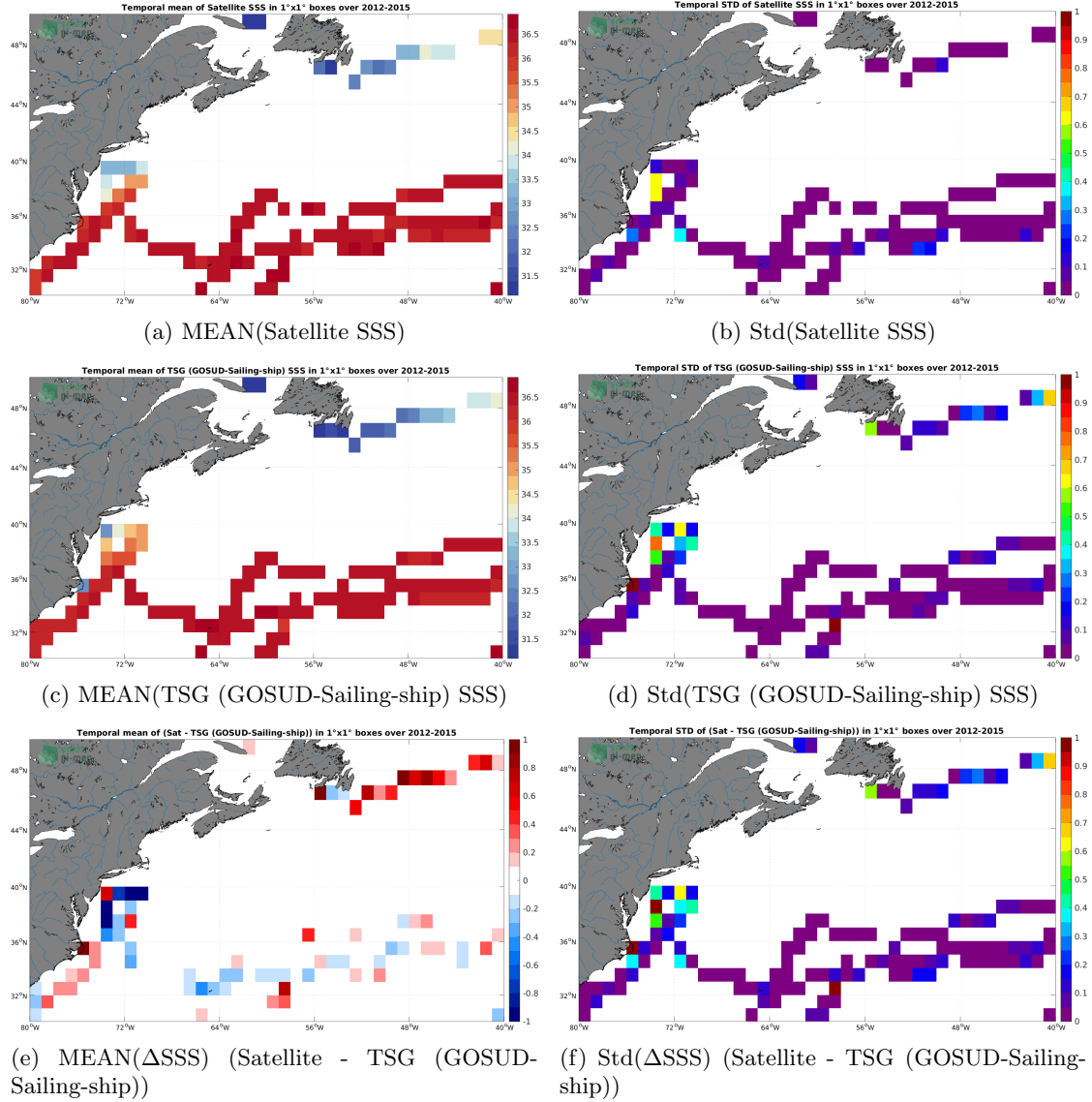
Figure 6: Temporal mean (left) and Std (right) of SSS from Aquarius SSS L3 OR v5 - 7-Day running - Rain mask (NASA-GSFC) (top), TSG (GOSUD-Sailing-ship) (middle), and of \Delta SSS (Satellite - TSG (GOSUD-Sailing-ship)). Only match-up pairs are used to generate these maps.
