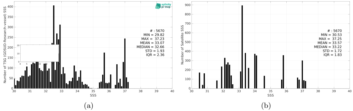
Figure 3: Histograms of SSS from TSG (GOSUD-Research-vessel) (a) and Aquarius SSS L3 OR v5 - 7-Day running - Rain mask (NASA-GSFC) (b) considering all match-up pairs per bins of 0.1 over the Gulf Stream Pi-MEP region and for the full satellite product period.
