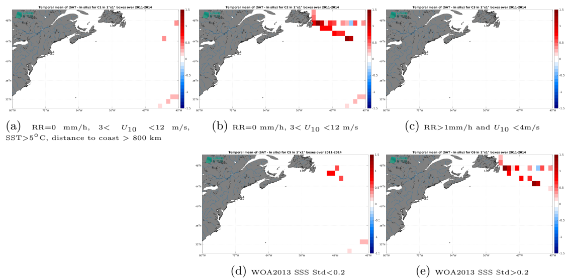
Figure 14: Temporal mean gridded over spatial boxes of size 1^\circ \times 1^\circ of \Delta SSS (Aquarius SSS L3 OR v5 - 7-Day running - Rain mask (NASA-GSFC) - TSG (GOSUD-Research-vessel)) for 5 different subdatasets corresponding to:RR=0 mm/h, 3 < U_{10} < 12 m/s, SST >5^\circ C, distance to coast > 800 km (a), RR=0 mm/h, 3 < U_{10} < 12 m/s (b), RR >1 mm/h and U_{10} < 4 m/s (c), WOA2013 SSS Std <0.2 (d), WOA2013 SSS Std >0.2 (e).
