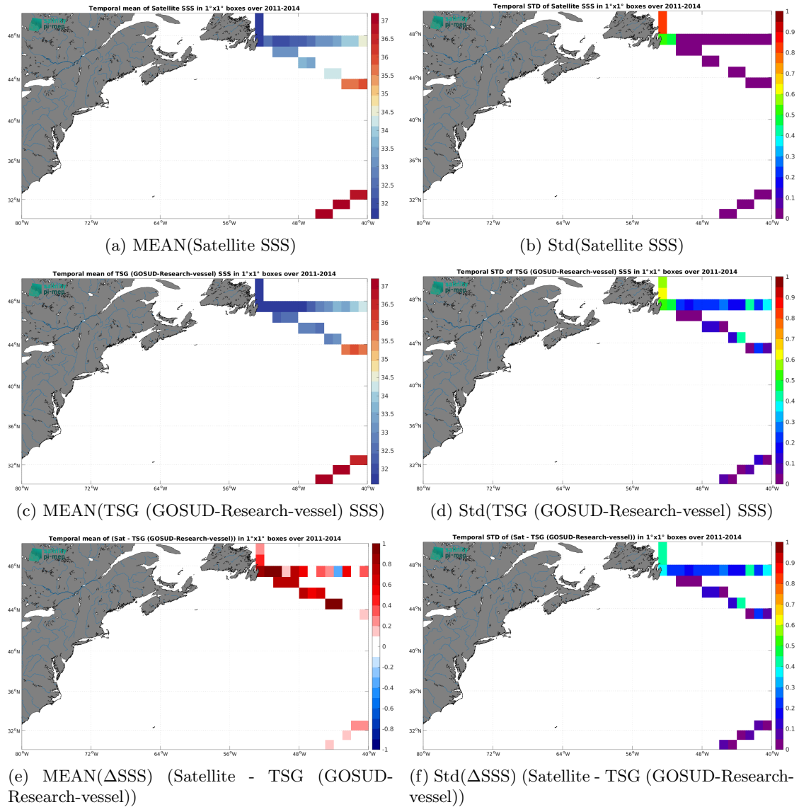
Figure 7: Temporal mean (left) and Std (right) of SSS from Aquarius SSS L3 OR v5 - 7-Day running - Rain mask (NASA-GSFC) (top), TSG (GOSUD-Research-vessel) (middle), and of \Delta SSS (Satellite - TSG (GOSUD-Research-vessel)). Only match-up pairs are used to generate these maps.
