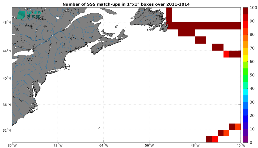
Figure 5: Number of SSS match-ups between TSG (GOSUD-Research-vessel) SSS and the Aquarius SSS L3 OR v5 - 7-Day running - Rain mask (NASA-GSFC) SSS product for the Gulf Stream Pi-MEP region over 1^\circ \times 1^\circ boxes and for the full satellite product period.
