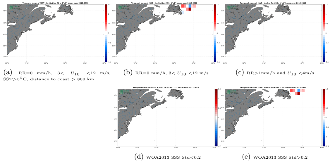
Figure 12: Temporal mean gridded over spatial boxes of size 1^{\circ}\times 1^{\circ} of \Delta\text{SSS} (Aquarius SSS L3 OR v5 - 7-Day running - Rain mask (NASA-GSFC) - TSG (CSIC-UTM)) for 5 different subdatasets corresponding to:RR=0 mm/h, 3 < U_{10} < 12 m/s, SST >5^{\circ}\text{C} , distance to coast > 800 km (a), RR=0 mm/h, 3 < U_{10} < 12 m/s (b), RR >1 mm/h and U_{10} < 4 m/s (c), WOA2013 SSS Std <0.2 (d), WOA2013 SSS Std >0.2 (e).
