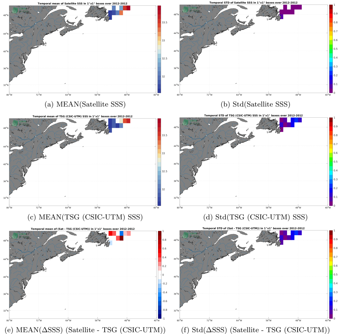
Figure 6: Temporal mean (left) and Std (right) of SSS from Aquarius SSS L3 OR v5 - 7-Day running - Rain mask (NASA-GSFC) (top), TSG (CSIC-UTM) (middle), and of \Delta SSS (Satellite - TSG (CSIC-UTM)). Only match-up pairs are used to generate these maps.
