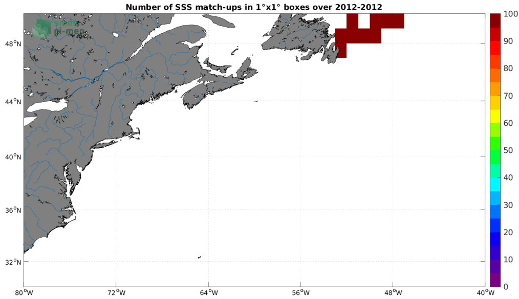
Figure 4: Number of SSS match-ups between TSG (CSIC-UTM) SSS and the Aquarius SSS L3 OR v5 - 7-Day running - Rain mask (NASA-GSFC) SSS product for the Gulf Stream Pi-MEP region over 1°×1° boxes and for the full satellite product period.
