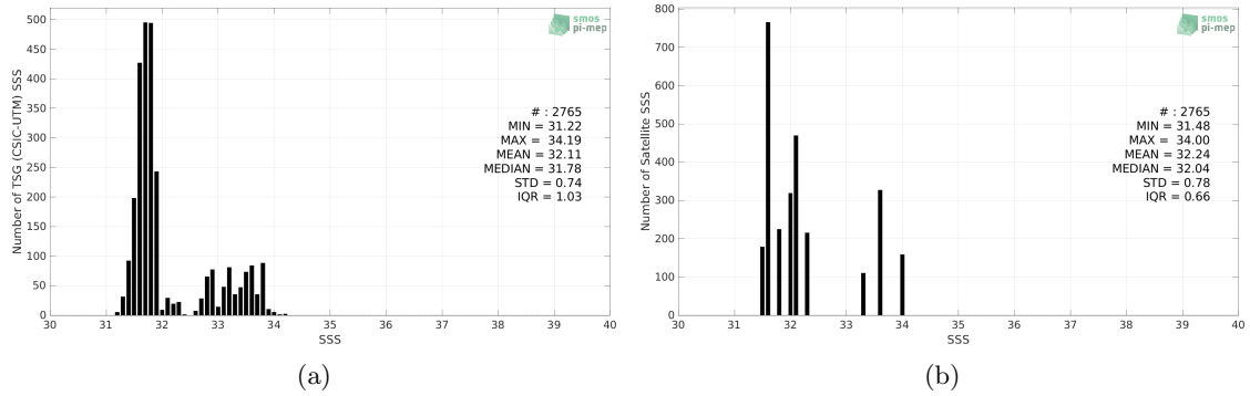
Figure 2: Histograms of SSS from TSG (CSIC-UTM) (a) and Aquarius SSS L3 OR v5 - 7-Day running - Rain mask (NASA-GSFC) (b) considering all match-up pairs per bins of 0.1 over the Gulf Stream Pi-MEP region and for the full satellite product period.
