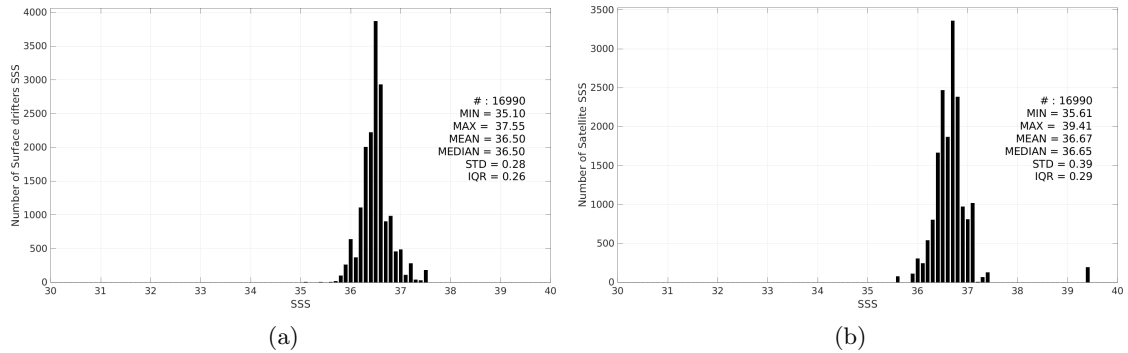
Figure 3: Histograms of SSS from Surface drifters (a) and Aquarius SSS L3 OR v5 - 7-Day running - Rain mask (NASA-GSFC) (b) considering all match-up pairs per bins of 0.1 over the Gulf Stream Pi-MEP region and for the full satellite product period.
