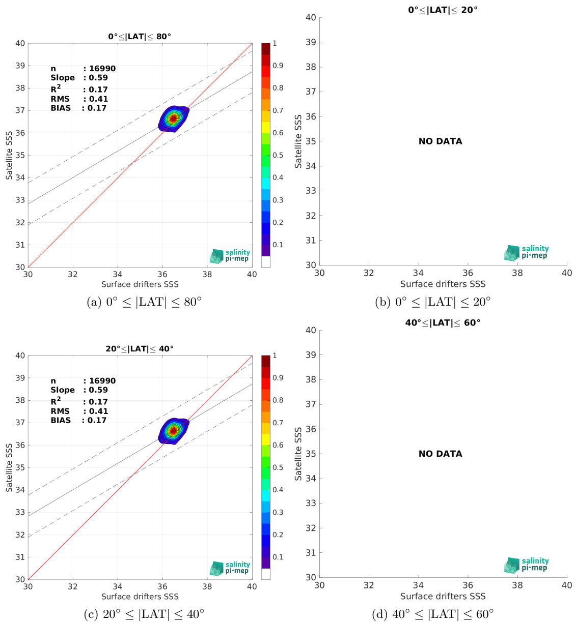
Figure 9: Contour maps of the concentration of Aquarius SSS L3 OR v5 - 7-Day running - Rain mask (NASA-GSFC) SSS (y-axis) versus Surface drifters SSS (x-axis) at match-up pairs for different latitude bands. For each plot, the red line shows x=y . The black thin and dashed lines indicate a linear fit through the data cloud and the \pm 95\% confidence levels, respectively. The number match-up pairs n , the slope and R^2 coefficient of the linear fit, the root mean square (RMS) and the mean bias between satellite and in situ data are indicated for each latitude band in each plots.
