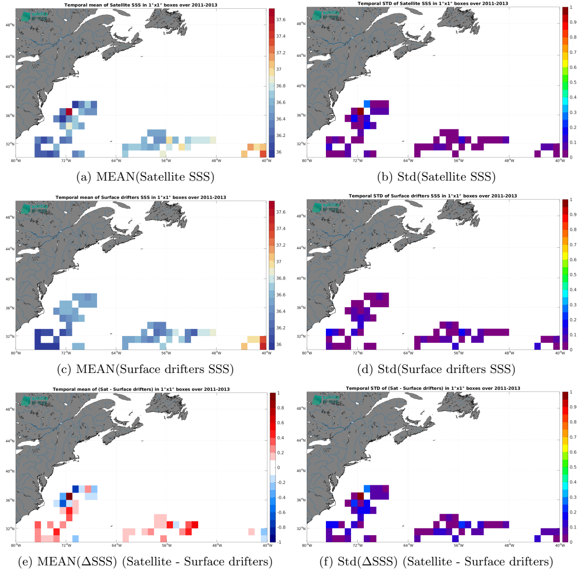
Figure 6: Temporal mean (left) and Std (right) of SSS from Aquarius SSS L3 OR v5 - 7-Day running - Rain mask (NASA-GSFC) (top), Surface drifters (middle), and of \Delta SSS (Satellite - Surface drifters). Only match-up pairs are used to generate these maps.
