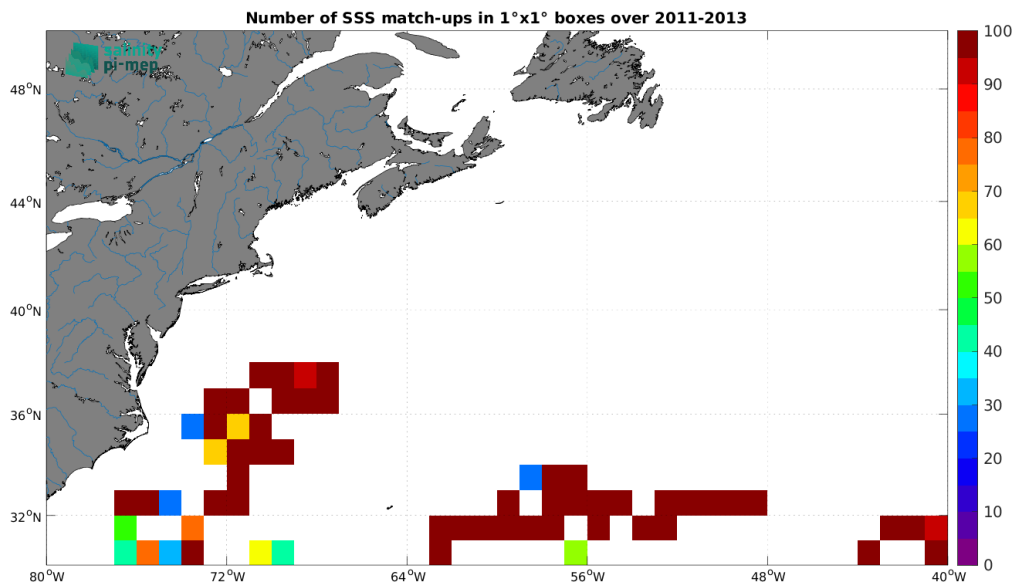
Figure 4: Number of SSS match-ups between Surface drifters SSS and the Aquarius SSS L3 OR v5 - 7-Day running - Rain mask (NASA-GSFC) SSS product for the Gulf Stream Pi-MEP region over 1^\circ \times 1^\circ boxes and for the full satellite product period.
