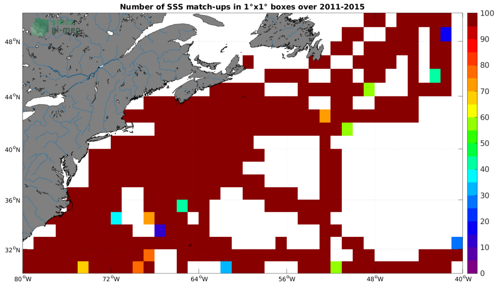
Figure 4: Number of SSS match-ups between TSG (SAMOS) SSS and the Aquarius SSS L3 OR v5 - Monthly (NASA-GSFC) SSS product for the Gulf Stream Pi-MEP region over 1^\circ \times 1^\circ boxes and for the full satellite product period.
