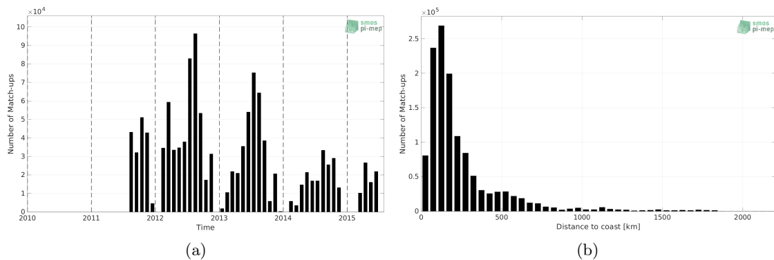
Figure 1: Number of match-ups between TSG (SAMOS) and Aquarius SSS L3 OR v5 - Monthly (NASA-GSFC) SSS as a function of time (a) and as function of the distance to coast (b) over the Gulf Stream Pi-MEP region and for the full satellite product period.
