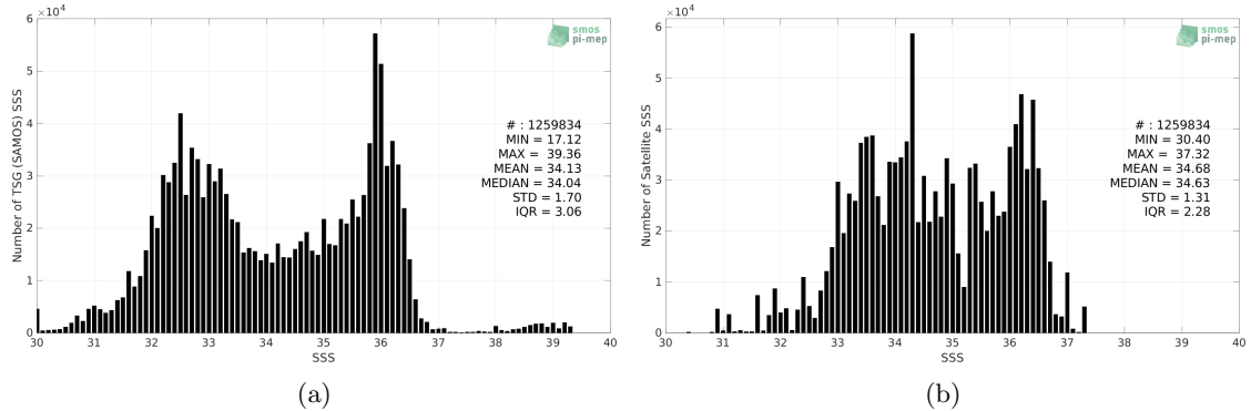
Figure 2: Histograms of SSS from TSG (SAMOS) (a) and Aquarius SSS L3 OR v5 - Monthly (NASA-GSFC) (b) considering all match-up pairs per bins of 0.1 over the Gulf Stream Pi-MEP region and for the full satellite product period.
