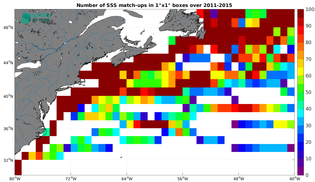
Figure 5: Number of SSS match-ups between TSG (LEGOS-DM) SSS and the Aquarius SSS L3 OR v5 - Monthly (NASA-GSFC) SSS product for the Gulf Stream Pi-MEP region over 1^\circ \times 1^\circ boxes and for the full satellite product period.
