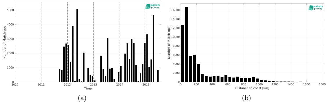
Figure 2: Number of match-ups between TSG (LEGOS-DM) and Aquarius SSS L3 OR v5 - Monthly (NASA-GSFC) SSS as a function of time (a) and as function of the distance to coast (b) over the Gulf Stream Pi-MEP region and for the full satellite product period.
