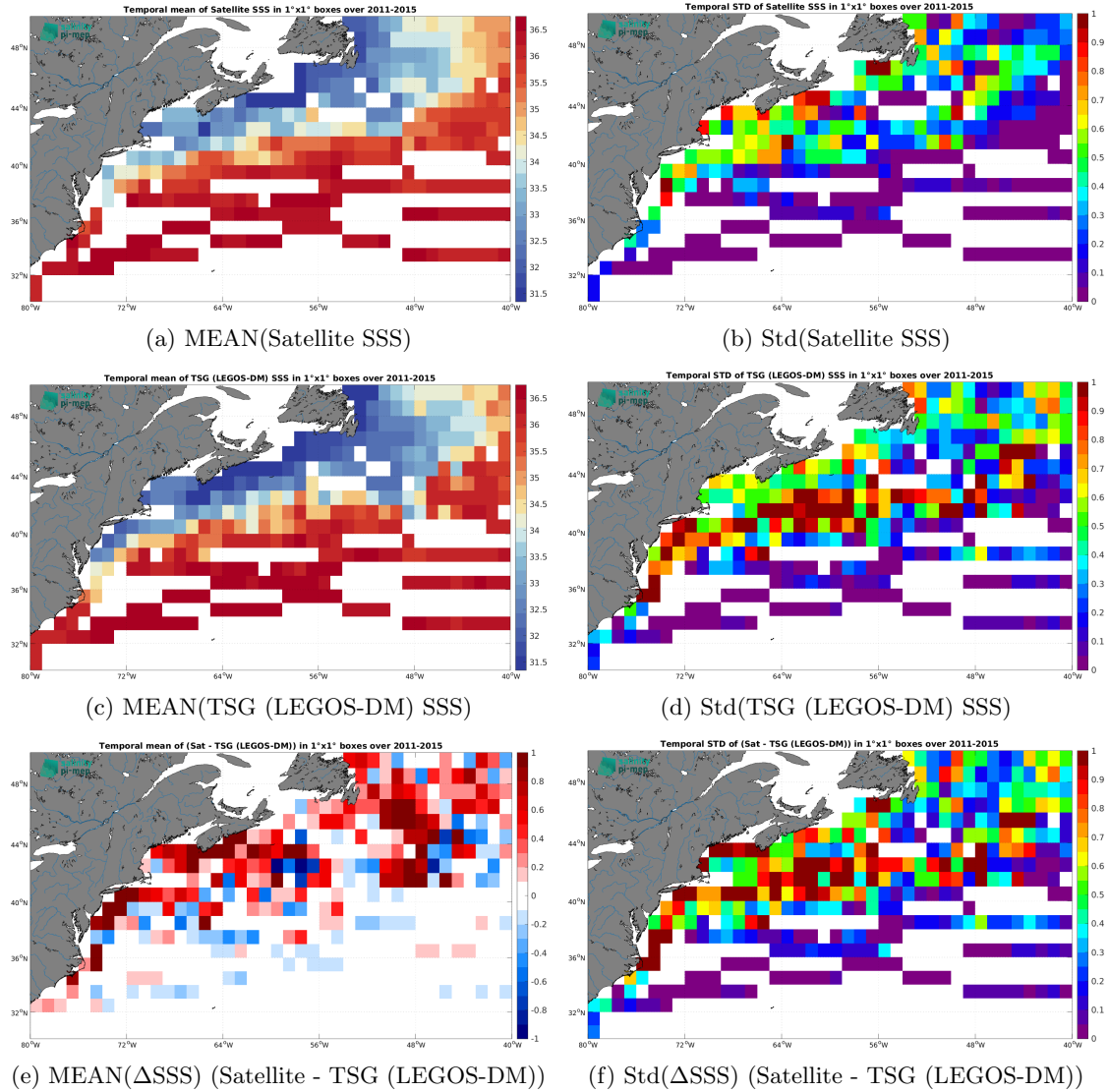
Figure 7: Temporal mean (left) and Std (right) of SSS from Aquarius SSS L3 OR v5 - Monthly (NASA-GSFC) (top), TSG (LEGOS-DM) ( in situ ) dataset (middle), and of \Delta SSS (Satellite - TSG (LEGOS-DM)). Only match-up pairs are used to generate these maps.
