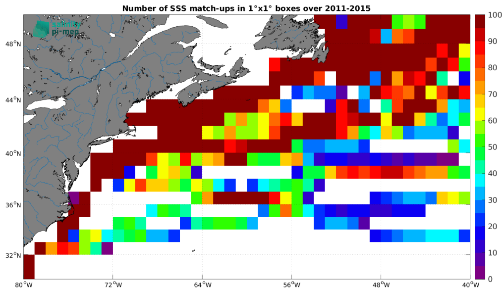
Figure 4: Number of SSS match-ups between TSG (LEGOS-DM) SSS and the Aquarius SSS L3 OR v5 - Monthly (NASA-GSFC) SSS product for the Gulf Stream Pi-MEP region over 1^\circ \times 1^\circ boxes and for the full satellite product period.
