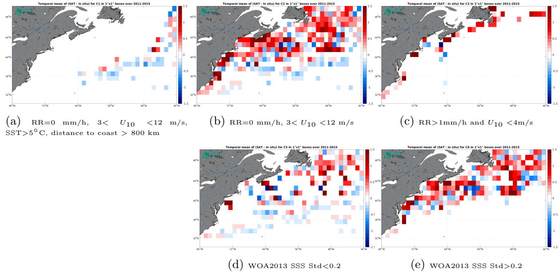
Figure 12: Temporal mean gridded over spatial boxes of size 1^{\circ}\times 1^{\circ} of \Delta\text{SSS} (Aquarius SSS L3 OR v5 - Monthly (NASA-GSFC) - TSG (LEGOS-DM)) for 5 different subdatasets corresponding to:RR=0 mm/h, 3 < U_{10} < 12 m/s, SST >5^{\circ}\text{C} , distance to coast > 800 km (a), RR=0 mm/h, 3 < U_{10} < 12 m/s (b), RR >1 mm/h and U_{10} < 4 m/s (c), WOA2013 SSS Std <0.2 (d), WOA2013 SSS Std >0.2 (e).
