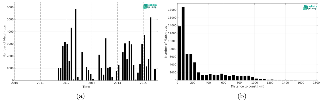
Figure 1: Number of match-ups between TSG (LEGOS-DM) and Aquarius SSS L3 OR v5 - Monthly (NASA-GSFC) SSS as a function of time (a) and as function of the distance to coast (b) over the Gulf Stream Pi-MEP region and for the full satellite product period.
