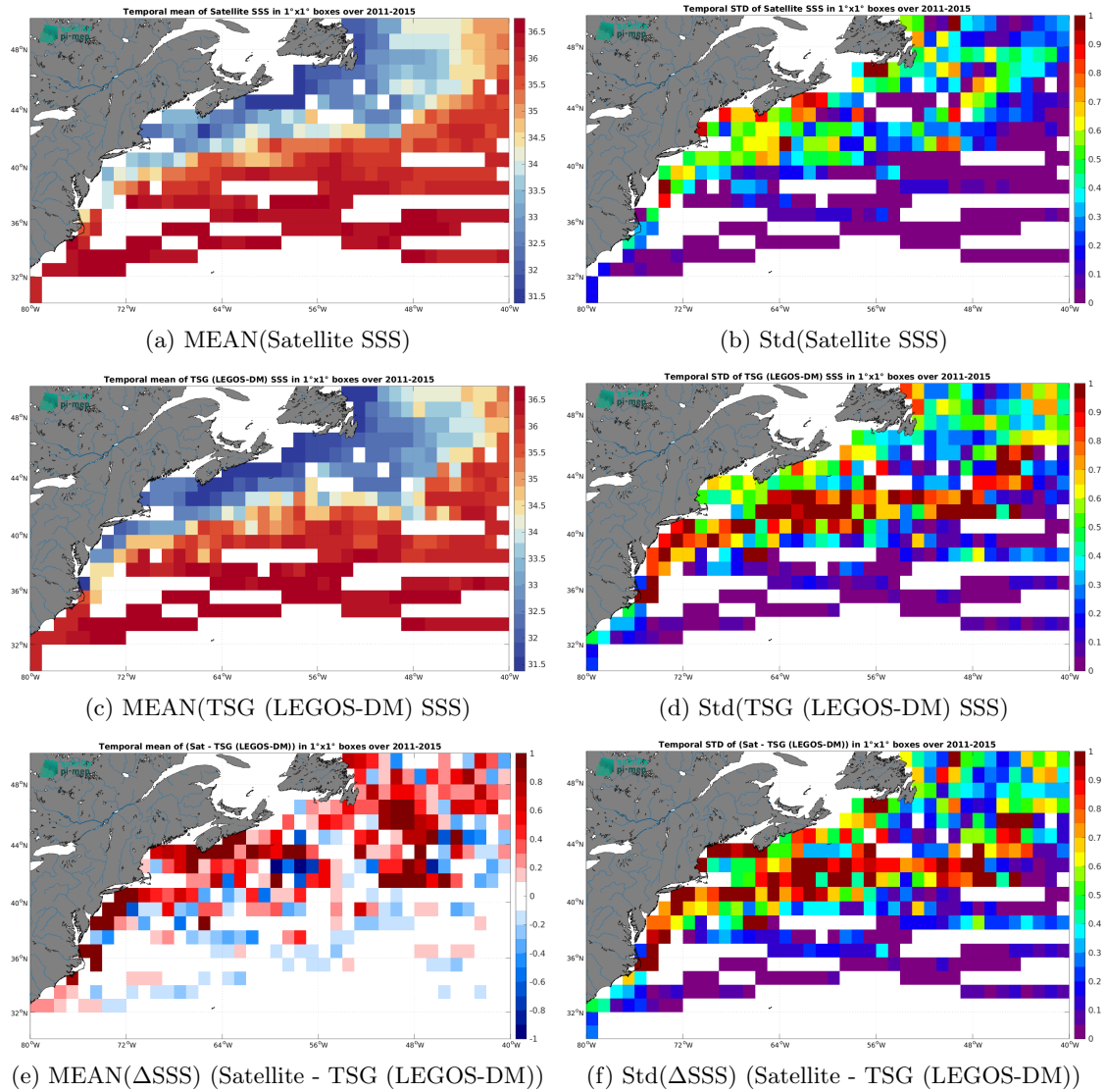
Figure 6: Temporal mean (left) and Std (right) of SSS from Aquarius SSS L3 OR v5 - Monthly (NASA-GSFC) (top), TSG (LEGOS-DM) ( in situ ) dataset (middle), and of \Delta SSS (Satellite - TSG (LEGOS-DM)). Only match-up pairs are used to generate these maps.
