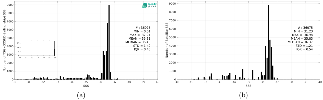
Figure 3: Histograms of SSS from TSG (GOSUD-Sailing-ship) (a) and Aquarius SSS L3 OR v5 - Monthly (NASA-GSFC) (b) considering all match-up pairs per bins of 0.1 over the Gulf Stream Pi-MEP region and for the full satellite product period.
