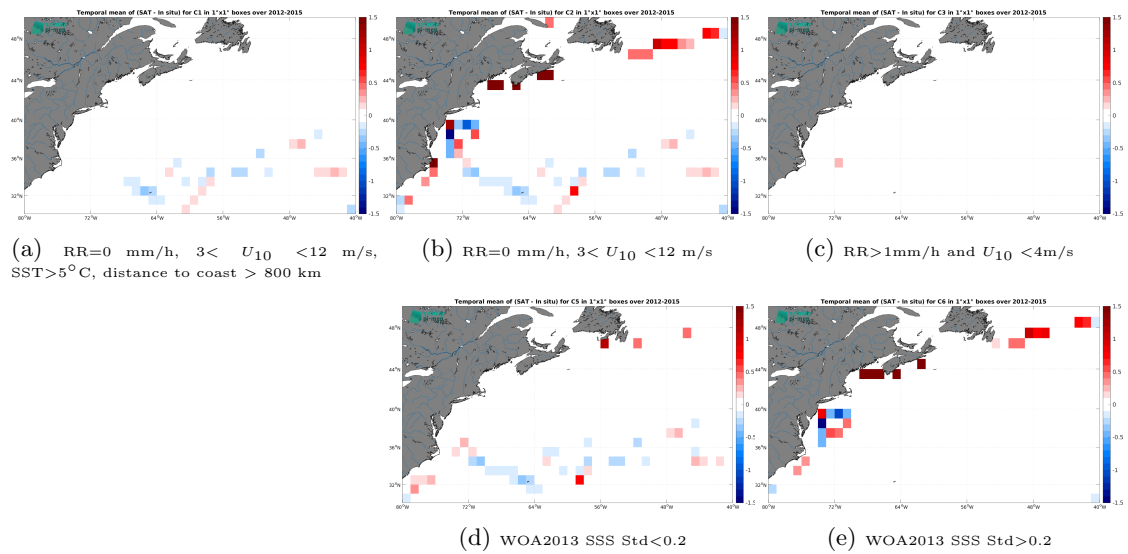
Figure 14: Temporal mean gridded over spatial boxes of size 1^\circ \times 1^\circ of \Delta SSS (Aquarius SSS L3 OR v5 - Monthly (NASA-GSFC) - TSG (GOSUD-Sailing-ship)) for 5 different subdatasets corresponding to: RR=0 mm/h, 3 < U_{10} < 12 m/s, SST > 5°C, distance to coast > 800 km (a), RR=0 mm/h, 3 < U_{10} < 12 m/s (b), RR > 1mm/h and U_{10} < 4 m/s (c), WOA2013 SSS Std < 0.2 (d), WOA2013 SSS Std > 0.2 (e).
