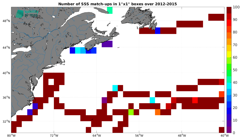
Figure 5: Number of SSS match-ups between TSG (GOSUD-Sailing-ship) SSS and the Aquarius SSS L3 OR v5 - Monthly (NASA-GSFC) SSS product for the Gulf Stream Pi-MEP region over 1^\circ \times 1^\circ boxes and for the full satellite product period.
