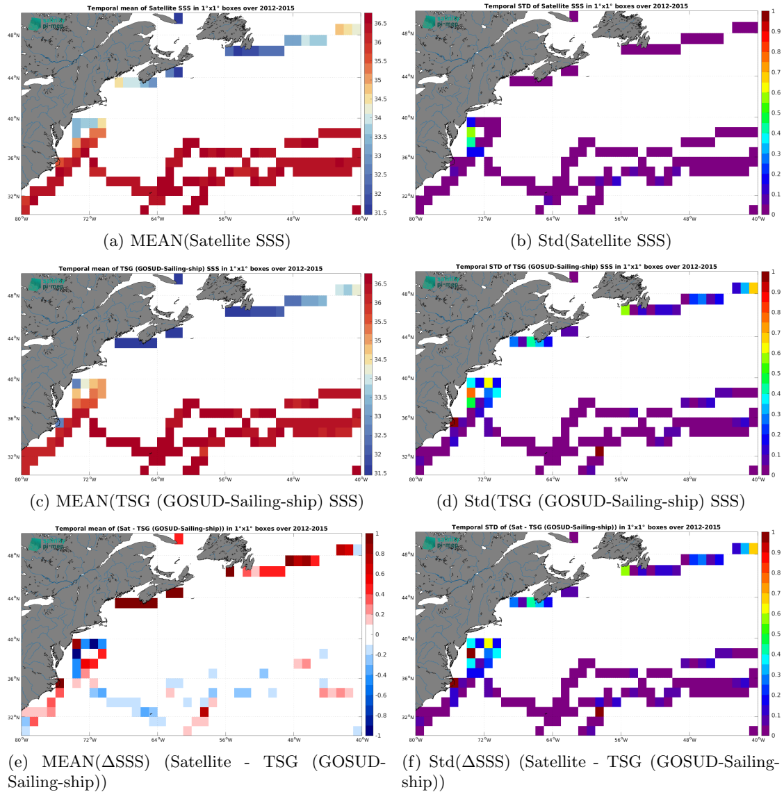
Figure 7: Temporal mean (left) and Std (right) of SSS from Aquarius SSS L3 OR v5 - Monthly (NASA-GSFC) (top), TSG (GOSUD-Sailing-ship) (middle), and of \Delta SSS (Satellite - TSG (GOSUD-Sailing-ship)). Only match-up pairs are used to generate these maps.
