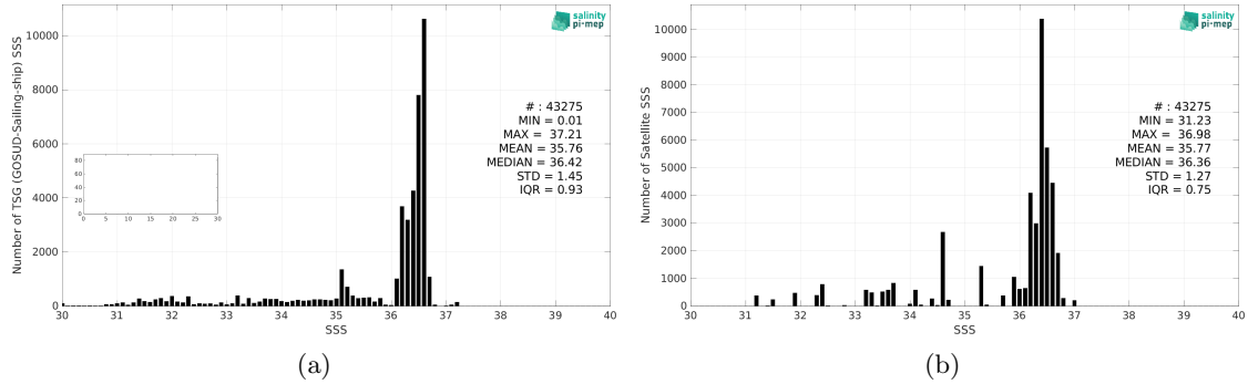
Figure 2: Histograms of SSS from TSG (GOSUD-Sailing-ship) (a) and Aquarius SSS L3 OR v5 - Monthly (NASA-GSFC) (b) considering all match-up pairs per bins of 0.1 over the Gulf Stream Pi-MEP region and for the full satellite product period.
