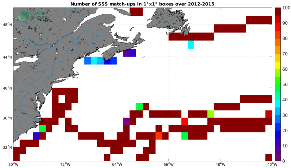
Figure 4: Number of SSS match-ups between TSG (GOSUD-Sailing-ship) SSS and the Aquarius SSS L3 OR v5 - Monthly (NASA-GSFC) SSS product for the Gulf Stream Pi-MEP region over 1^\circ \times 1^\circ boxes and for the full satellite product period.
