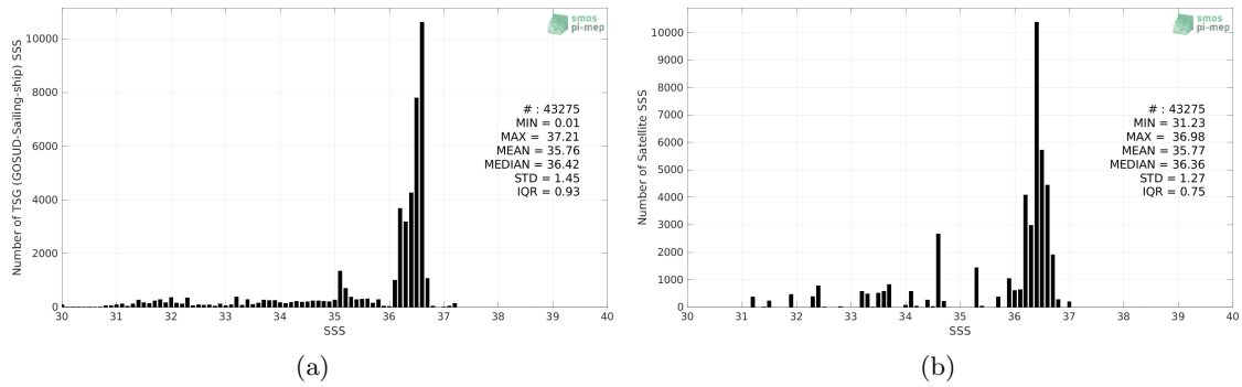
Figure 2: Histograms of SSS from TSG (GOSUD-Sailing-ship) (a) and Aquarius SSS L3 OR v5 - Monthly (NASA-GSFC) (b) considering all match-up pairs per bins of 0.1 over the Gulf Stream Pi-MEP region and for the full satellite product period.
