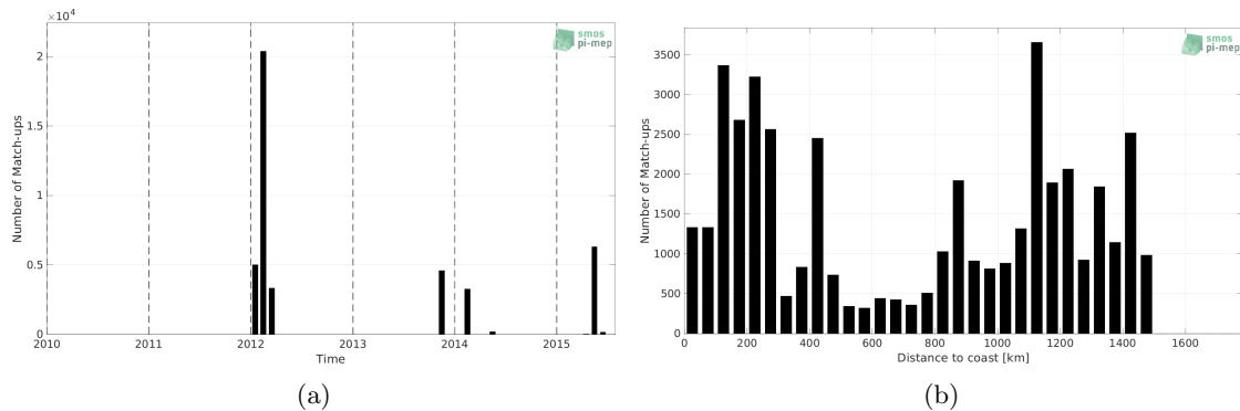
Figure 1: Number of match-ups between TSG (GOSUD-Sailing-ship) and Aquarius SSS L3 OR v5 - Monthly (NASA-GSFC) SSS as a function of time (a) and as function of the distance to coast (b) over the Gulf Stream Pi-MEP region and for the full satellite product period.
