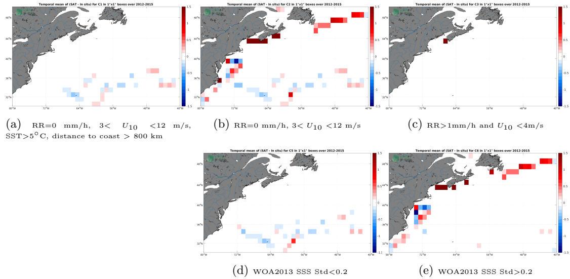
Figure 12: Temporal mean gridded over spatial boxes of size 1^{\circ}\times 1^{\circ} of \Delta SSS (Aquarius SSS L3 OR v5 - Monthly (NASA-GSFC) - TSG (GOSUD-Sailing-ship)) for 5 different subdatasets corresponding to:RR=0 mm/h, 3 < U_{10} < 12 m/s, SST > 5^{\circ}\text{C} , distance to coast > 800 km (a), RR=0 mm/h, 3 < U_{10} < 12 m/s (b), RR > 1 mm/h and U_{10} < 4 m/s (c), WOA2013 SSS Std < 0.2 (d), WOA2013 SSS Std > 0.2 (e).
